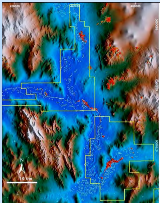
Digital Terrain Model (Topographic) Image
