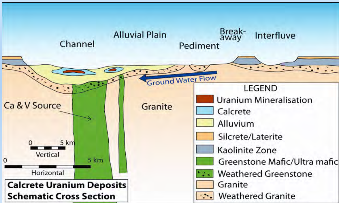
Model for Calcrete Hosted Uranium deposits
