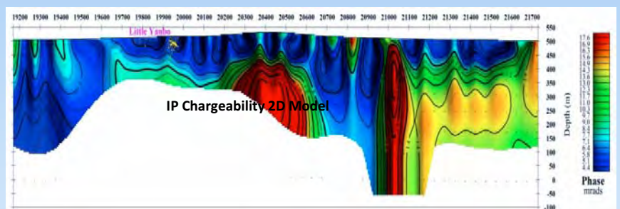
IP Chargeability 2D Model
