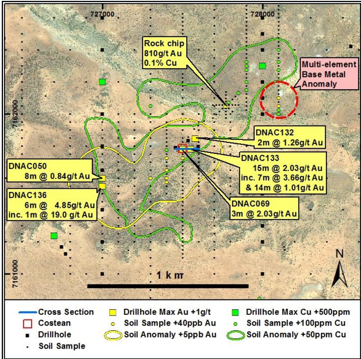
Figure 3: Vulcan Soil Au and Cu Anomalies, and Rock Chip Location
