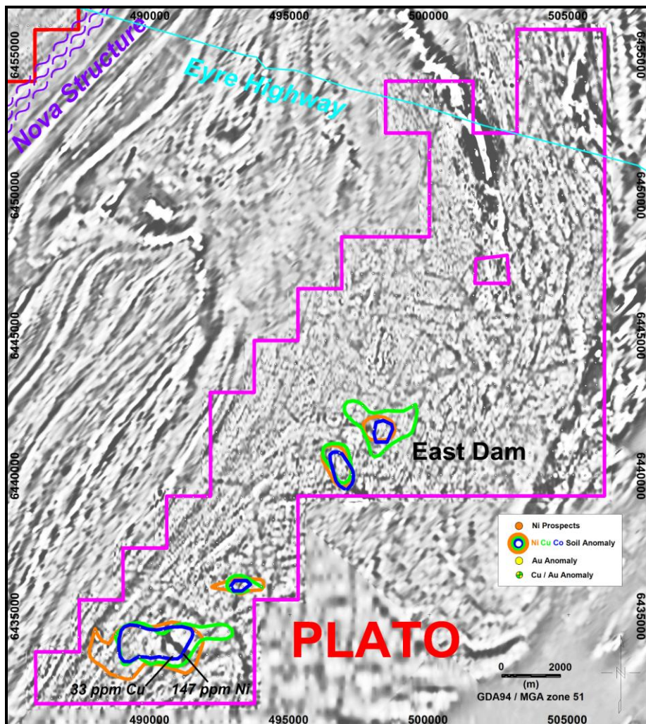
Figure 2: Fraser Range, Detail: Plato Nickel Prospect over Magnetic Image
