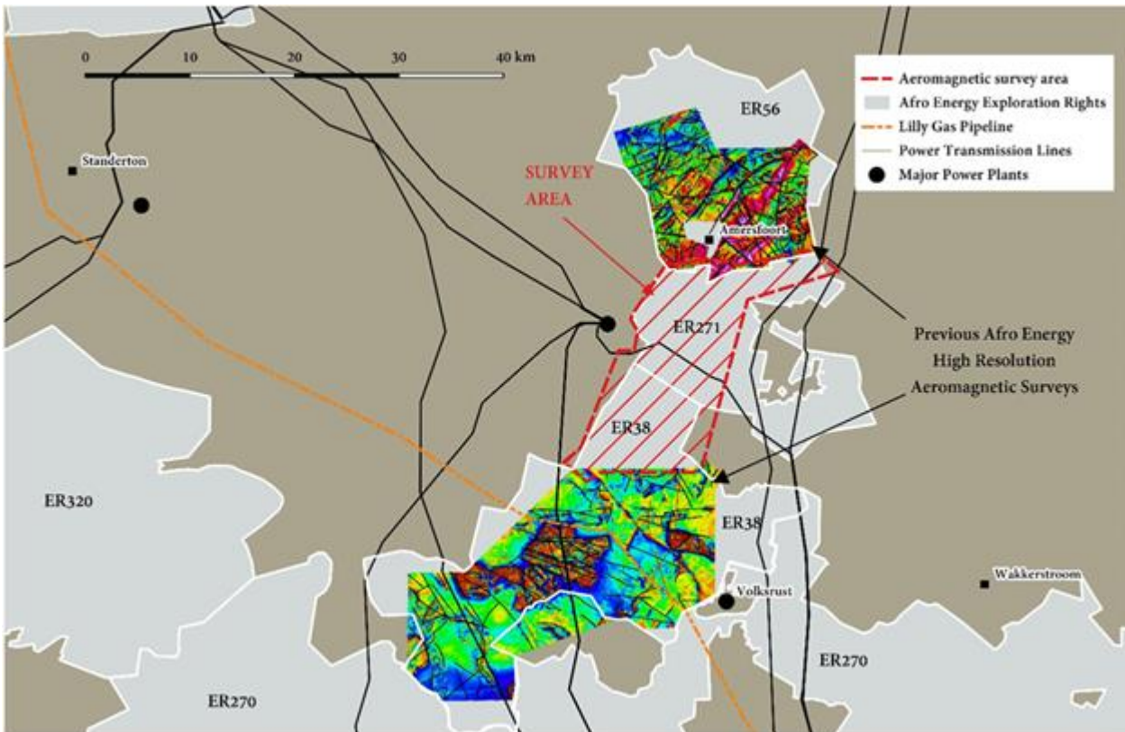
Figure 1 Amersfoort Project exploration licences and 2020 aeromagnetic survey areas.
