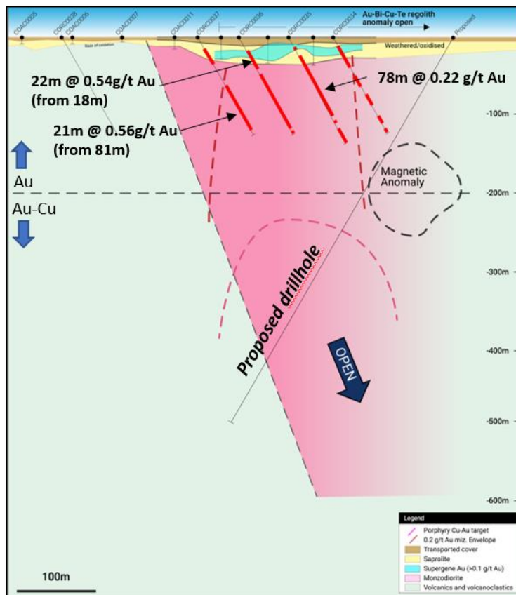
Figure 3: Lady Ilse Prospect schematic cross section (6408300N) showing wide zone of gold anomalism at 100m depth, akin to the equivalent stage of drilling/exploration at the nearby Boda Discovery (ALK ASX 15 August 2017)
