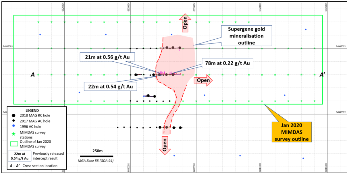
Figure 2: Lady Ilse Prospect, showing MIMDAS survey area with main drilling results (see ASX MAG 19 February 2018)
