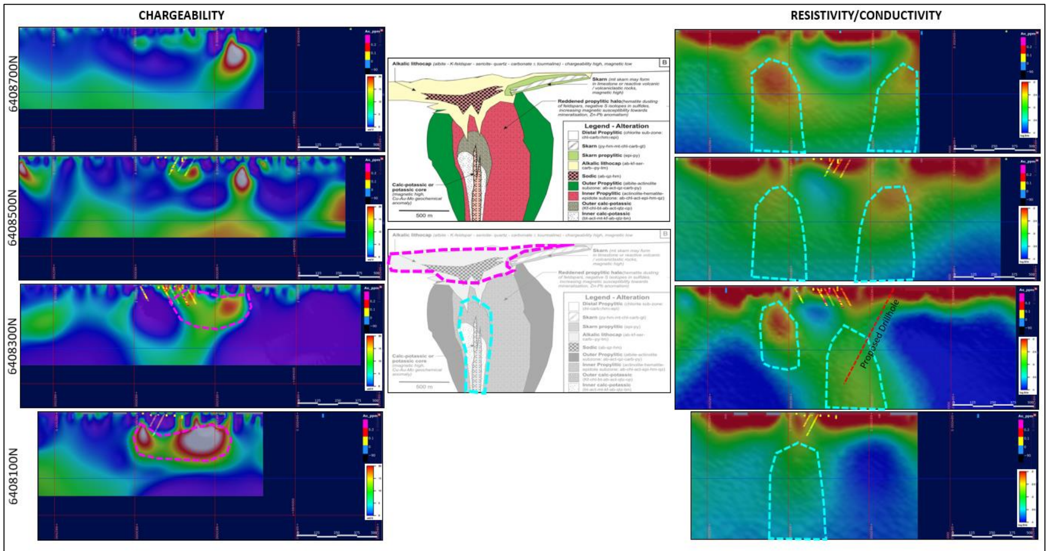
Figure 1: Lady Ilse MIMDAS Chargeability and Resistivity/Conductivity Inversions, Lines 6408100N - 6408700N, looking north, showing a strongly chargeable feature downdip from zone of gold + porphyry pathfinder anomalism in drilling and overlying a conductive porphyry target. The significance of the conductive feature downdip from a strongly chargeable zone is unconfirmed at Cadia, however high conductivity contrasts for Cadia porphyry mineralisation is described by Close et al (2001) with the usefulness of advanced DC resistivity and magnetotelluric (MT) resistivity systems (such as MIMDAS) for detecting porphyry systems also highlighted by Holliday and Cooke (2007)
