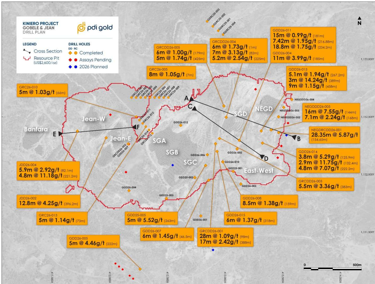
Figure 2: Gobeles and Jean drill plan
