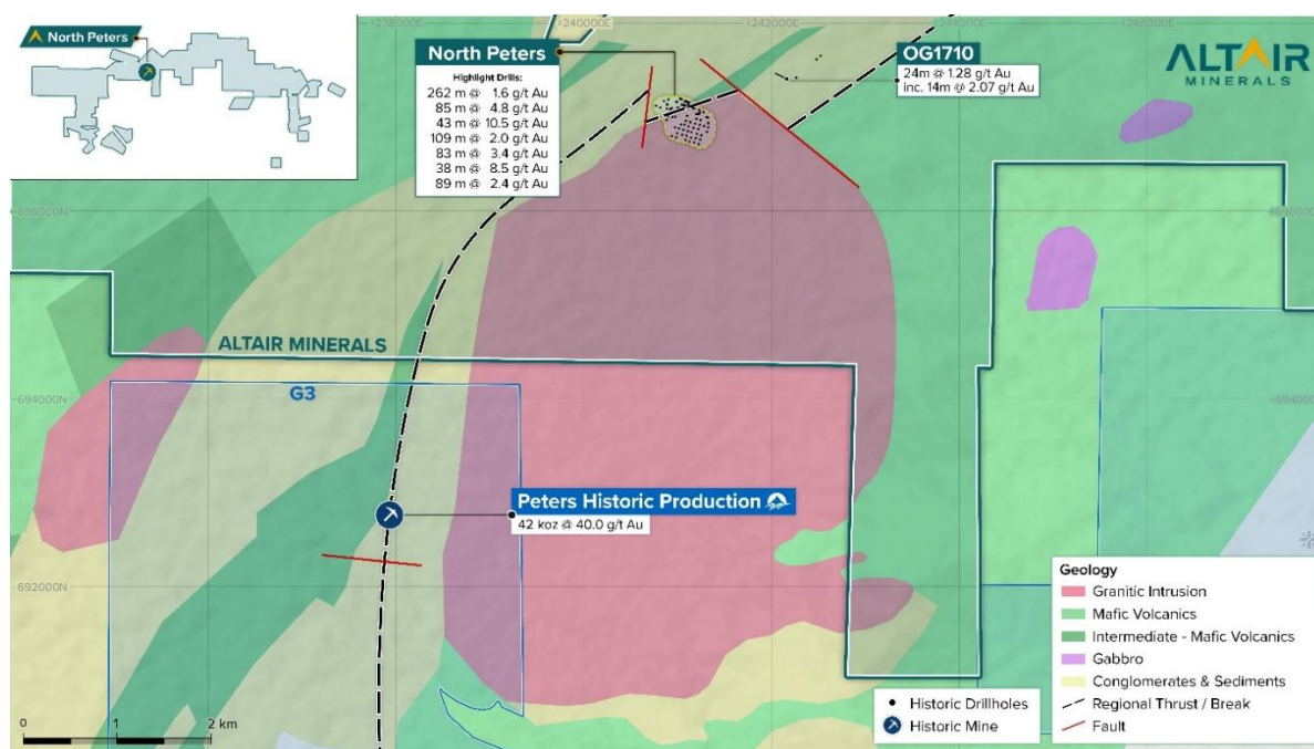
Figure 5: Geological map of Puruni District with NP historic drilling. WGS84 UTM Zone 21N. 19,20,26,34
