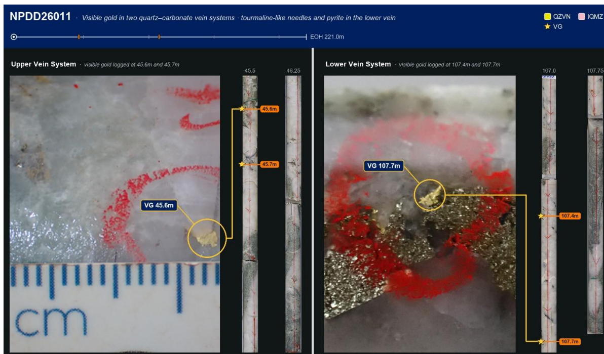
Figure 6: Visible gold in NPDD26011. A – stylolitic quartz–carbonate vein within broader veining system, with visible gold at 45.6m (close-up with centimetre scale). B – visible gold at 107.7m within a quartz–carbonate vein carrying tourmaline-like needles and pyrite. Visual observations only; see Cautionary Statement 42 .
