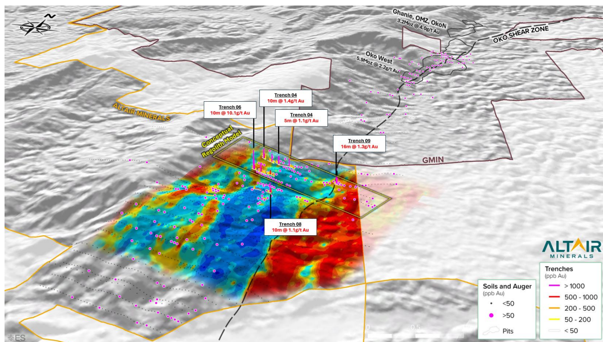
Figure 3: Perspective 3D view at SOKO of ground gradient array IP chargeability survey, soil and auger geochemistry and selected trenching results at SOKO. Note: 3D perspective view skews axis and scale moving from image centre. 1,3,23,33,34,38,43
