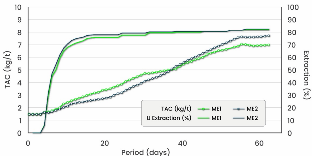
Figure 4: Column leach uranium dissolution and total acid consumption over time
