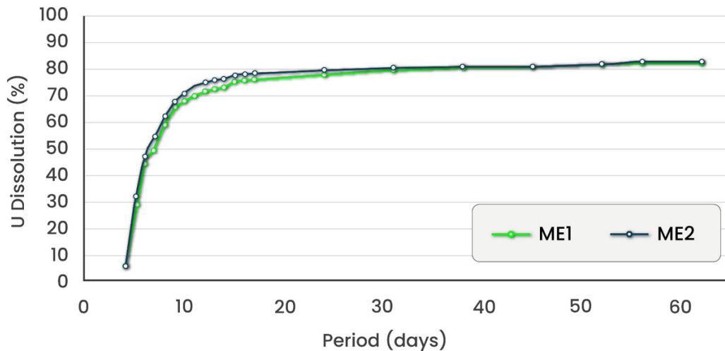
Figure 3: Bottle Roll leach uranium dissolution over time
