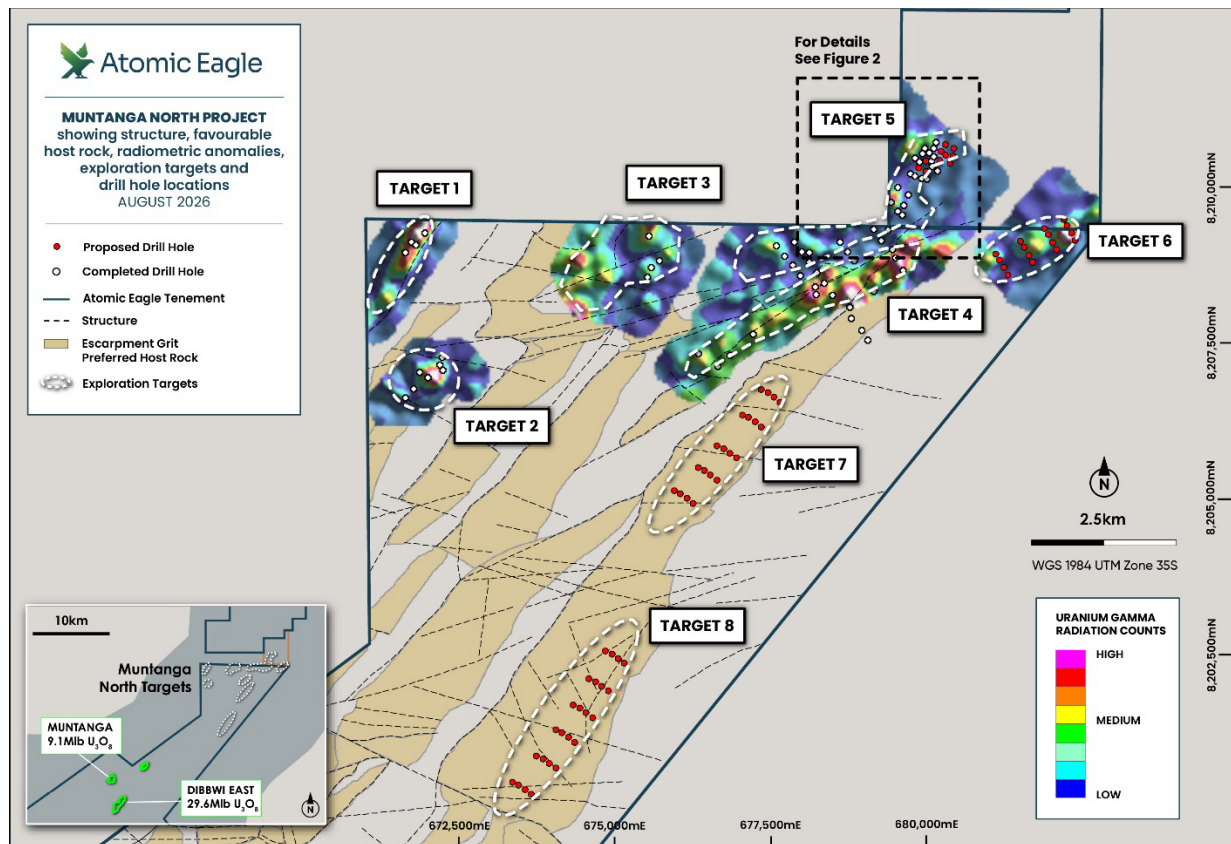
Figure 1: Muntanga North proposed drilling
