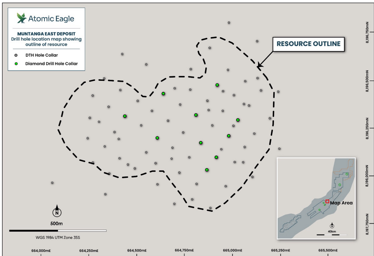
Figure 2: Muntanga East resource outline showing locations of diamond drill holes used to generate the composite samples
