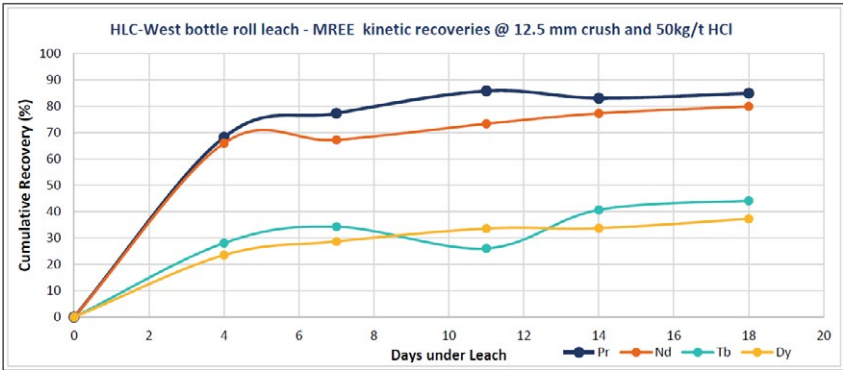
Figure 2.10: HLC - West bottle roll leach results – cumulative recovery by day
