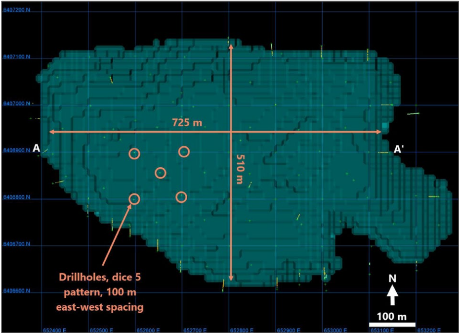
Figure 2.2: Plan view of Toongi deposit – Dubbo Project
