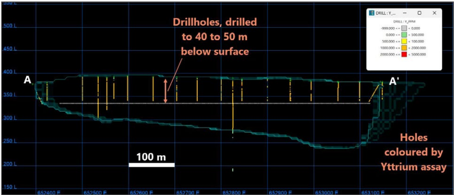
Figure 2.3: Section view of Toongi deposit – Dubbo Project
