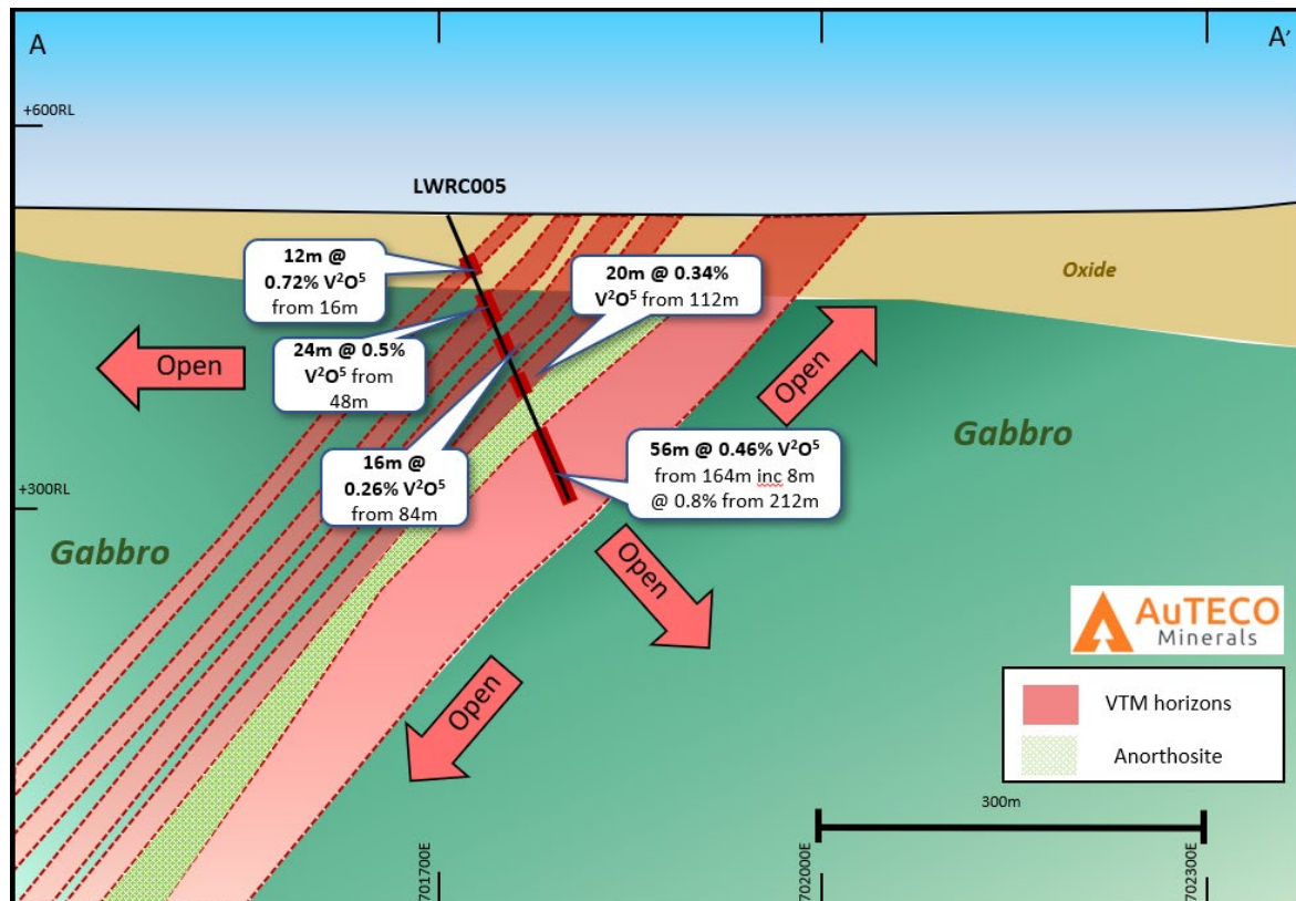
Figure 2: Interpreted Cross-section showing the recent drill hole LWRC005 with significant vanadium-titanium mineralisation intercepted over broad widths including to the end of hole. The hole assayed 56m @ 0.46 % V 2 O 5 and 6.1% TiO 2 from 164m to EOH.
