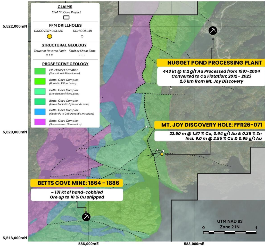
Figure 4. Mount Joy discovery location and regional geology, showing the Nugget Pond processing facility and the prospective volcanic sequence within the Tilt Cove-Betts Cove district.
