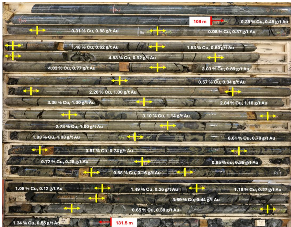
Figure 2: Mount Joy discovery hole FFR26-071 with high-grade copper and gold mineralisation of 22.5m @ 2.5% CuEq including 9.0m @ 3.9% CuEq (3.0% Cu and 1.0g/t Au). Core photograph showing mineralisation in the upper VMS and transitioning into the lower stringer zone. These mineralisation styles are similar to those observed at the Ming Mine (with a current MRE of 57.4Mt @ 2.4% CuEq M&I plus 17.3Mt @ 2.8% CuEq Inferred).
