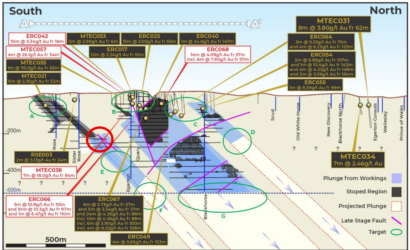
Figure 1: Mt Egerton mining complex long-section showing drill target areas – the red circle indicates the area to be drilled by the next few holes.
