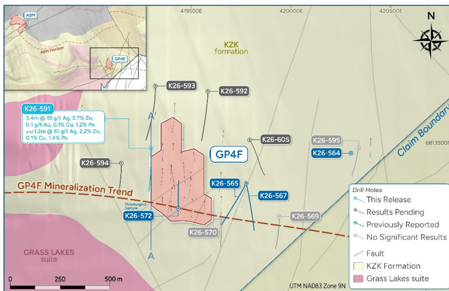
Figure 5: Plan view of GP4F prospect and 2026 drilling.
