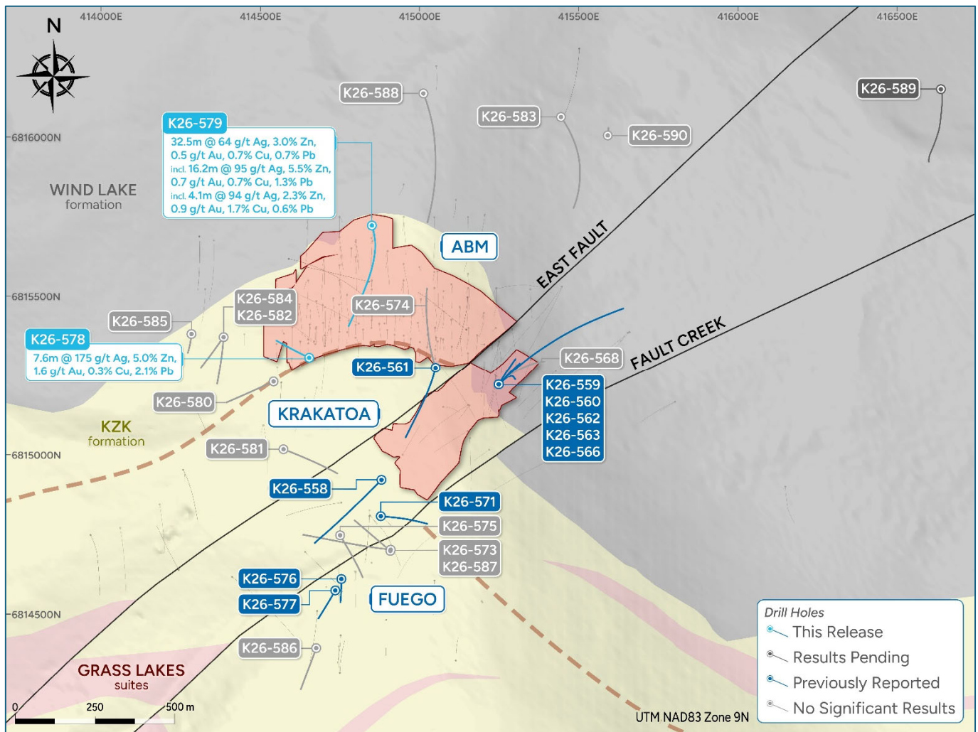
Figure 7: Recent drilling in the ABM area
