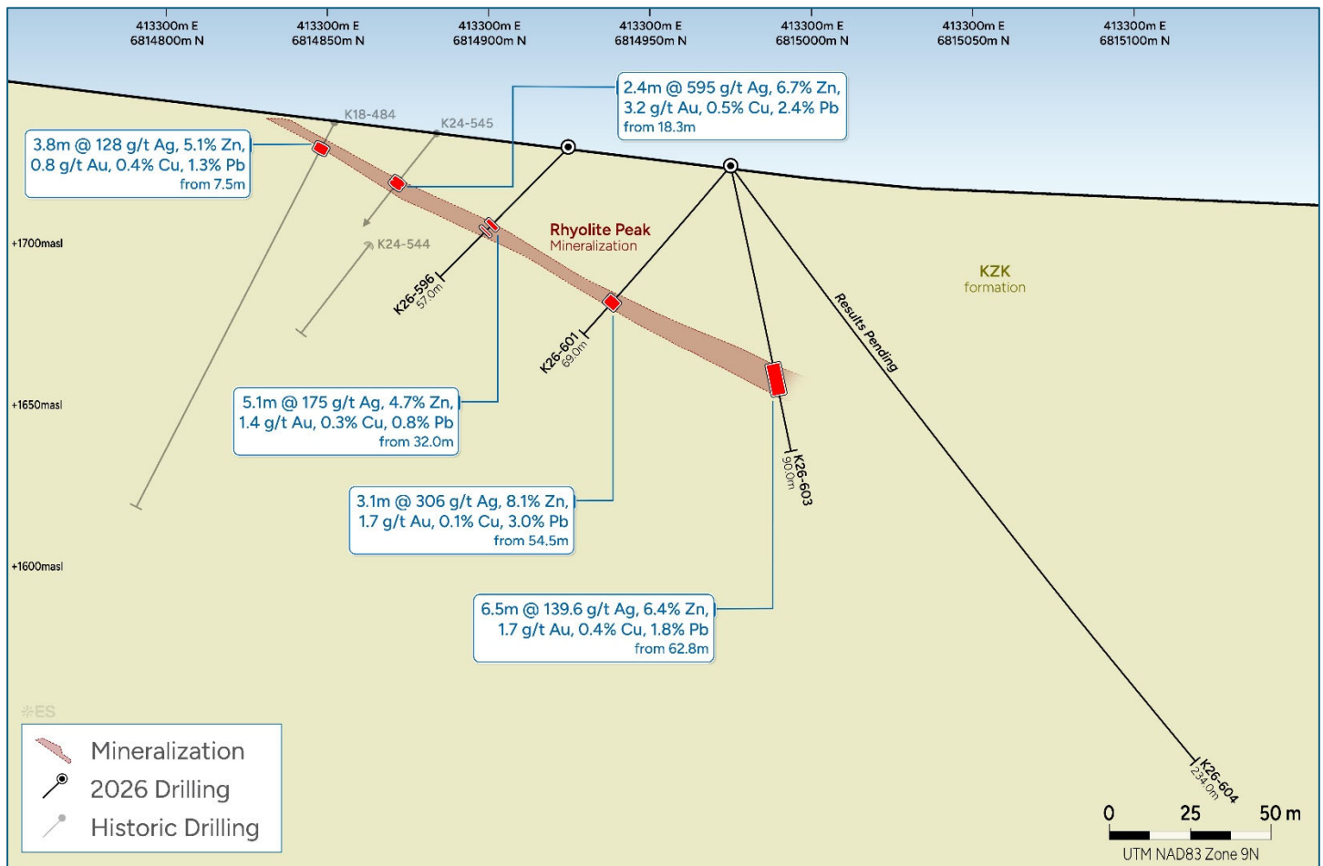
Figure 4: Section 413300mE looking west showing typical thickness and extent of Rhyolite Peak mineralization.
