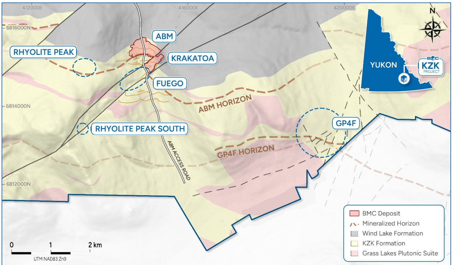
Figure 2: Location map of BMC's key target areas at the KZK property
