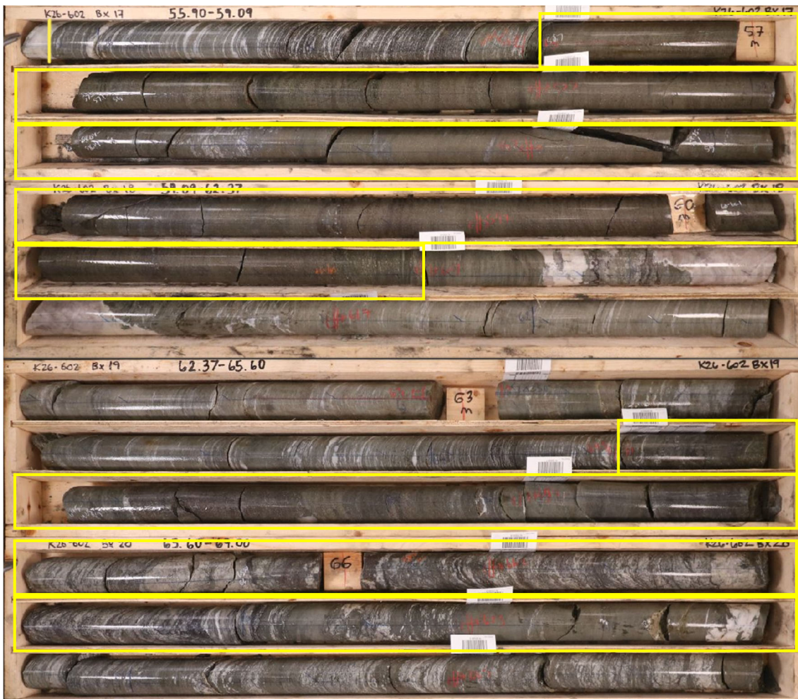
Photo 8: Hole K26-602 (Rhyolite Peak) highlighted interval of 4.0m (2.6m true width) @ 264g/t Ag, 9.0% Zn, 2.9g/t Au, 0.6% Cu, 4.3% Pb from 56.7m and 3.0m (1.9m true width) @ 37g/t Ag, 5.4% Zn, 0.4g/t Au, 0.3% Cu, 1.3% Pb from 64.3m
