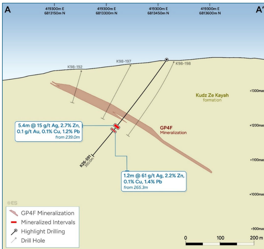
Figure 6: Cross section view of GP4F prospect (looking west) with K26-591 projected to adjacent drill section.
