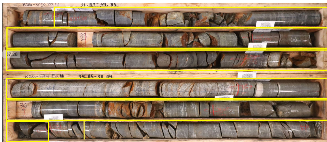
Photo 3: Hole K26-596 (Rhyolite Peak) Highlighted interval of 5.1m (5.0m true width) @175g/t Ag, 4.7% Zn, 1.4g/t Au, 0.3% Cu, 0.8% Pb from 32.0m including: 3.6m (3.5m true width) @ 237g/t Ag, 6.4% Zn, 1.9g/t Au, 0.4% Cu, 1.0% Pb from 33.5m
