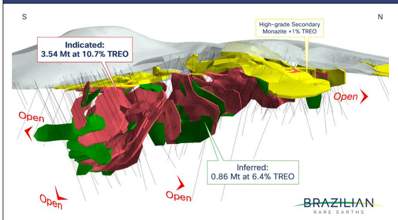
FIGURE 1: 3D VIEW OF UPDATED MONTE ALTO MINERAL RESOURCE
