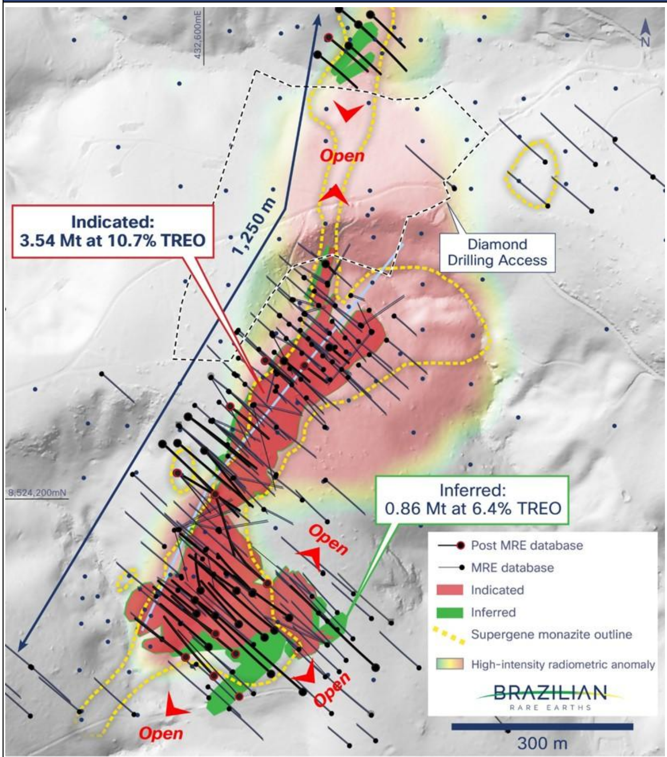
FIGURE 2: MONTE ALTO PLAN VIEW OF UPDATED MINERAL RESOURCE EXTENT AND DRILLING
