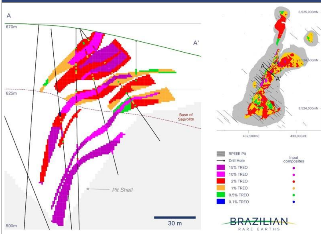
FIGURE 5: CROSS-SECTION VIEW OF MONTE ALTO BLOCK MODEL
