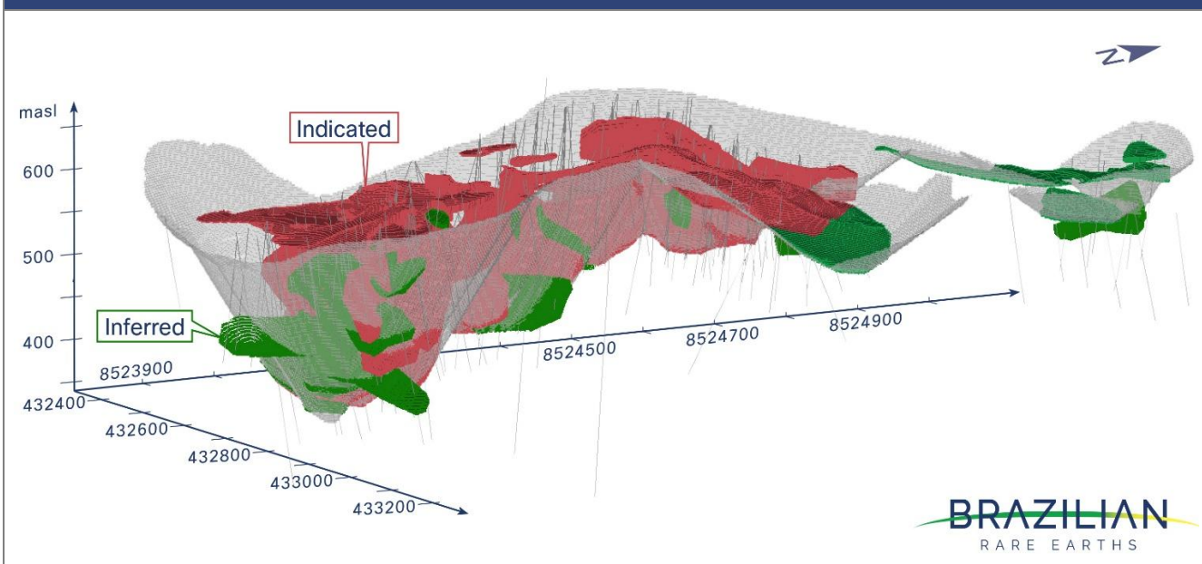
FIGURE 12: 3D VIEW OF BLOCK MODEL COLORED BY TREO GRADE WITH PIT SHELL
