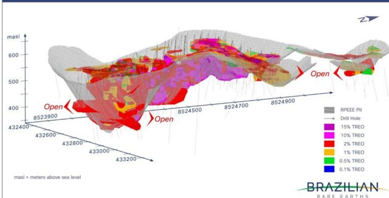
FIGURE 4: 3D VIEW OF MONTE ALTO BLOCK MODEL
