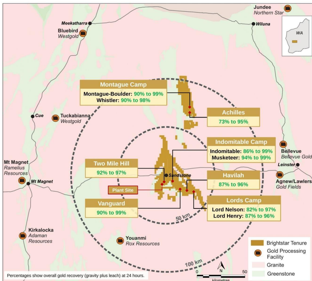
Figure 7: Sandstone deposits and metallurgical outcomes
