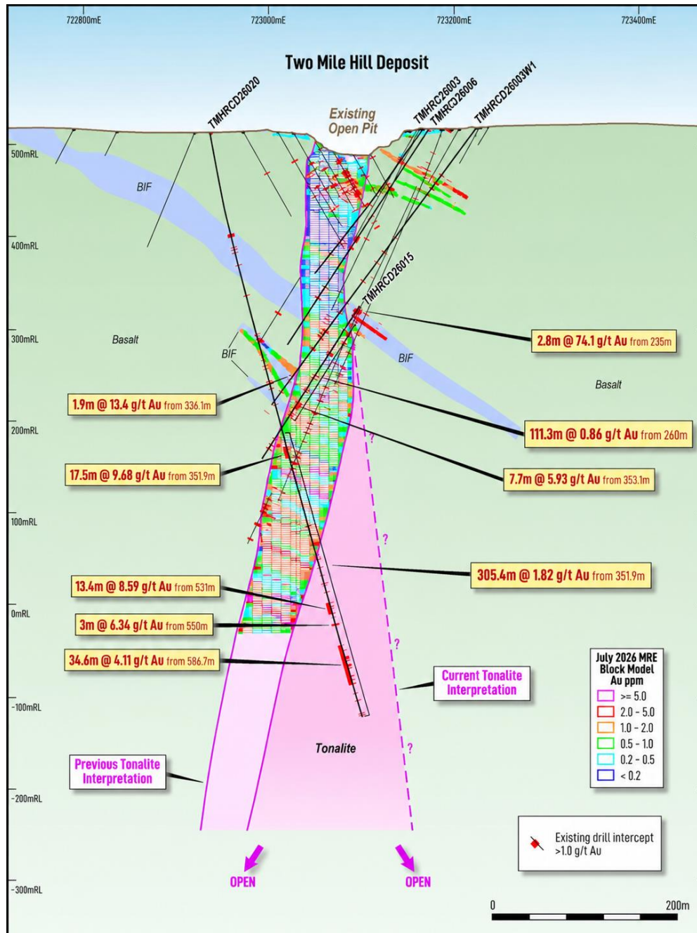
Figure 10: Cross section through drillhole TMHRCD26020 at Two Mile Hill, illustrating the then-interpreted expansion to the host tonalite, relative to the previous July 2026 MRE boundary.
