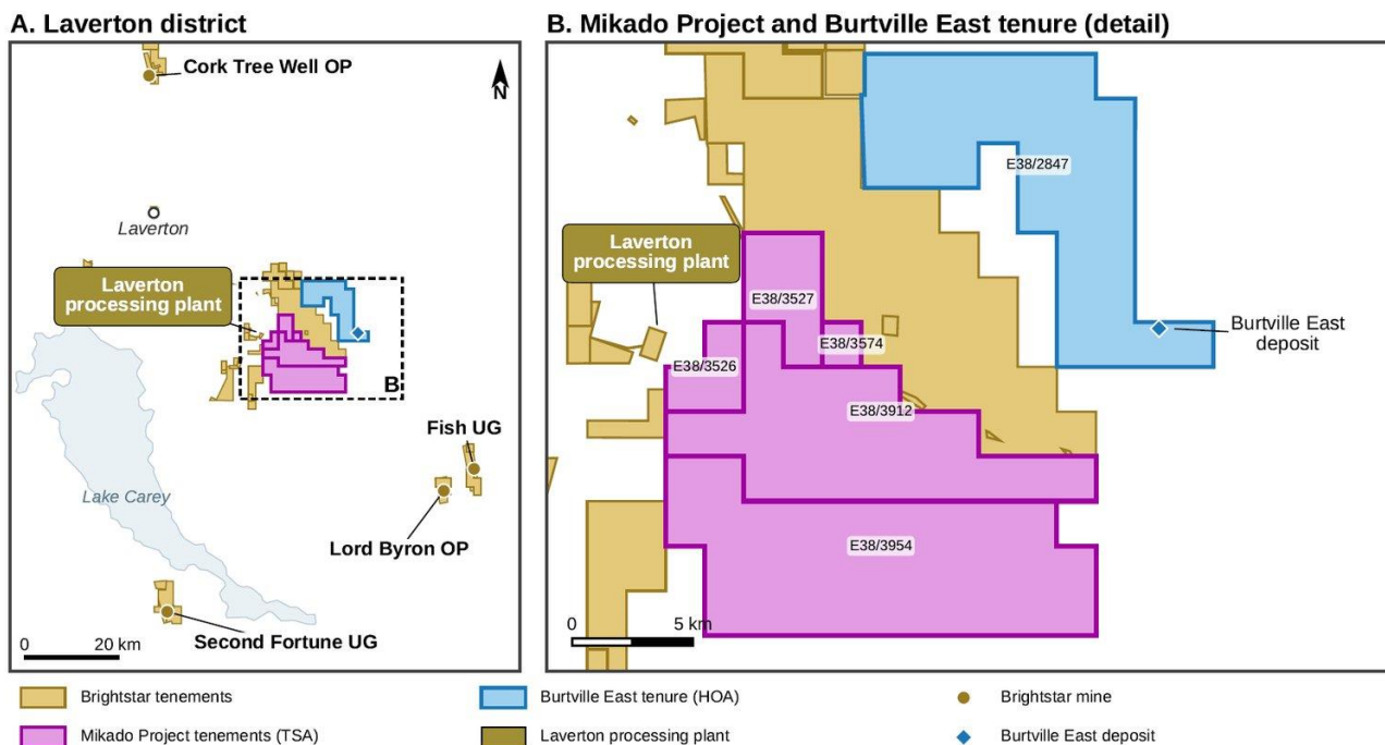
Figure 6: Laverton district (A) and detail of the Mikado Project tenements (magenta) and Burtville East HOA tenure (blue) (B)
