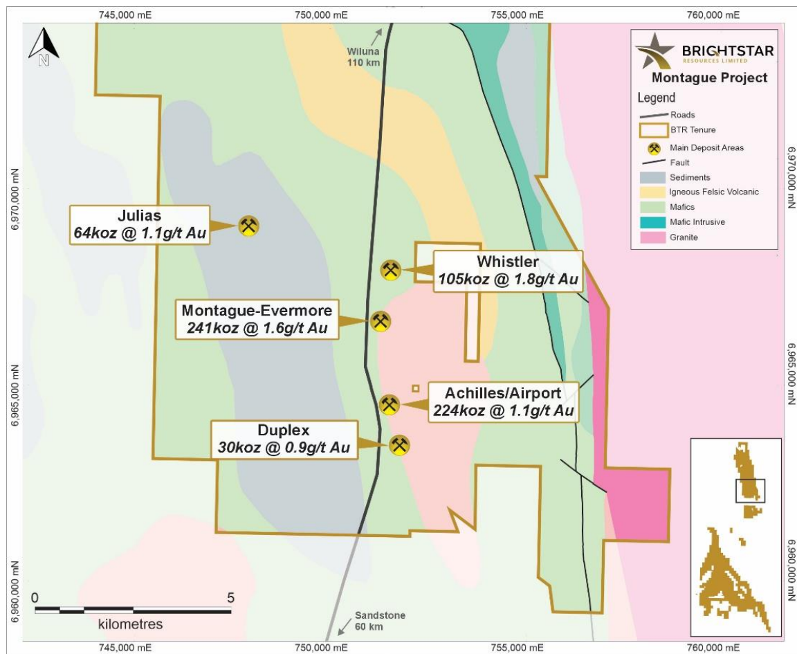
Figure 9: Geology of Brightstar's Montague Project showing deposit locations and current resources.
