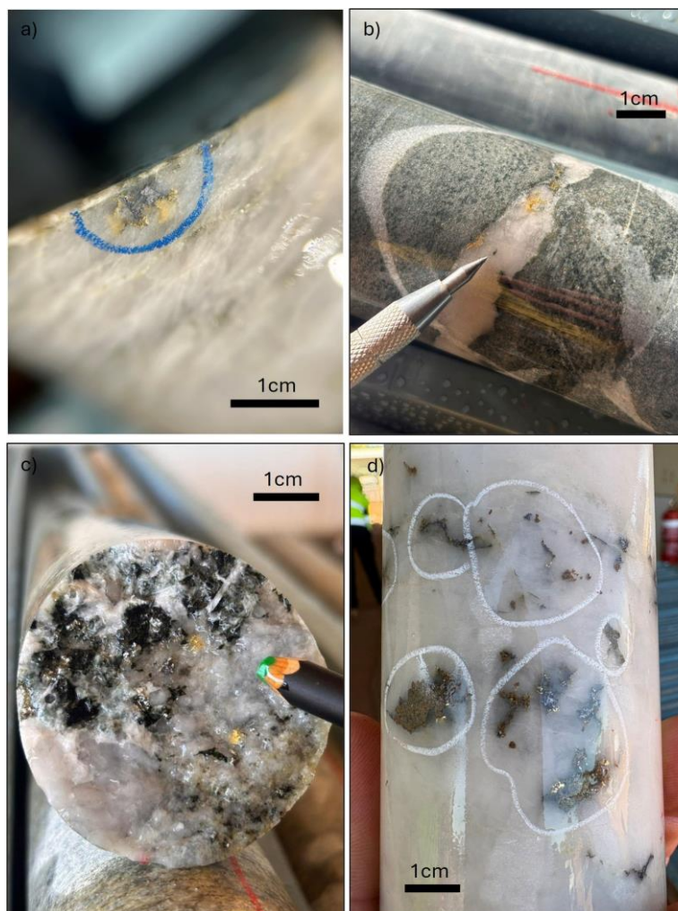
Figure 12: Examples of visible gold from 2026 diamond drilling at the Two Mile Hill Deposit; a) TMHRCD26013 at 268.25m, b) TMHRCD26010 at 174.7m, c) TMHRCD26010 at 438.75m, d) TMHRCD26009 at 302.6m.
