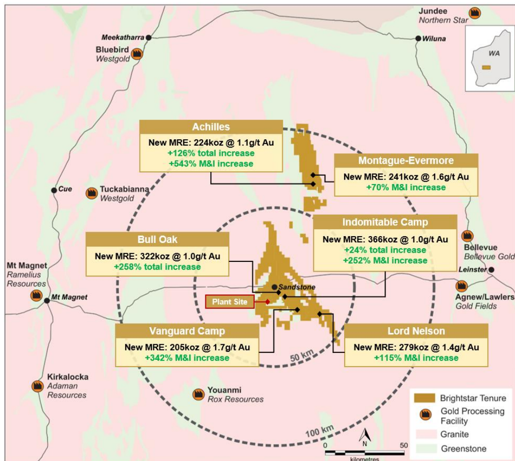
Figure 17: Brightstar's Sandstone Gold Project - interim Mineral Resource upgrades for selected deposits
