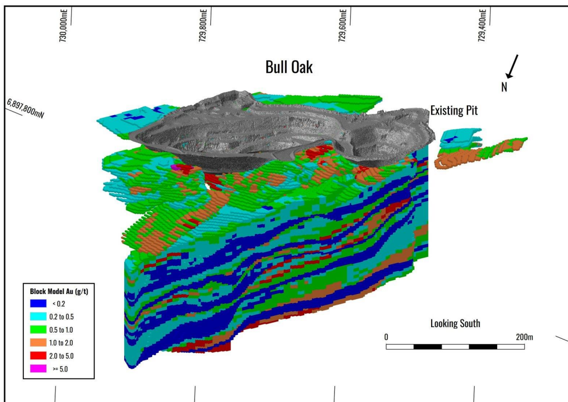
Figure 19: Oblique view looking South of the Bull Oak 2026 block model coloured by gold grade.
