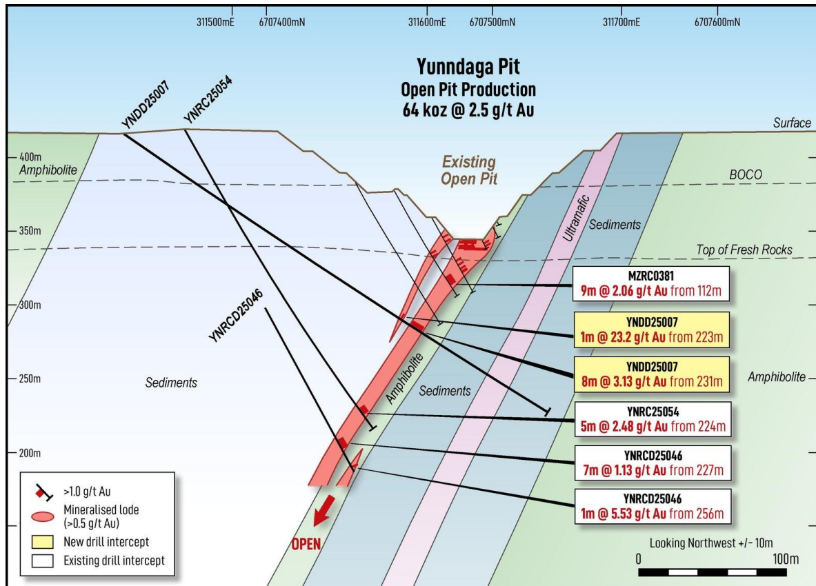
Figure 24: Cross Section at the Yunndaga Deposit
