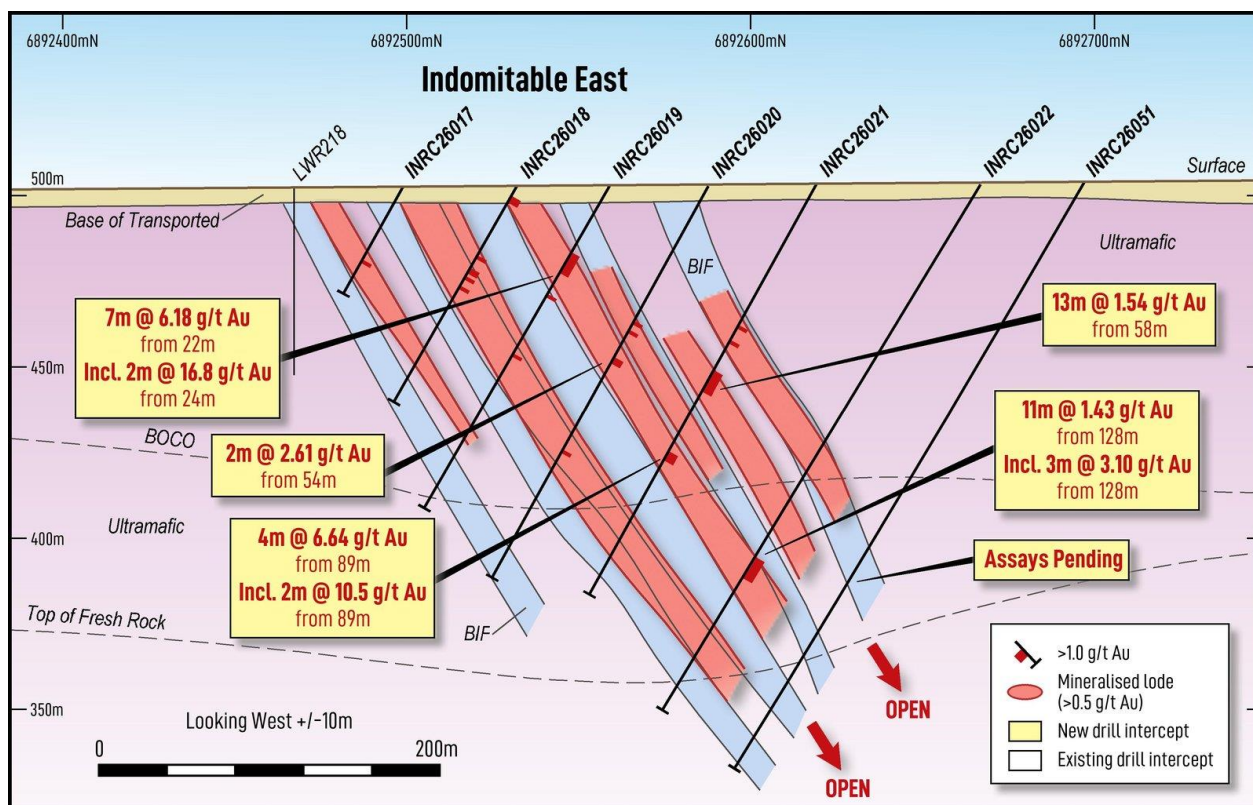
Figure 15: Cross section through the Indomitable East Deposit.
