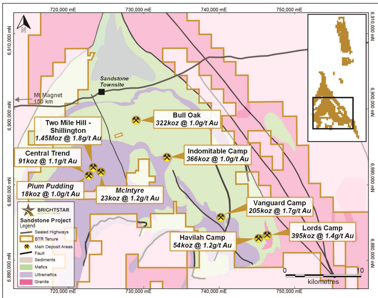
Figure 8: Geology of Brightstar's Sandstone Project showing deposit locations and current resources.
