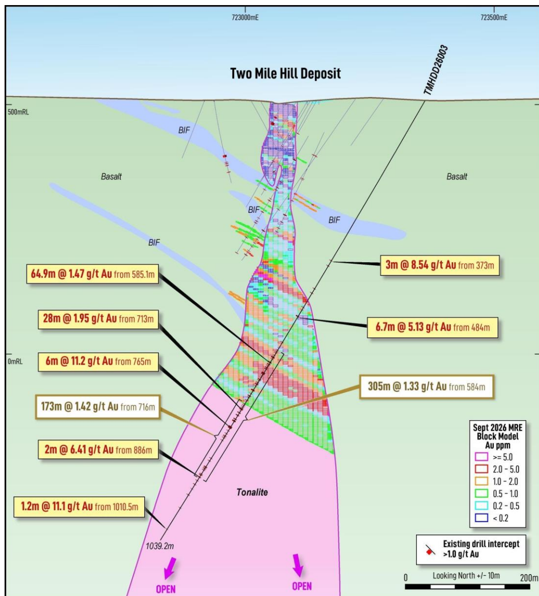
Figure 25: Cross section A-A' at the Two Mile Hill deposit, showing drillhole TMHDD26003 in relation to the existing MRE
