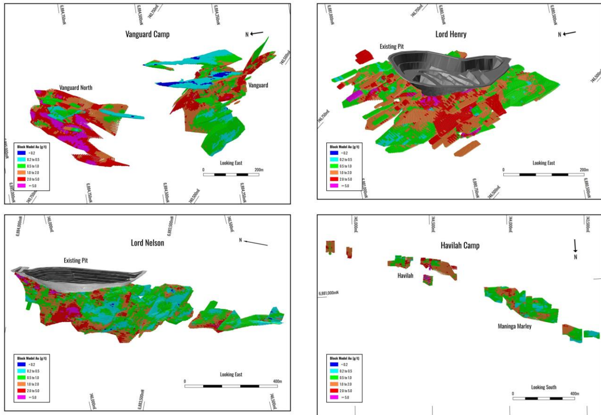
Figure 21: Oblique views of the 2026 block models for Vanguard Camp, Lord Henry, Lord Nelson, and Havilah Camp.
