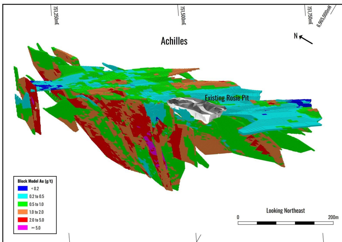
Figure 20: Oblique view looking East of the 2026 Achilles block model.
