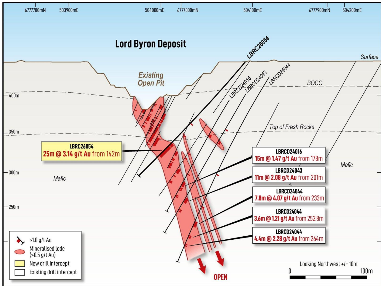
Figure 23: Cross section at the Lord Byron Deposit
