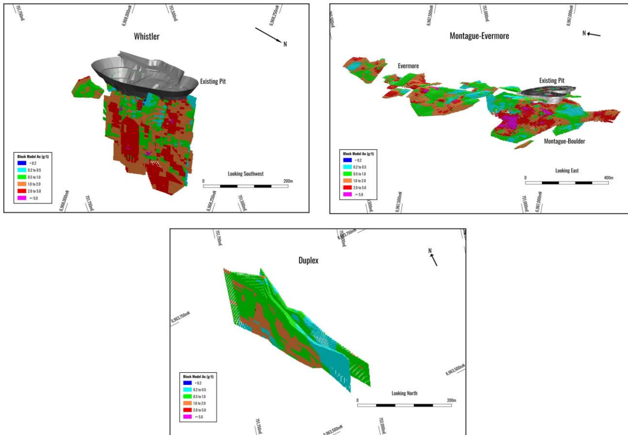
Figure 22: Oblique views of the 2026 block models for Whistler, Montague-Evermore, and Duplex, all located at the Montague Project
