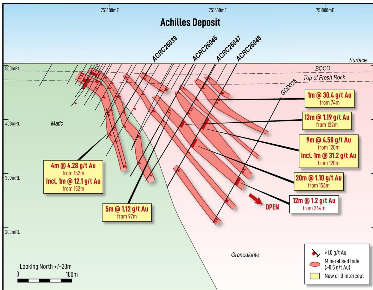
Figure 16: Cross section through the Achilles Deposit.
