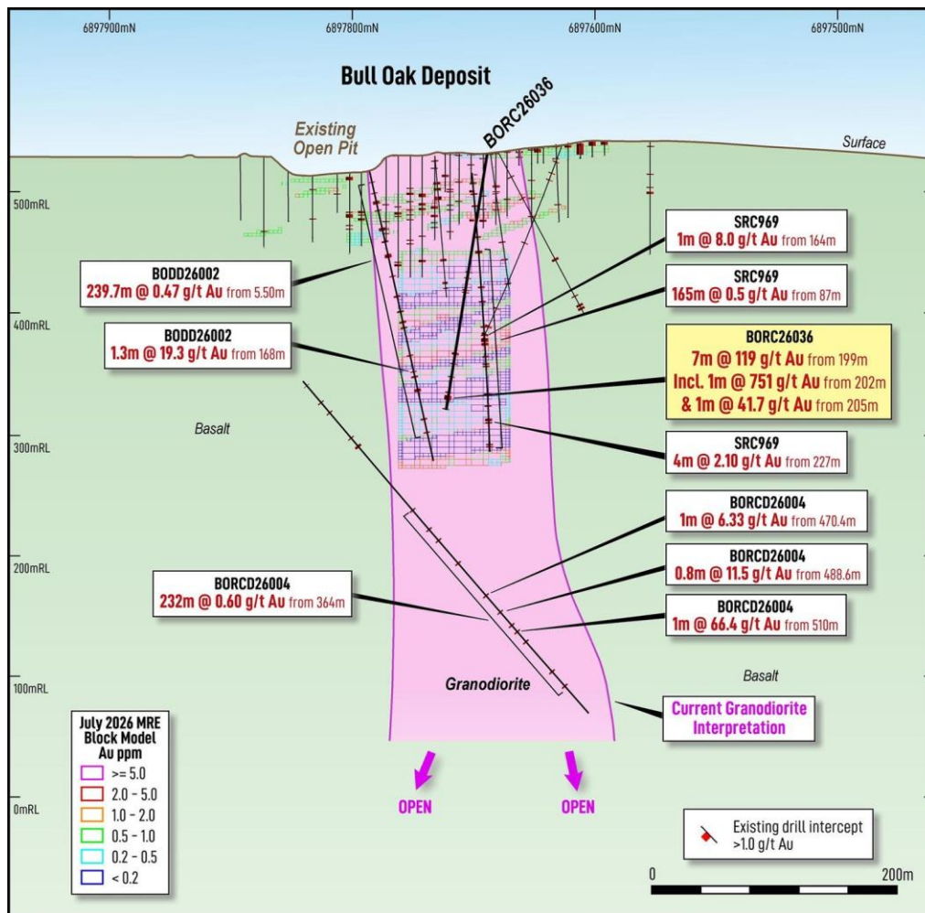
Figure 14: Cross section A-A' at the Bull Oak deposit, displaying recent drilling in relation to the existing data and MRE. Looking east, section width is +/- 10m.
