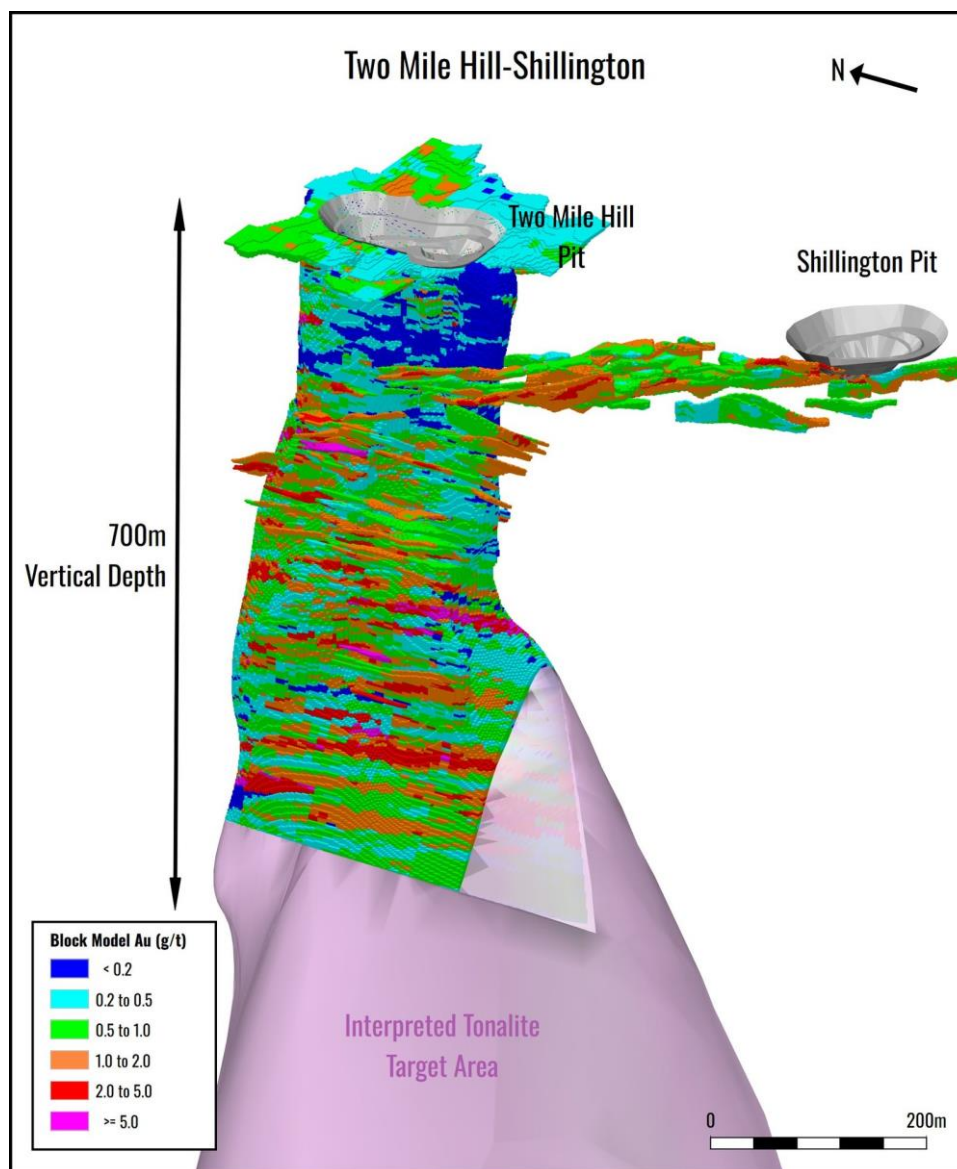
Figure 18: 3D Oblique view of the block model for the September 2026 Two Mile Hill-Shillington MRE update. Due to a lack of drilling the MRE has been truncated to the south and at depth. These areas remain open for drill testing.
