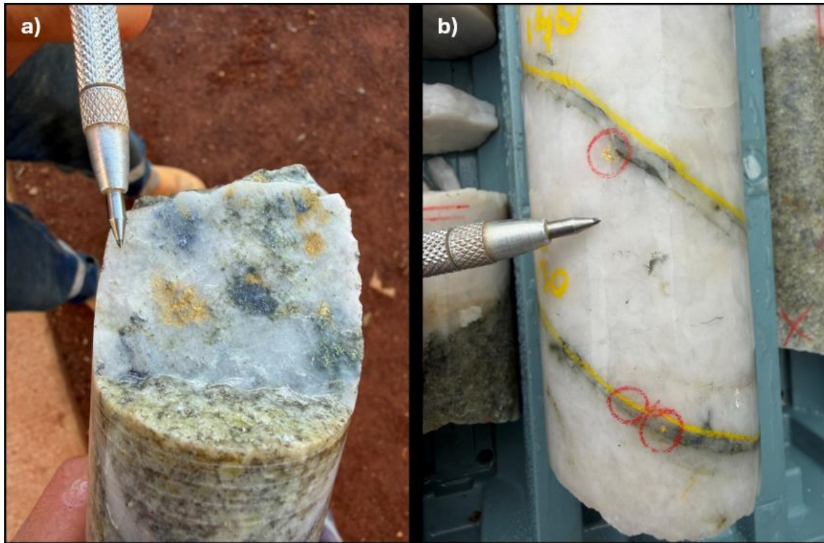
Figure 11: Examples of visible gold observed in TMHRCD26020 drill core. a) at 363.1m, gold observed on the margins of a quartz vein associated with galena and pyrite, within sericite-altered tonalite. Contained within an intercept of 17.5m @ 9.68g/t from 351.9m. b) at 481.5m, gold (circled in red) within a laminated quartz vein associated with pyrite and galena. Contained within an intercept of 0.5m @ 10.9g/t Au from 481.2m. In both images the core is approximately 5cm wide.
