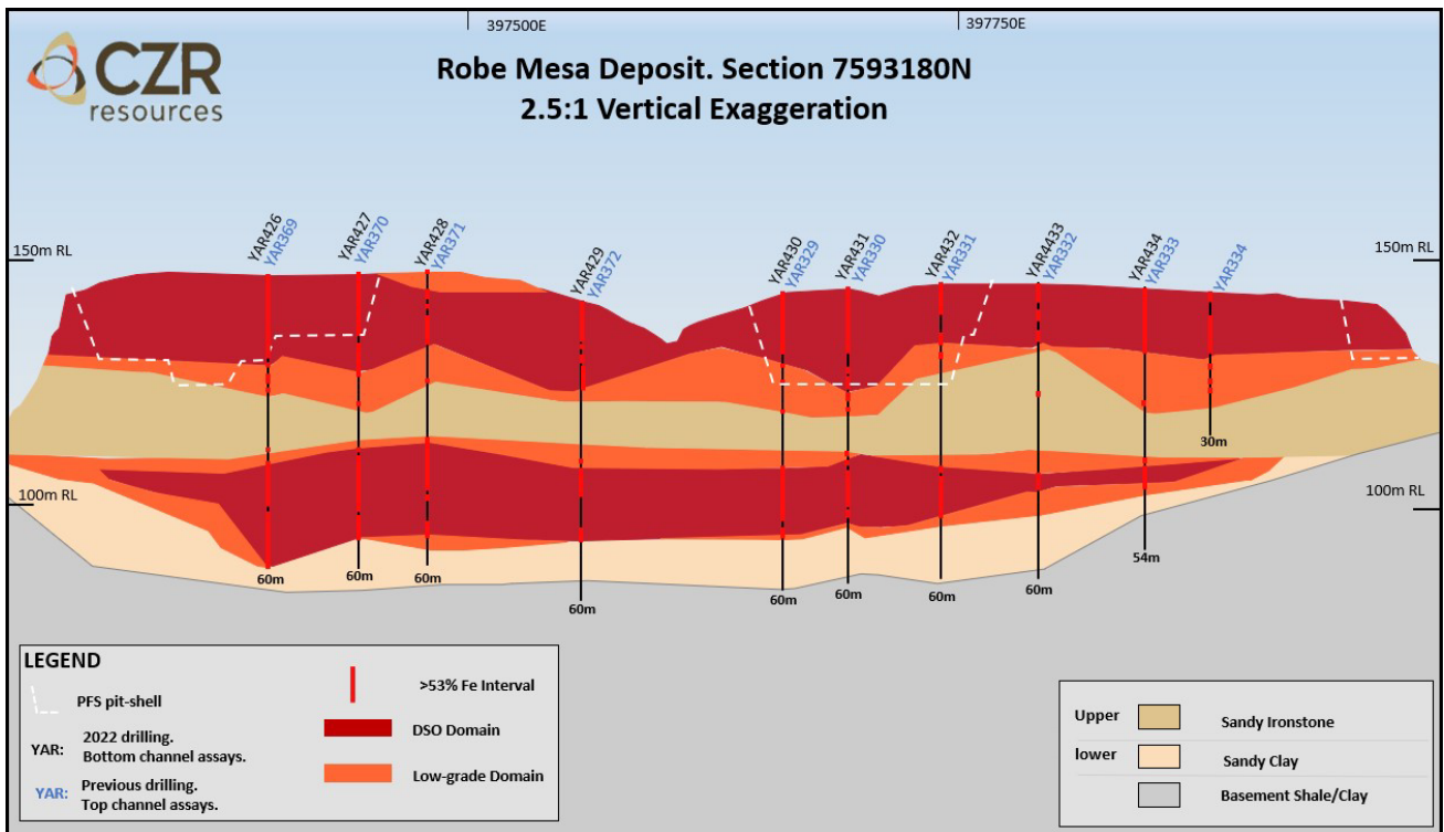
Figure 4. Cross Section 7593180
