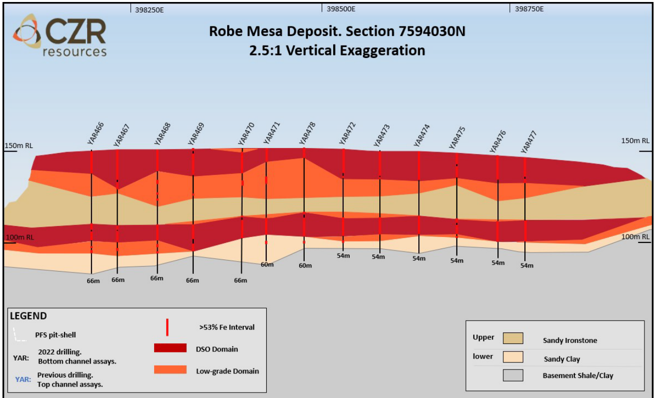
Figure 3. Cross Section 7594030 – Northern Extension, outside current Mineral Resource estimate and pit designs
