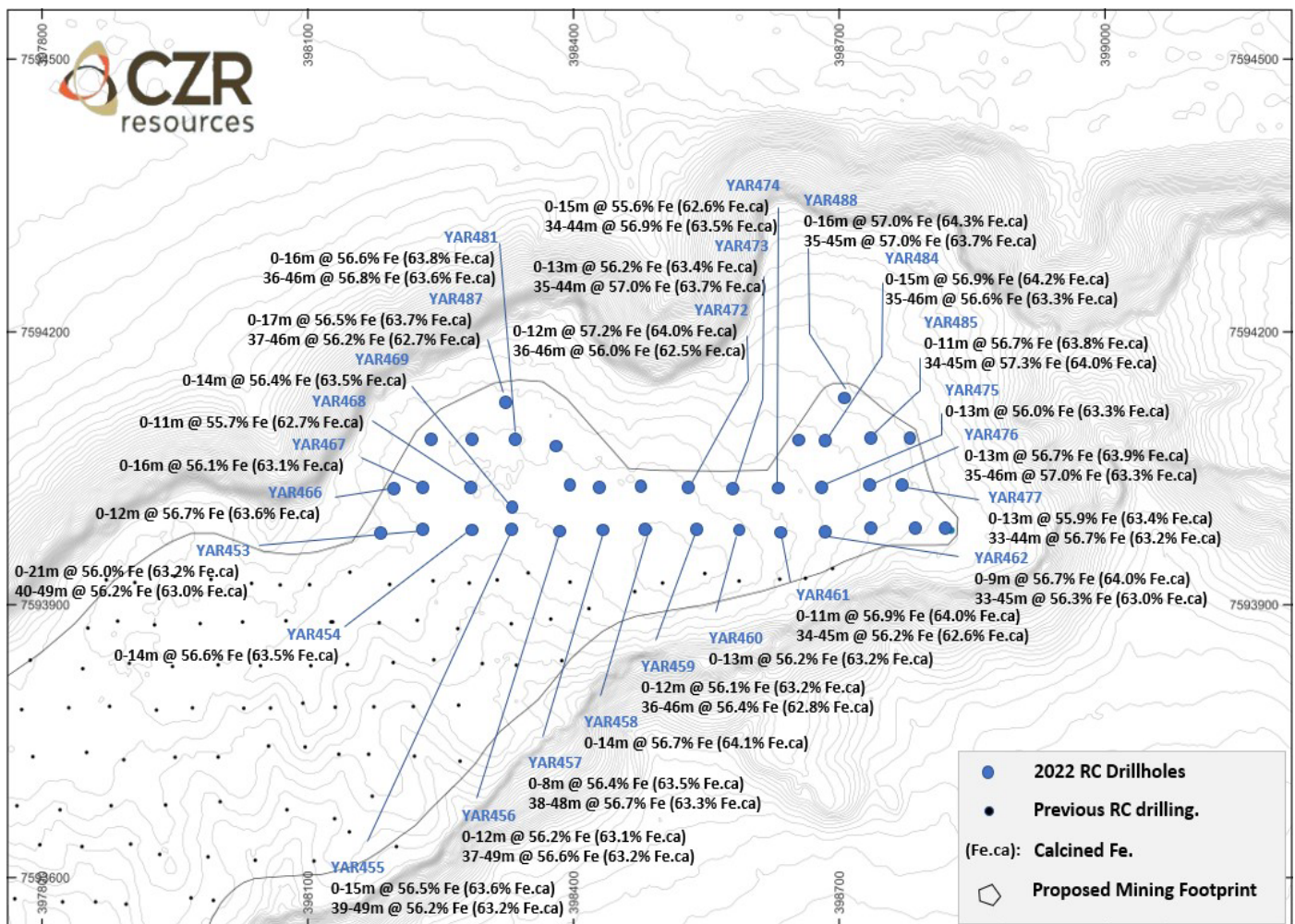
Figure 2. Location of RC drill-holes from the Northern Extension (outside current Mineral Resource) with a selection of significant intersections (refer to Table 1 for a full list of significant intersections)
