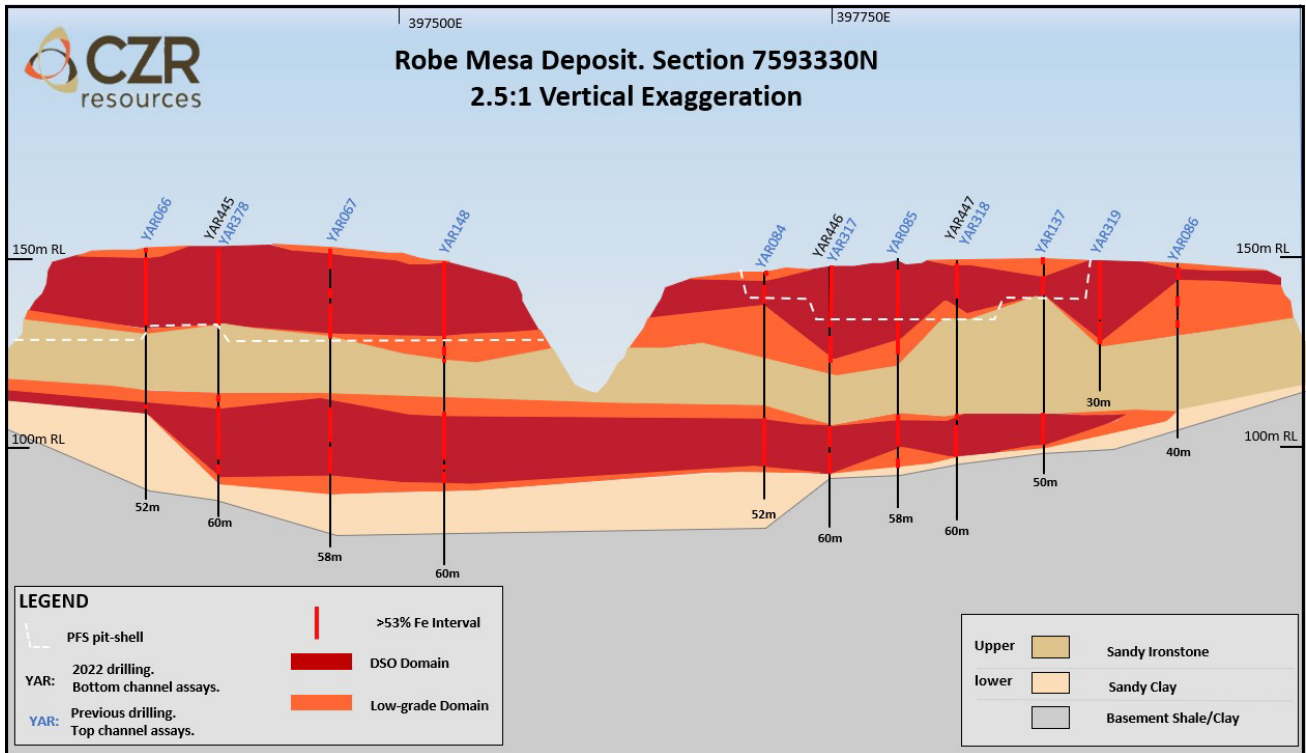
Figure 5. Cross Section 7593330
