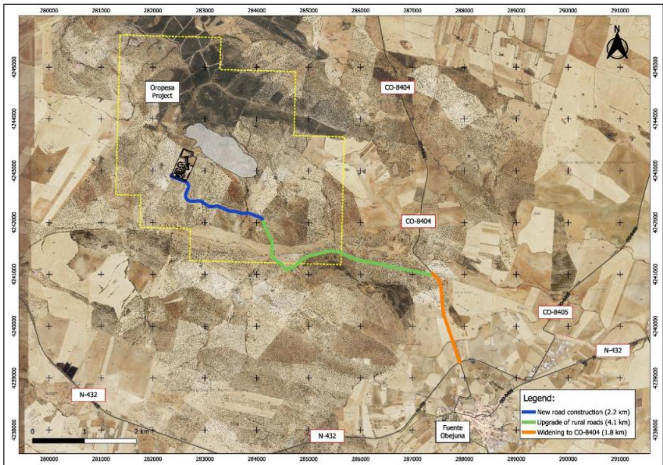
Figure 2. Approved section of dedicated site access (surface improvement and construction).
