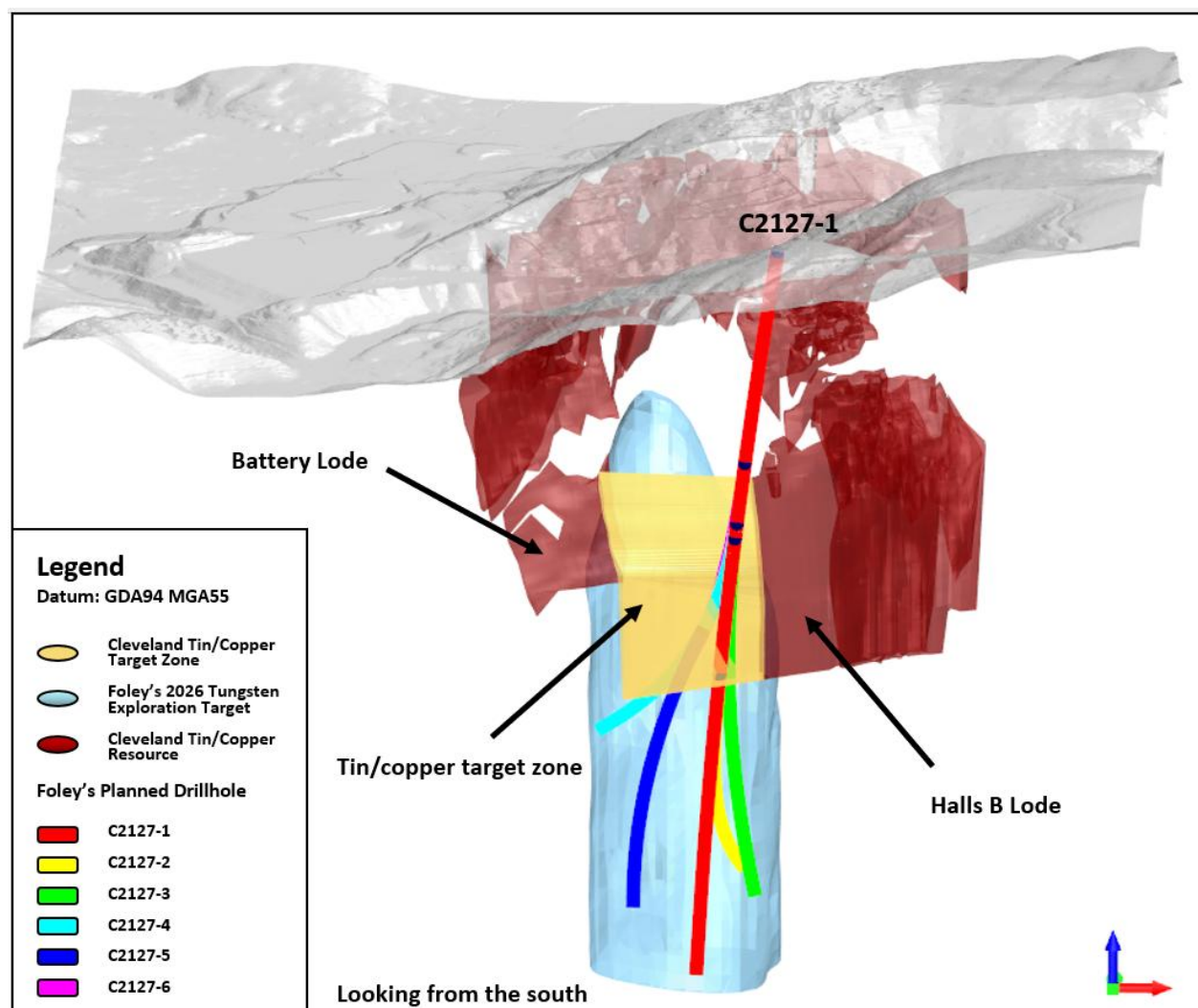
Figure 7. View looking north (from the south) of the planned drilling into the prospective tin/copper stratigraphy between the Halls B Lode and Battery Lode and then into the Foleys Zone Tungsten targets
