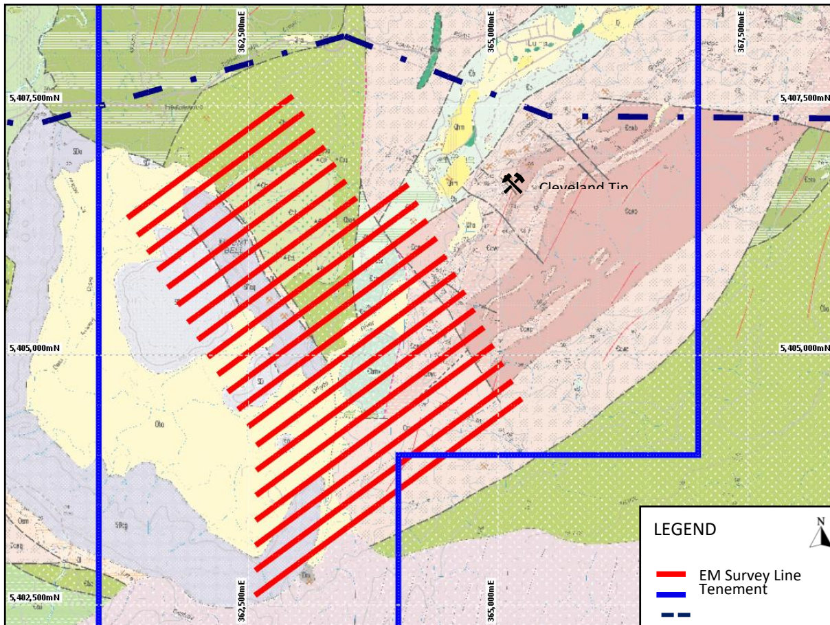
Figure 6. Planned 35 line-kilometre helicopter-borne electromagnetic
