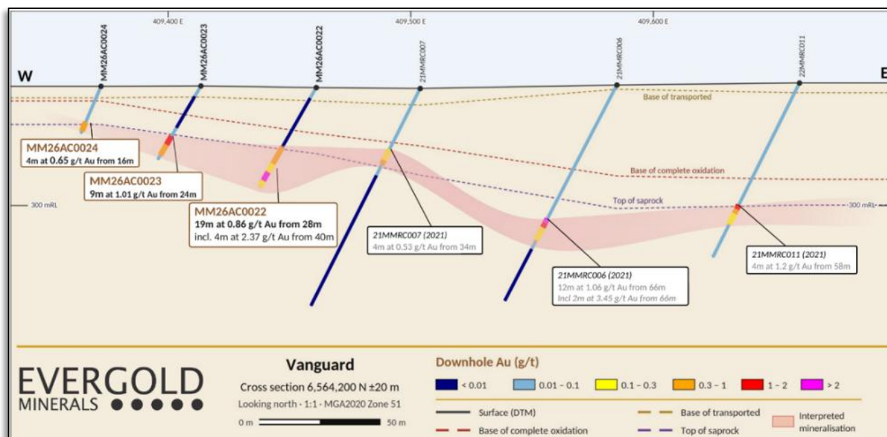
Figure 4: Vanguard – cross section 6,564,200N (±20m), looking north, showing 2026 aircore and 2021 RC drilling
