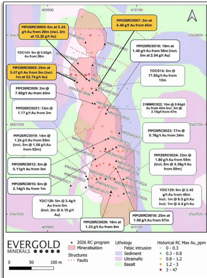
Figure 2: Duchess of York – 2026 RC drilling plan showing significant intercepts, historical drilling and interpreted mineralisation
