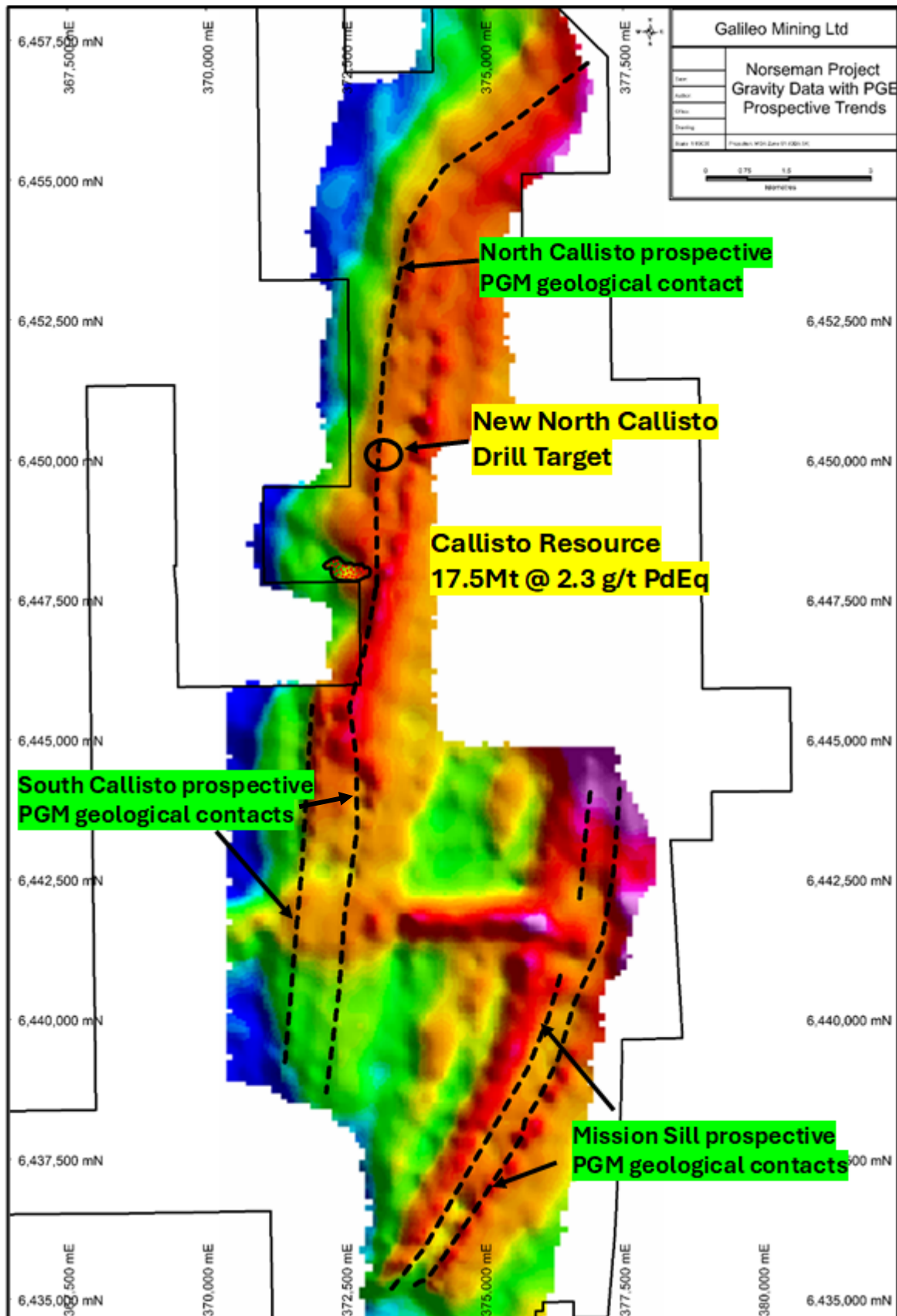
Figure 3: Norseman Project residual gravity image with existing Callisto resource, upcoming drill target at North Callisto, and prospective PGM geological contact zones
