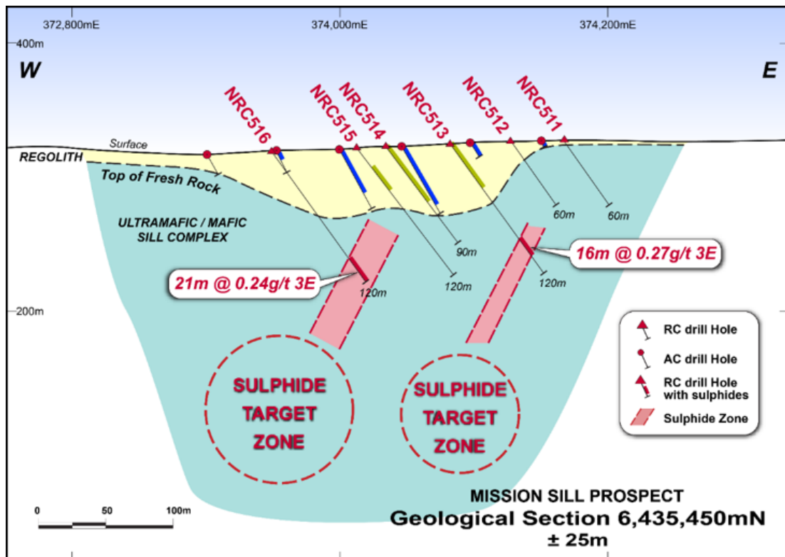
Figure 6: Mission Sill section 6,435,450N with sulphide target zones at depth. Drill hole NRC516 finished in mineralisation.
