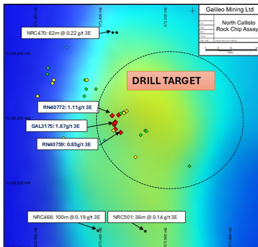
Figure 2: Rock chip sampling from North Callisto prospect with previous drilling (black stars) and upcoming drill target area (dotted ellipse). TMI magnetic background.
