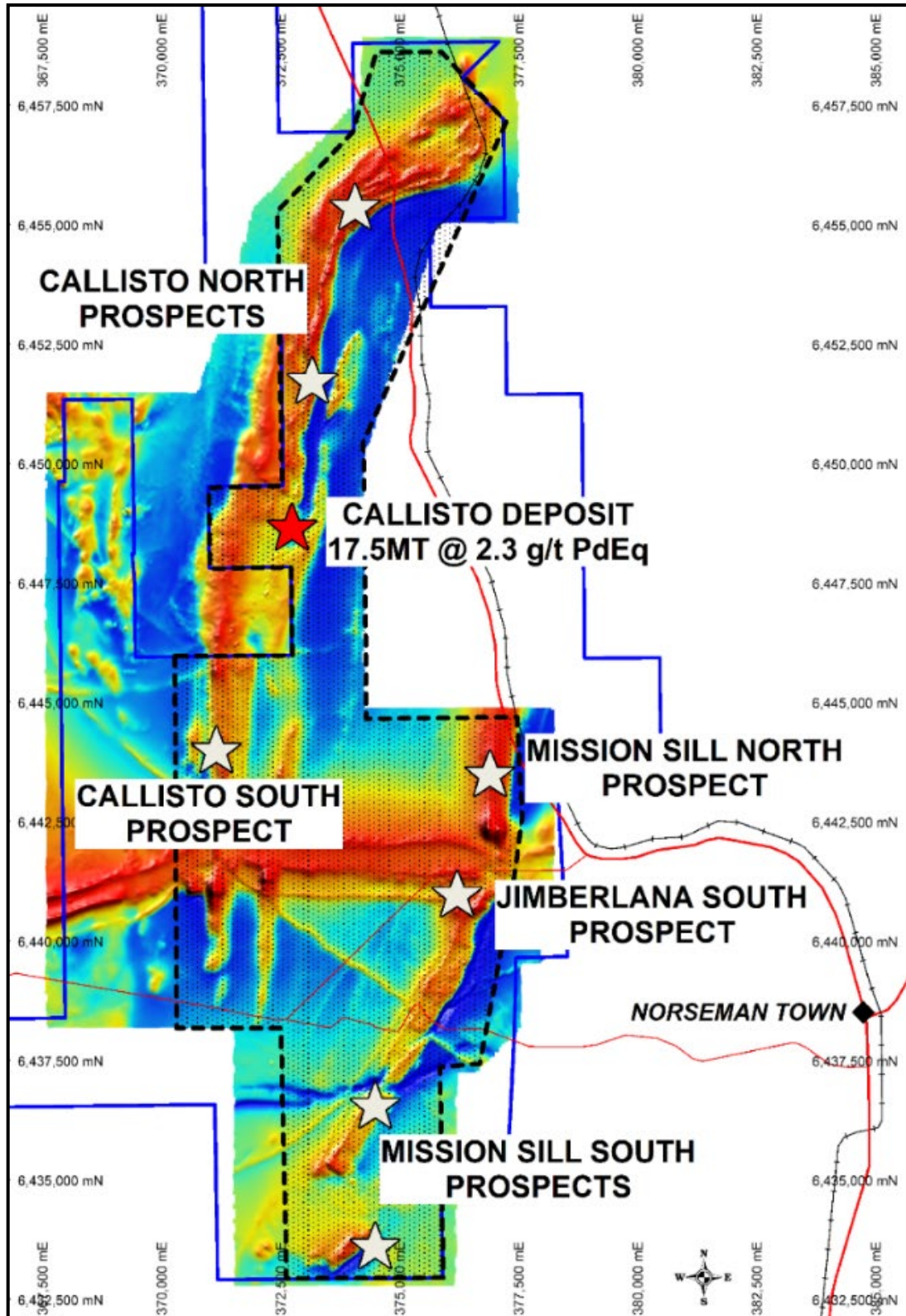
Figure 1: Norseman Project regional/prospective trends map.
