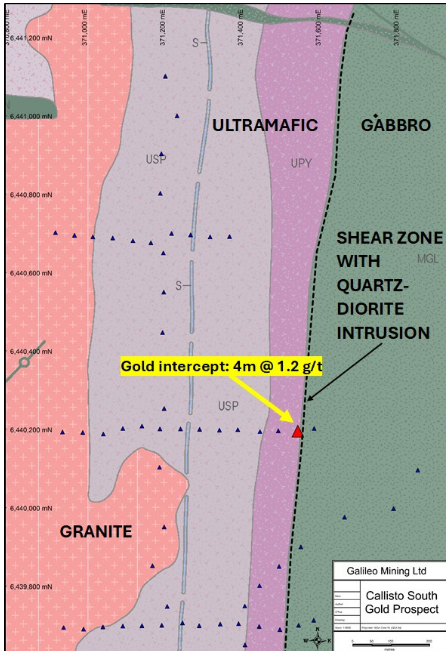
Figure 7: Callisto South gold prospect with air core drilling (triangles), gold drill intersection, 10k mapped geology and interpreted shear zone.
