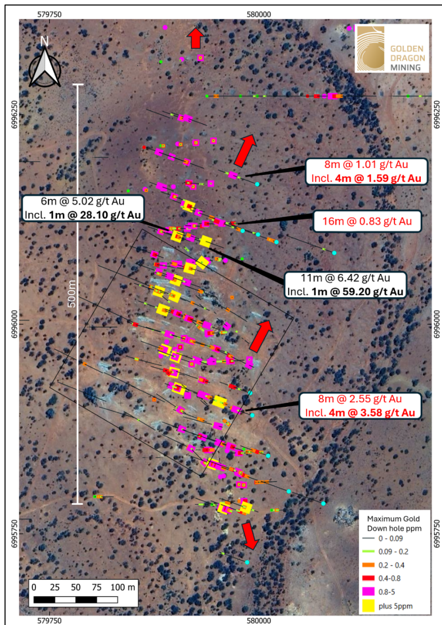
Figure 1 - Previous high-grade downhole gold intersections at the Coodardy Prospect, with intersections >5 g/t Au highlighted in yellow. Previously reported intersections within the interpreted northeast-trending high-grade shoot have been resampled and re-assayed at 1m intervals (black text). Significant gold intersections from recent drilling are shown in red text, with drill collars shown in light blue.
