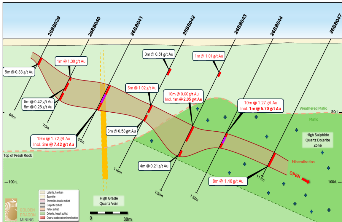
Figure 2– Drill Cross Section 69957750mN highlighting moderately east-dipping gold lode within the upper portion of an altered, pyritic dolerite and the newly identified northeast trending high grade quartz veins.
