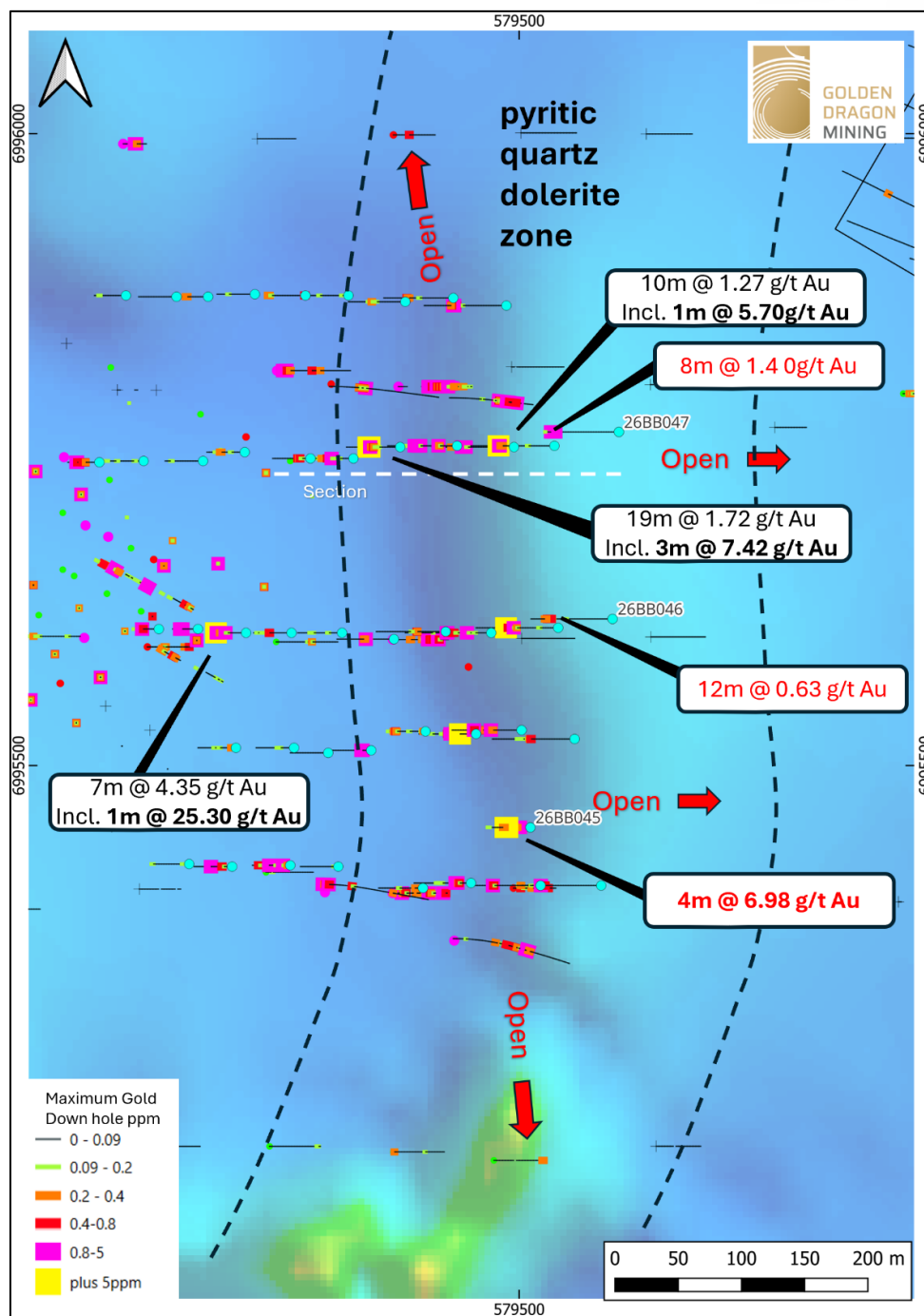
Figure 3—High-grade downhole gold intersections at the Behring Bore Prospect, with intersections >5 g/t Au highlighted in yellow. Previously reported high-grade intervals have been resampled and re-assayed at 1m intervals (black text). Significant gold intersections from recent drilling within the reporting period are shown in red text, with drill collars shown in light blue. (TMI magnetic image background).
