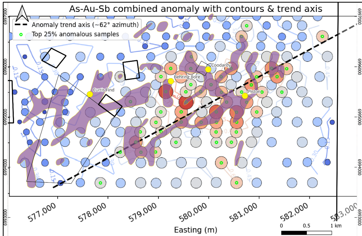
Figure 5 Combined As-Au-Sb soil geochemical anomaly score overlayed with gold only contour and known gold Prospects highlighting the strong exploration vector linking known prospects including Behring Bore, Coodardy and Piston and highlights significant potential for further discovery along this emerging mineralised trend.
