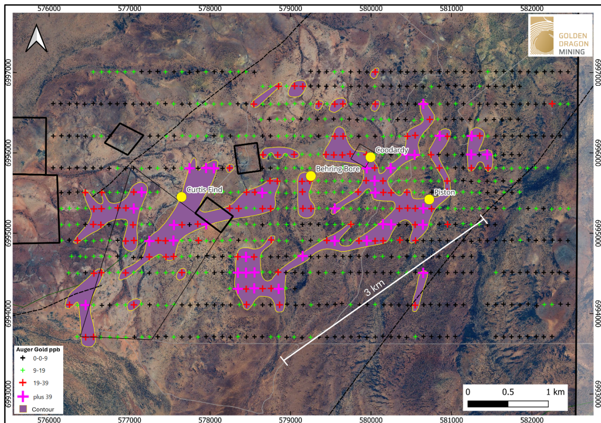
Figure 4—Significant kilometre-scale gold in auger anomalies with a north-east trending orientation, linking multiple known prospects highlights the potential for a much larger, mineralised system than previously recognise
