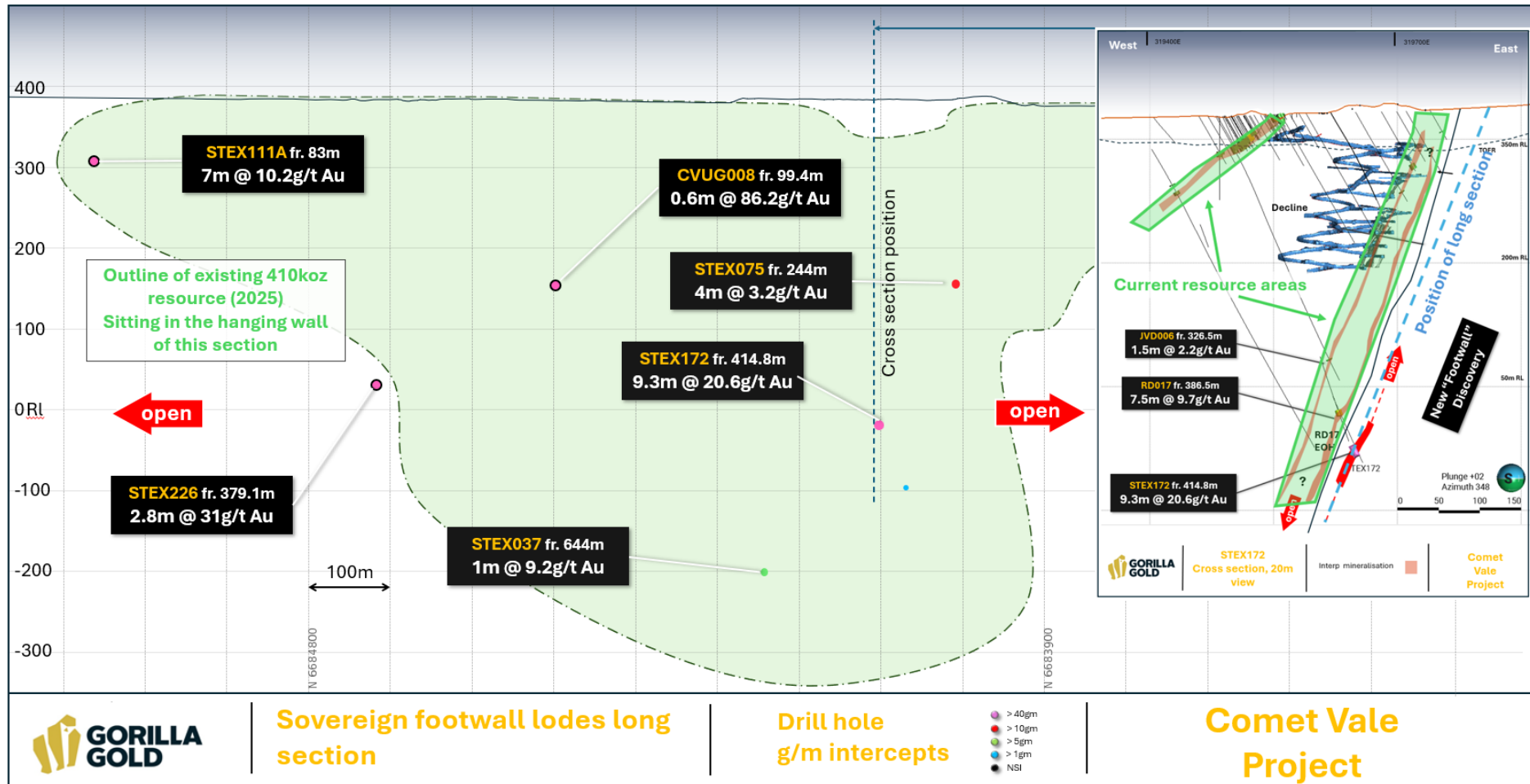
Figure 3 – Sovereign footwall lode long section.
