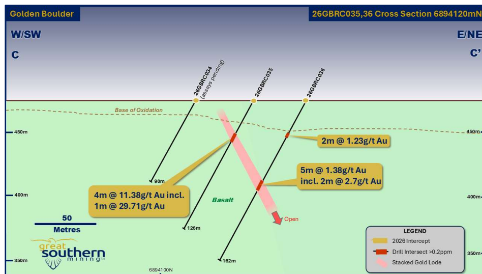
Figure 5. Interpreted cross-section at 6894120mN showing results from recent drill holes 26GBRC035 and 26GBRC036.
