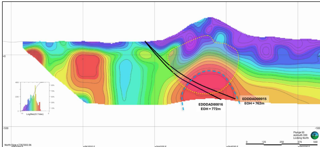
Figure 15. IP Resistivity section showing actual drill traces for diamond holes EDDDAD00015 and EDDDAD00016 at the Mt Dillon target. The blue dashed line represents the modelled resistivity anomaly, and yellow dashed line represents the modelled chargeability anomaly.
