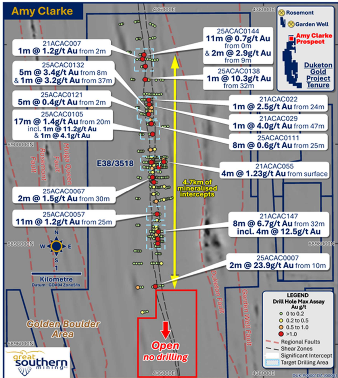
Figure 7. Map of the Amy Clarke prospect showing key mineralised trends, significant faults, and previous air core drill intercepts.
