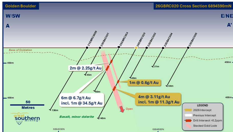
Figure 3. Interpreted cross-section at 6894590mN showing results from recent drill hole 26GBRC020 and previous drilling.
