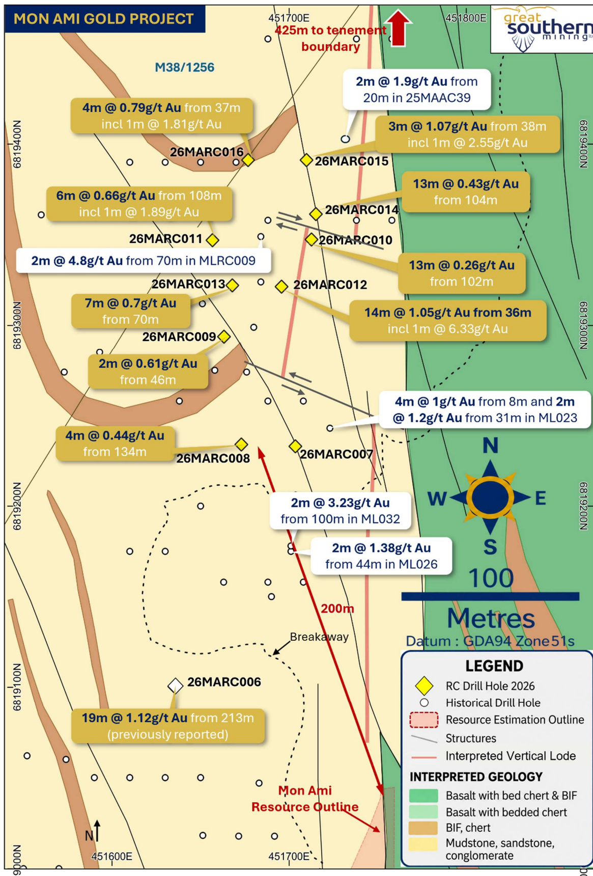
Figure 12. Map showing the location of recent reverse circulation drilling at the Blanc Platt target within the Mon Ami Gold Project, in Western Australia. Significant intersections from recent RC drilling shown in gold, historic ones in white.
