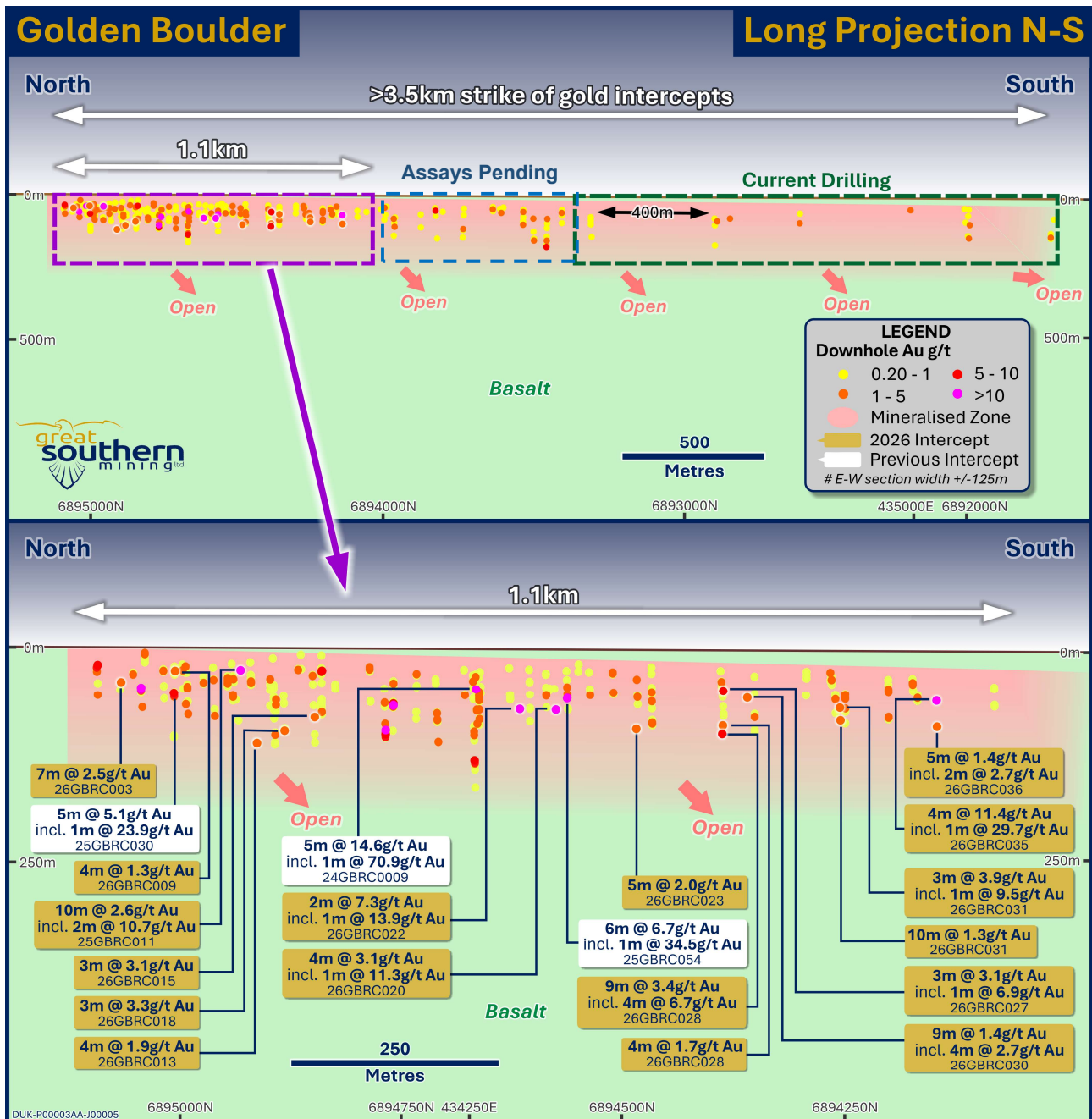
Figure 6. Long projection of the Golden Boulder Main line showing significant drill intercepts from previous drilling (white) and results received and reported in this announcement (gold).
