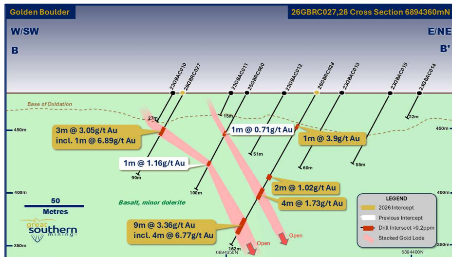
Figure 4. Interpreted cross-section at 6894360mN showing results from recent drill holes 26GBRC027 and 26GBRC028 and previous drilling.
