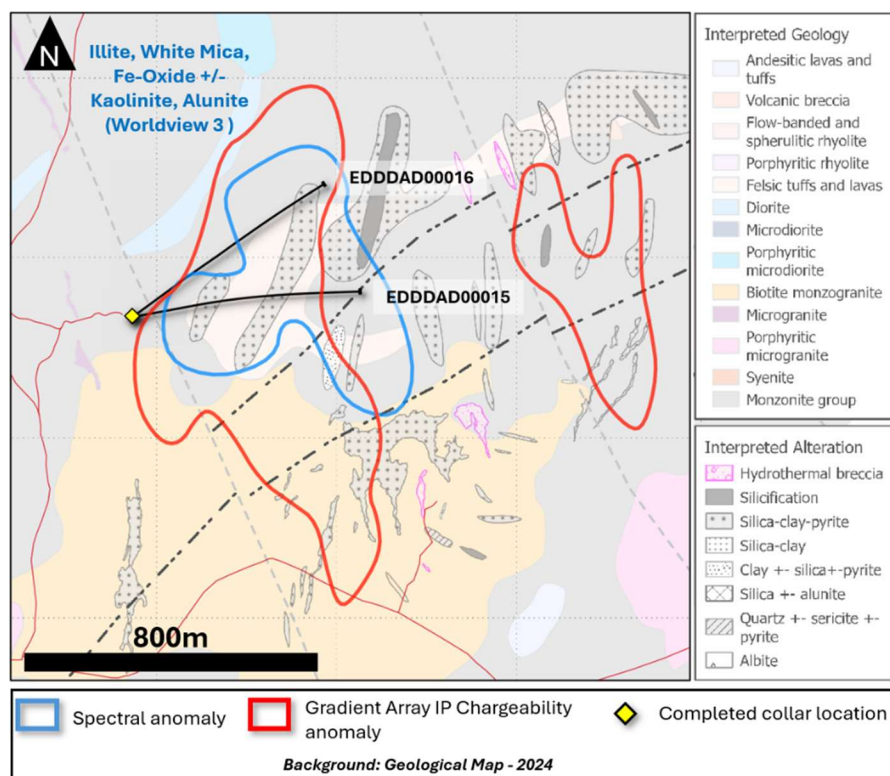
Figure 14. Actual drill traces for diamond holes EDDDAD00015 and EDDDAD00016 at the Mt Dillon target on surface geology map with spectral and gradient array chargeability anomalies highlighted.
