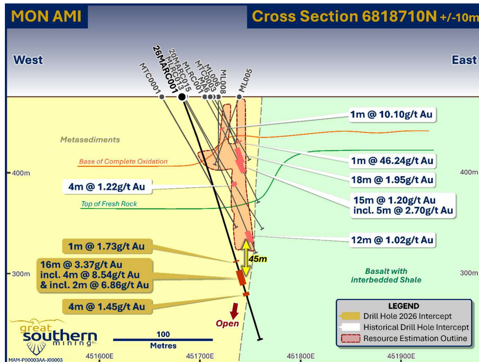
Figure 10. Cross-section through 6818710N showing recent intercepts from drill hole 26MARC001 and previous drill intercepts.
