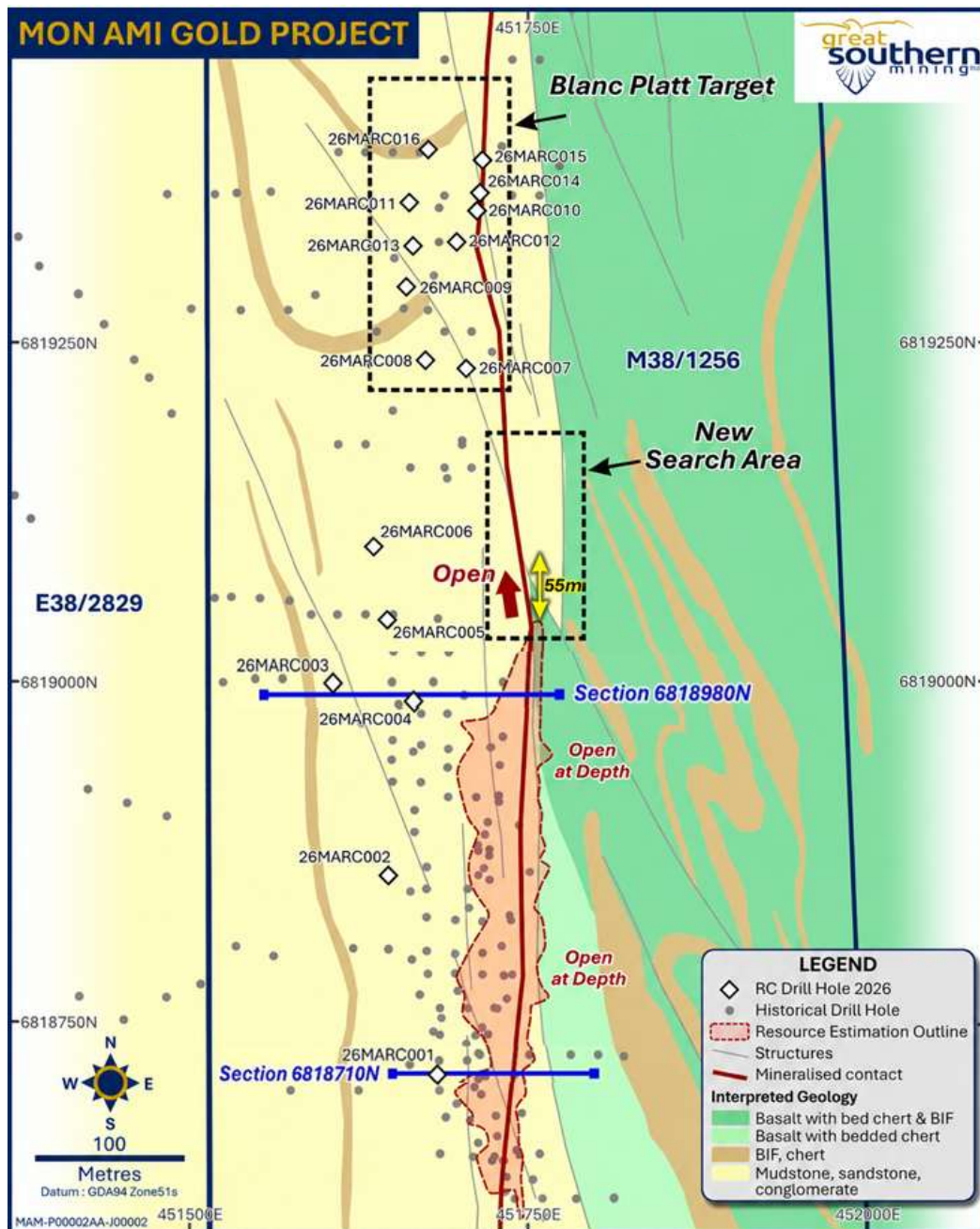
Figure 9. Plan view map of the Mon Ami Gold Project over interpreted geology showing the collar locations of recently completed reverse circulation holes, an outline of the existing JORC Mineral Resource and cross-section traces depicted in Figures 10-11 below.
