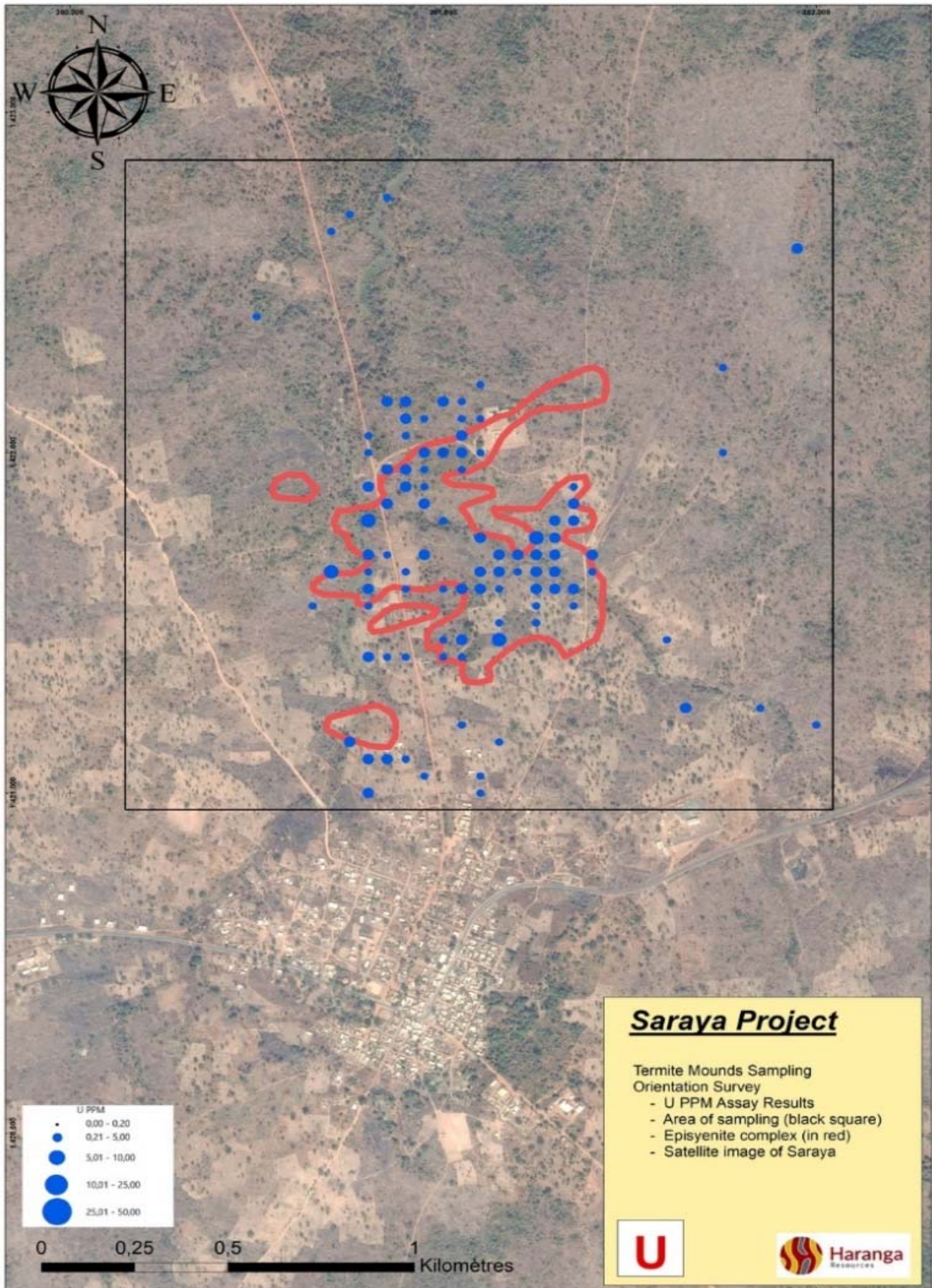
Figure 2: Termite Mound Orientation Survey– XRF Uranium Assays ppm
