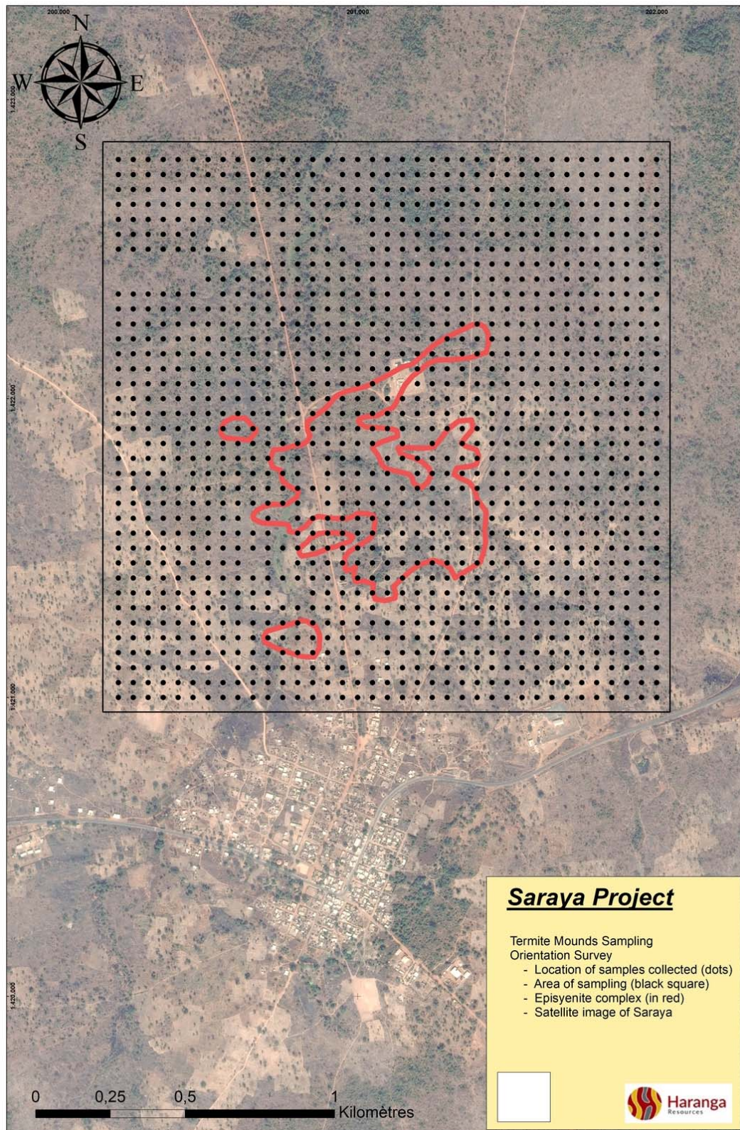
Figure 1: Orientation termite mound sample points on a 50m x 50m grid. The red outline shows the known uranium mineralised episyenite.
