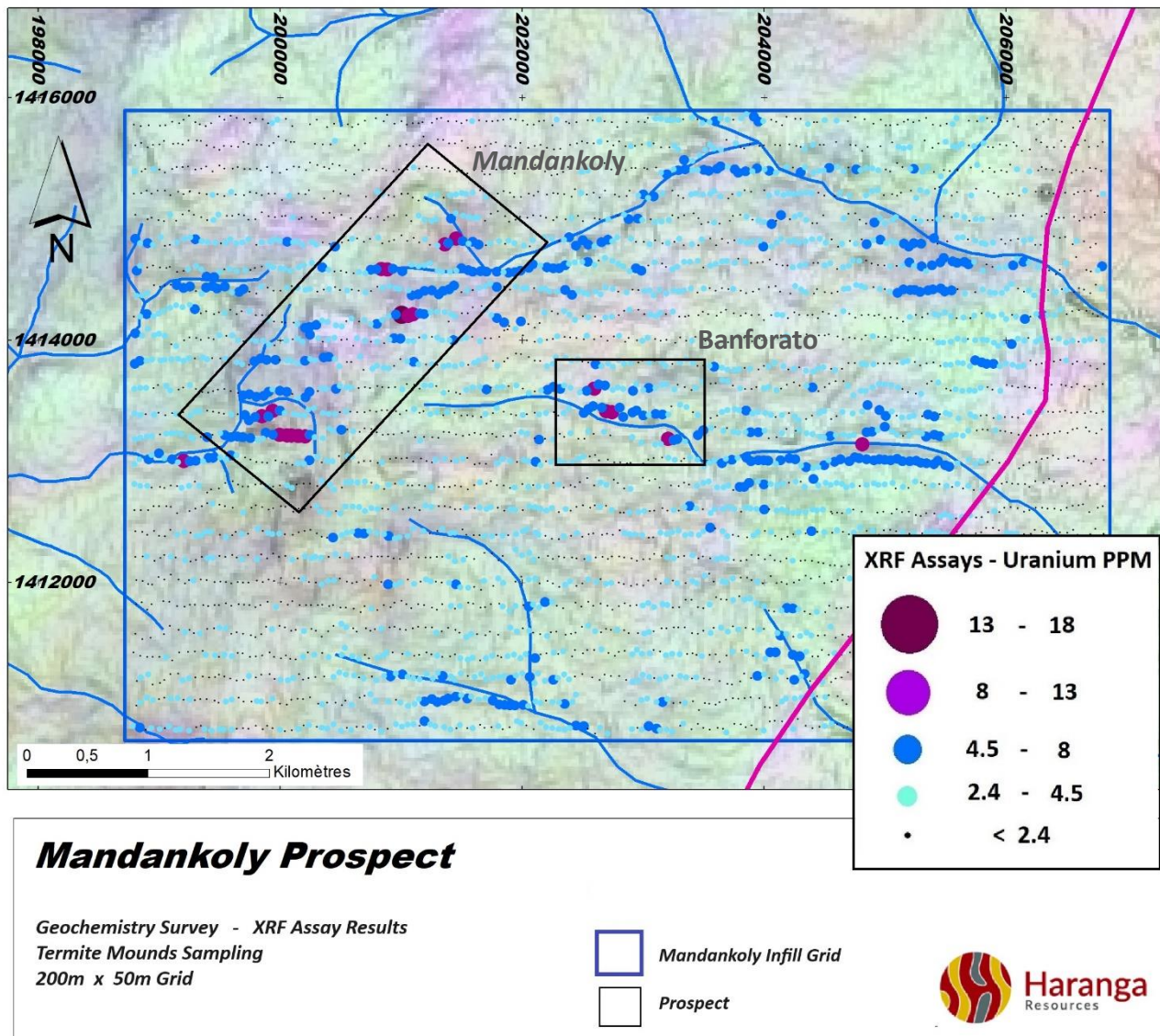
Figure 1: Uranium results for the termite mound infill sampling over the Mandankoly Grid. The results outlined two Uranium anomalies, ten kilometres South of the Saraya Maiden Resource (Figure 3). All analysis was carried out using an in-house XRF analyser.
