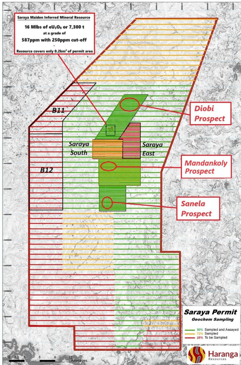
Figure 3 : Termite mound sampling progress to date: Green lines show the sampled and assayed lines, yellow lines show the sampled, but unassayed lines, while the red lines shows remaining program to be completed. +70% of the permit surface has been covered by the 1000m x 100m sampling survey, with two more blocks B11 and B12 in preparation for sampling. The first four Infill grids (200mx50m) defining the central area of the permit have been completed and the fourth grid (Saraya South) will be assayed by the end January. A fifth infill, Saraya East, is being sampled.
