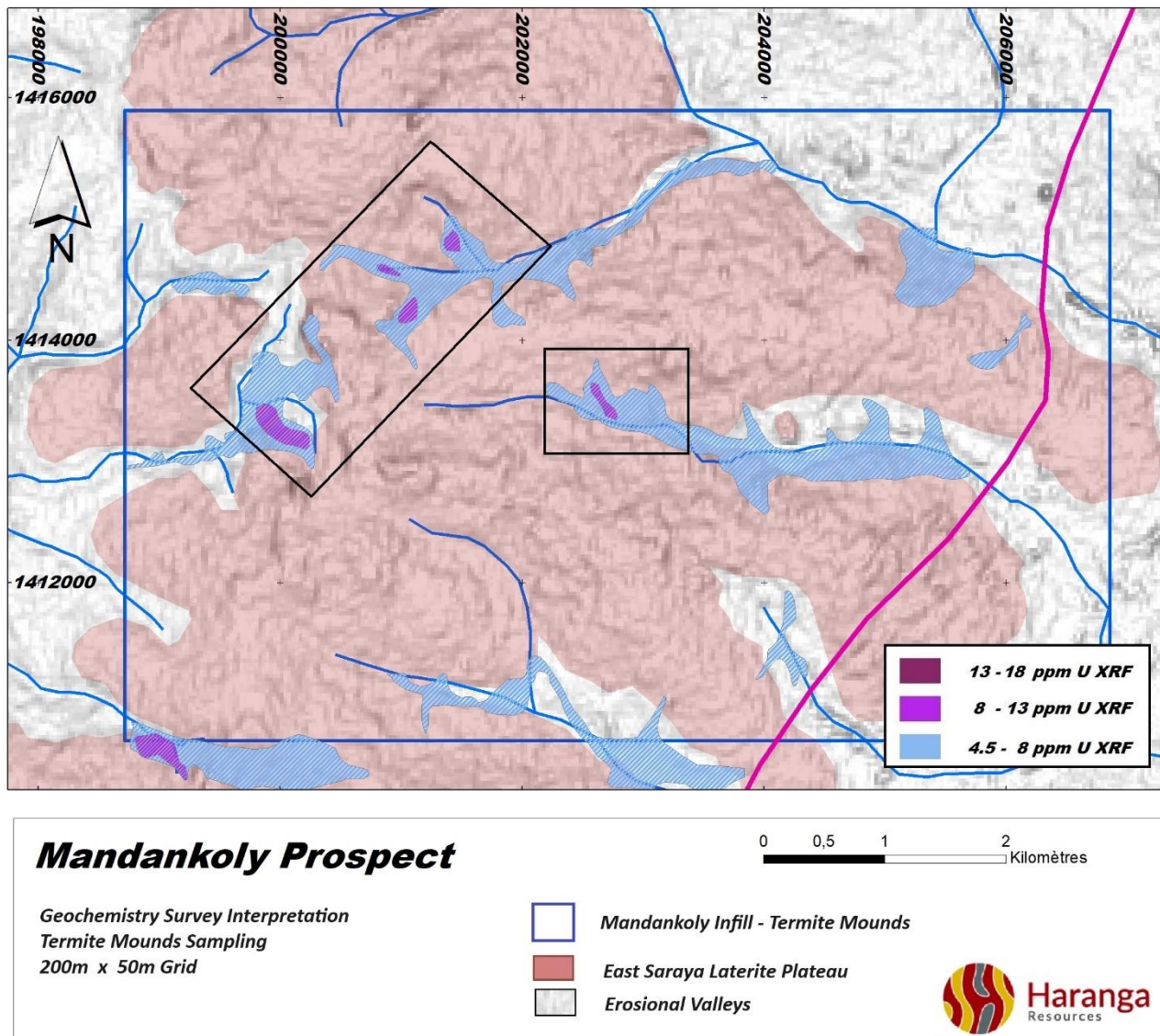
Figure 2: Interpretation of termite mound infill sampling results for the Mandankoly Grid. The main uranium anomalies detected are aligned along a NE trend of +2km long.
