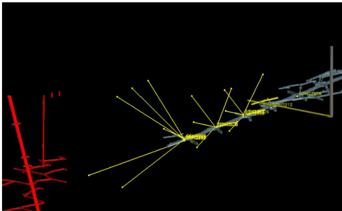
Figure 6: Phase 2 Drilling Program - viewed towards an azimuth of 283°. Stringbean Alley Decline in grey, Old Lincoln workings in Red, Mutual shaft and crosscut in grey and yellow.
