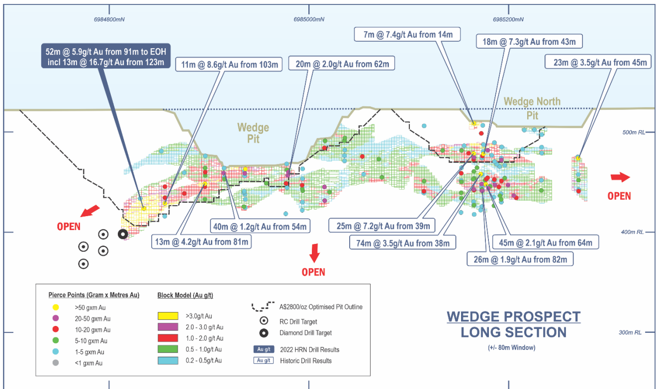
Figure 1: Wedge Prospect long section showing gold intercept gram x metre pierce points, historic open pit, A$2,800/oz optimised pit shell, block model, diamond hole mineralisation pierce point and proposed RC drilling mineralisation pierce points.
