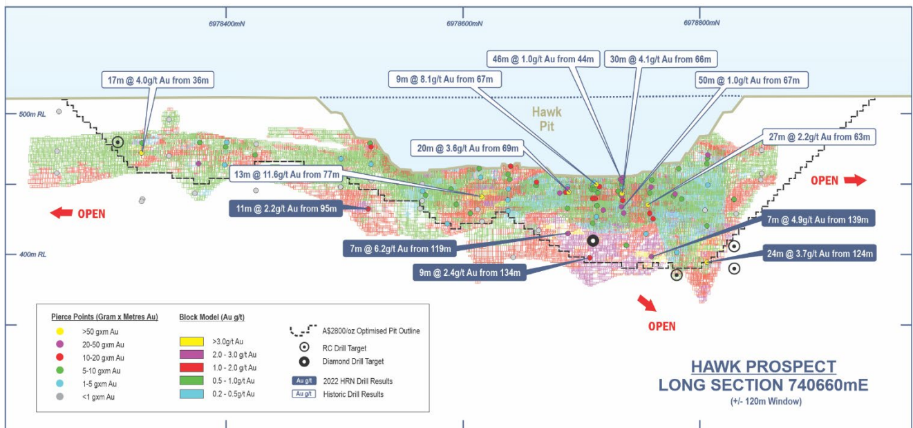
Figure 3: Hawk Prospect long section showing gold intercept gram x metre pierce points, historic open pit, A$2,800/oz optimised pit shell, block model, diamond hole mineralisation pierce point and proposed RC drilling mineralisation pierce points.
