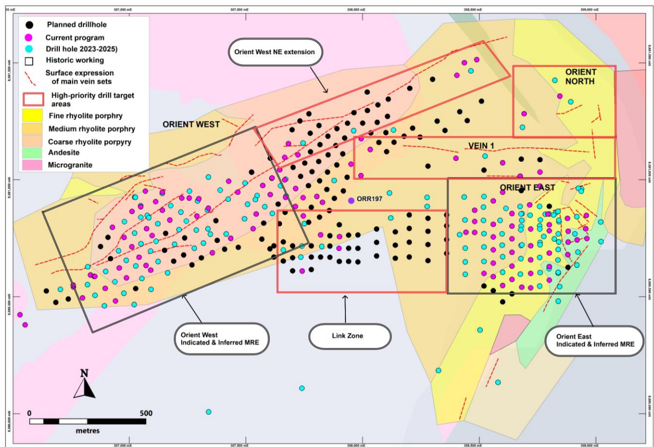
Figure 3 Orient East & West JORC Resource MRE
