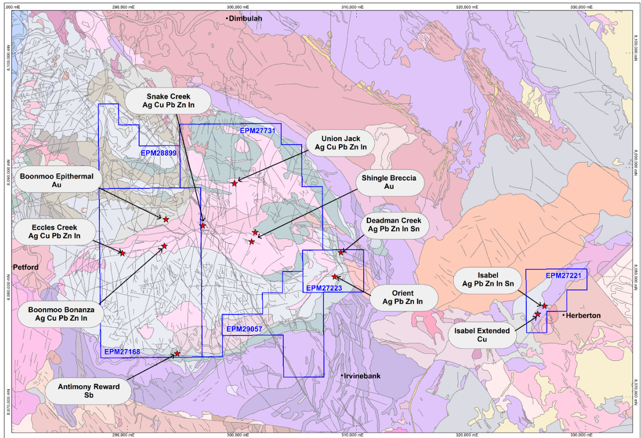
Figure 4 Herberton Project Regional Exploration Targets
