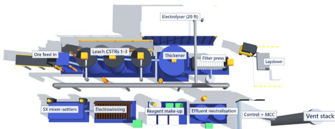
Figure 2 – Alpha Plant initial design
