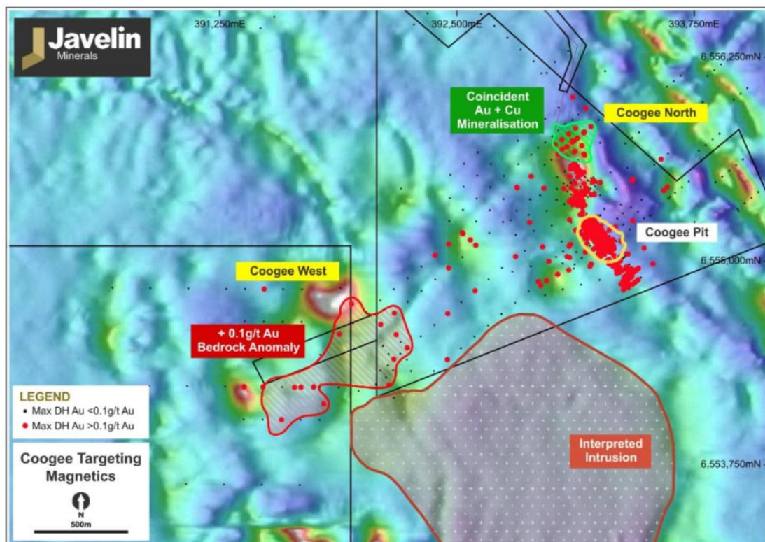
Figure 4 – Coogee Project airborne magnetics with historic drilling –maximum downhole gold(>0.1g/t Au). Note the location of the extensive bedrock gold anomaly at Coogee West and the coincident gold-copper mineralisation at Coogee North
