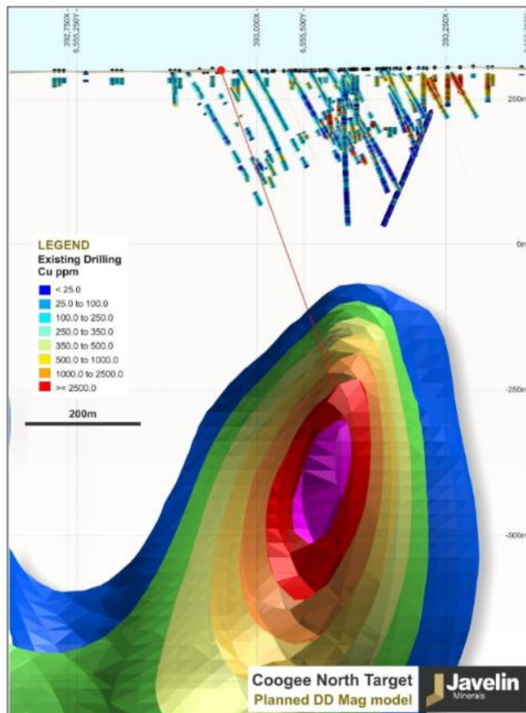
Figure 5 – Coogee North cross-section view of magnetic inversion model and existing Cu assay data from historic and recent drilling, highlighting the planned EIS diamond drillhole to test the modelled magnetic body
