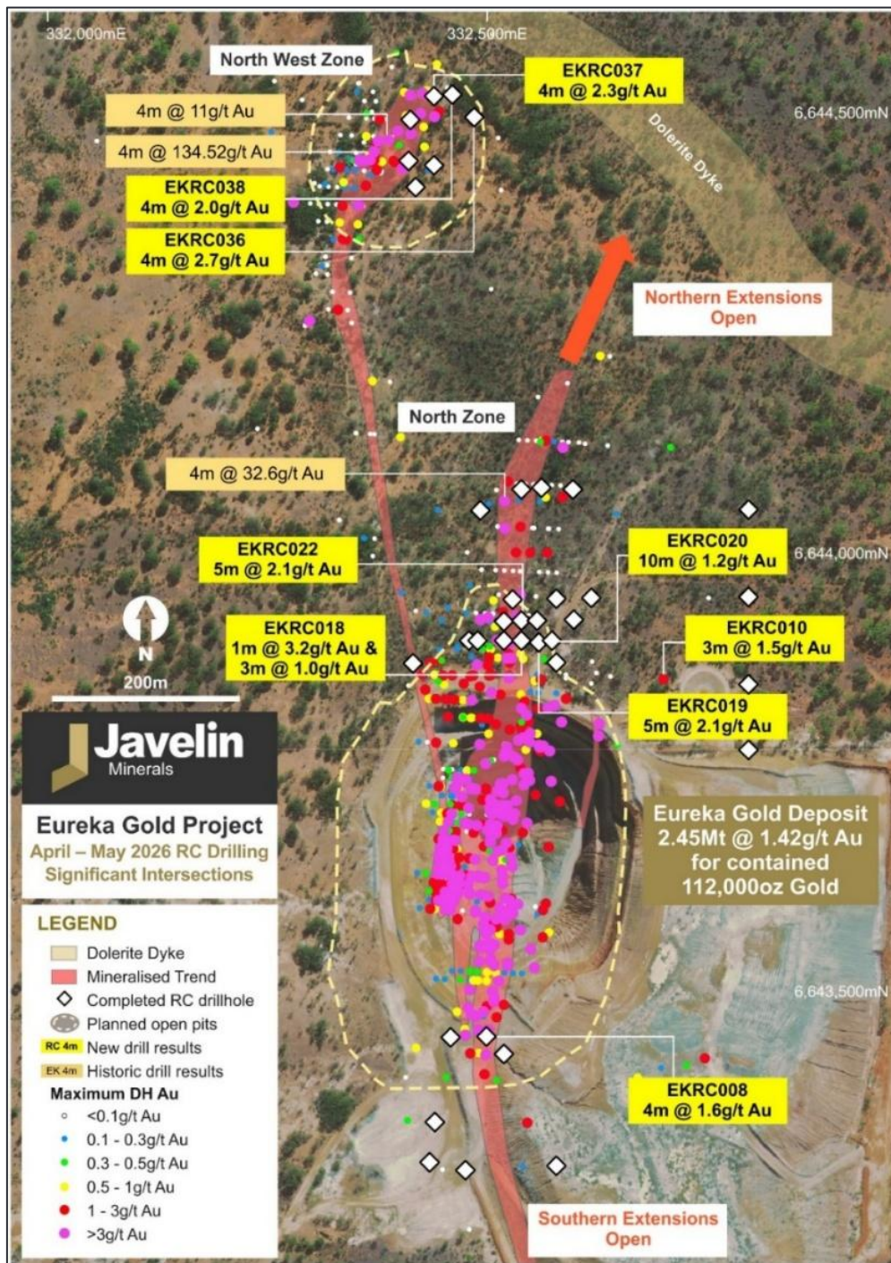
Figure 2 – Interpreted mineralised trends with significant intersections from Eureka RC drilling
