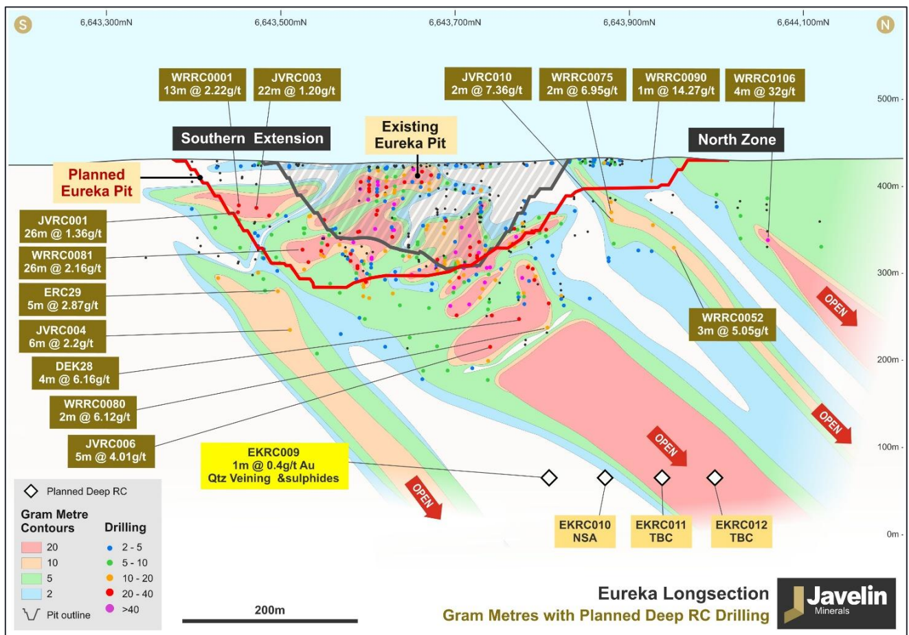
Figure 3 – Long-section (looking west) with high-grade intersections at depth and planned open pit cutback, including EKRC011 and EKRC012 to be completed with diamond tails to test the potential extensions of the Eureka orebody at depth
