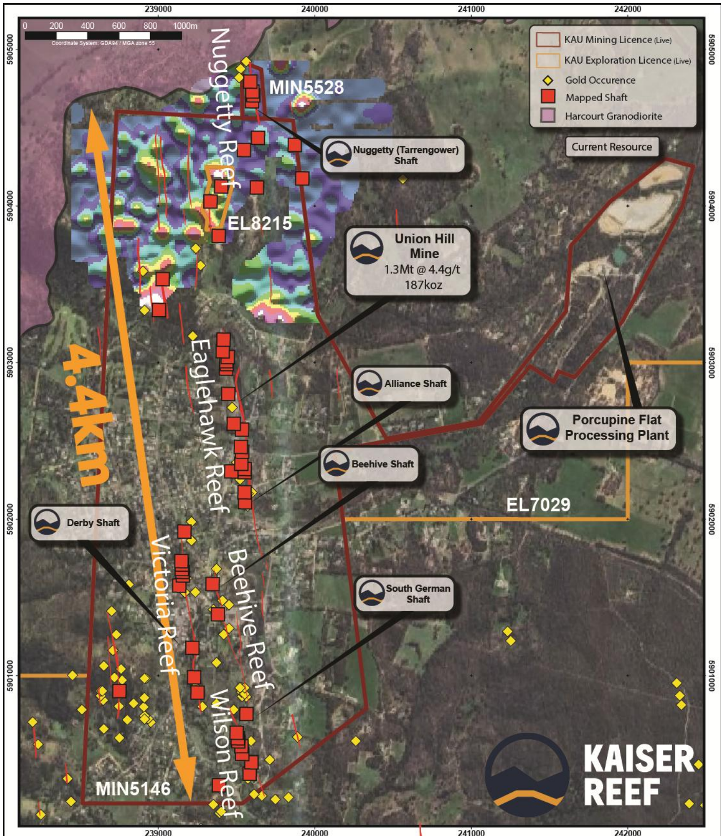
Figure 6. Soil sample gold results. Gridded soil sample percentile (99/98/95/90/80/60/30) Au results with mapped quartz veins and shafts over the Maldon Gold Project.
