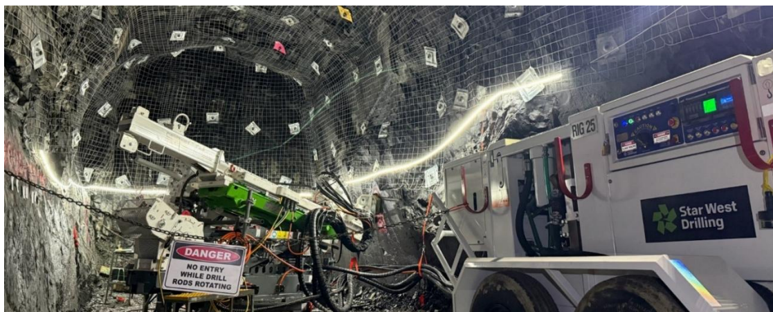
Figure 2. Drill rig at the face, Northern Drill Drive
