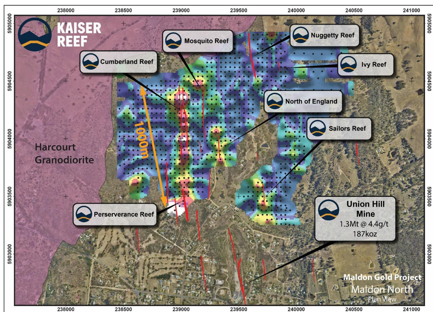
Figure 5. Soil sample arsenic results gridded by percentile (99/98/95/90/80/60/30) with mapped quartz veins and shafts.
