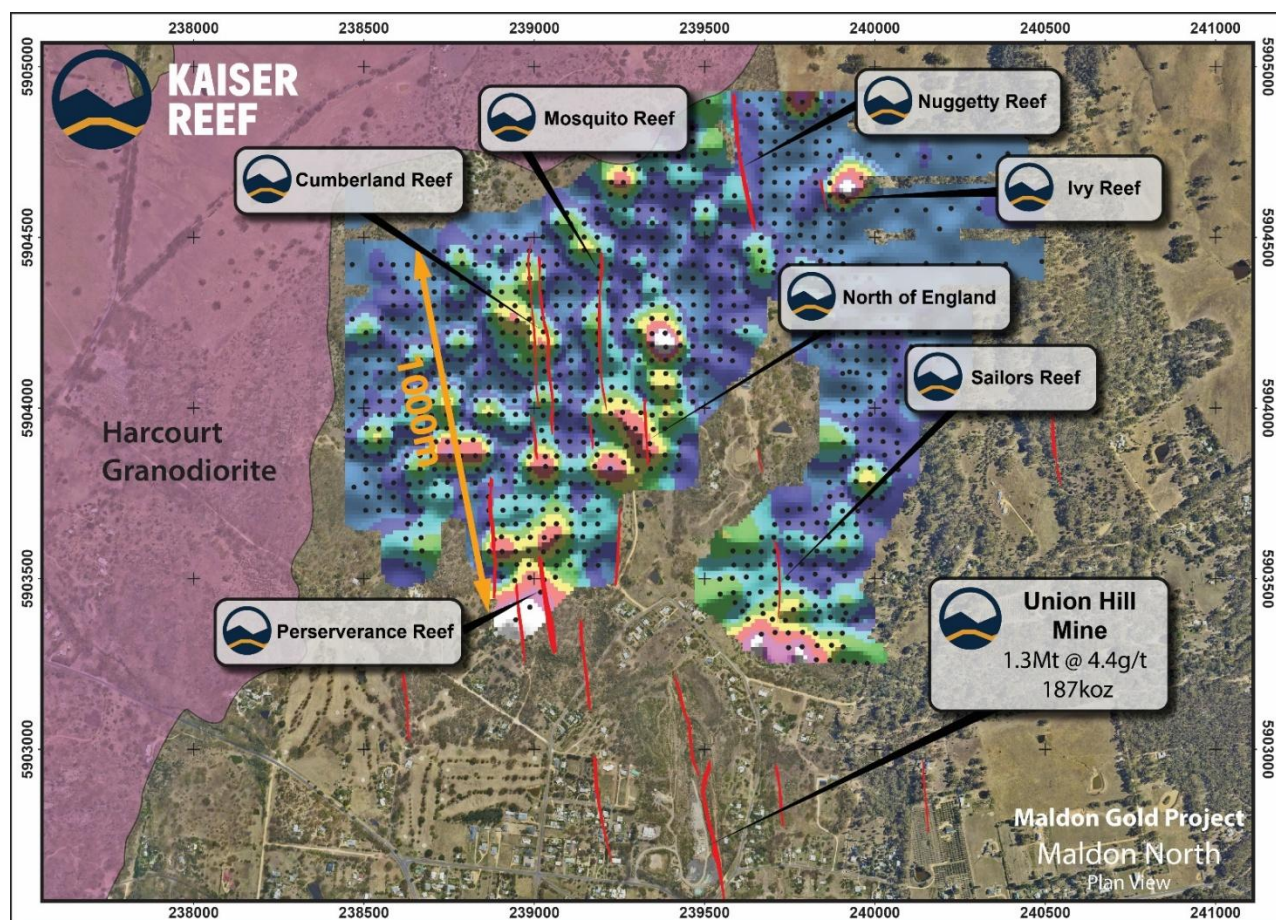
Figure 4. Soil sample gold results gridded by percentile (99/98/95/90/80/60/30) with mapped quartz veins and shafts.
