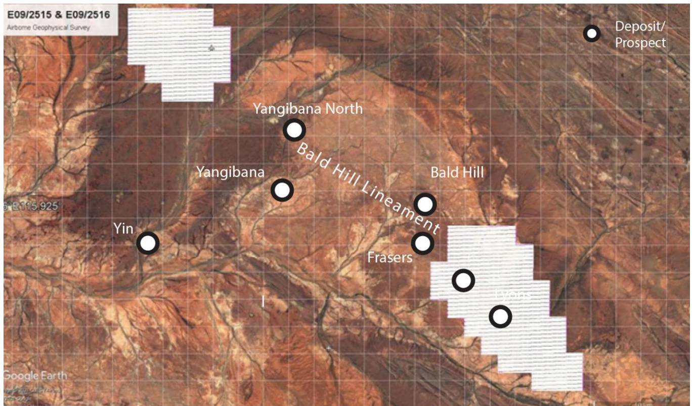
Figure 13. Magnetic-Radiometric Geophysical survey area, with planned 50m flight line spacing with a sensor height of 30m.
