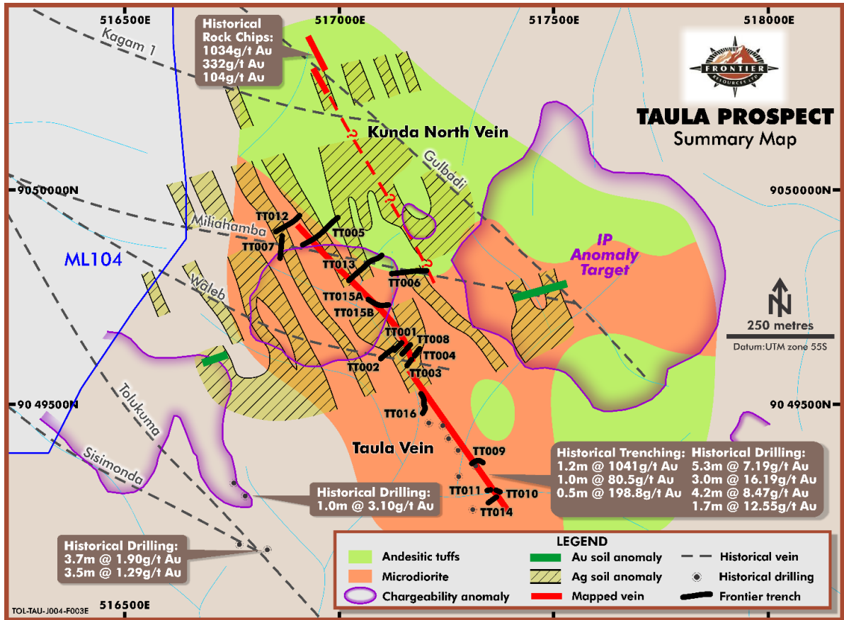
Figure 20: Taula Prospect Geology and Trench Sampling Locations.
