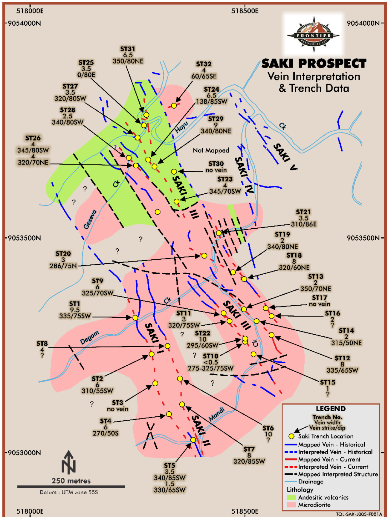
Figure 18: Saki Geology and Vein Orientation Map.
