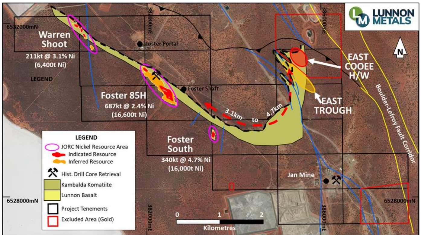
Figure 3 : Plan of the Kambalda Nickel Project detailing location of East Cooee – H/W and East Trough
