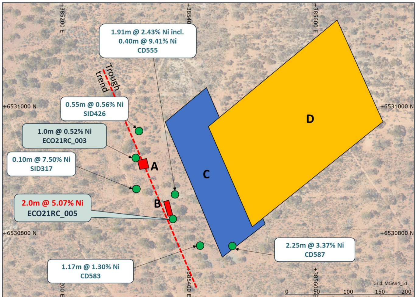
Figure 2 : Representation of DHTEM plates surrounding 2m @ 5.07% Ni in ECO21RC_005 – see ASX announcements dated 27 th July & 28 th September 2021 for additional details of holes annotated.
