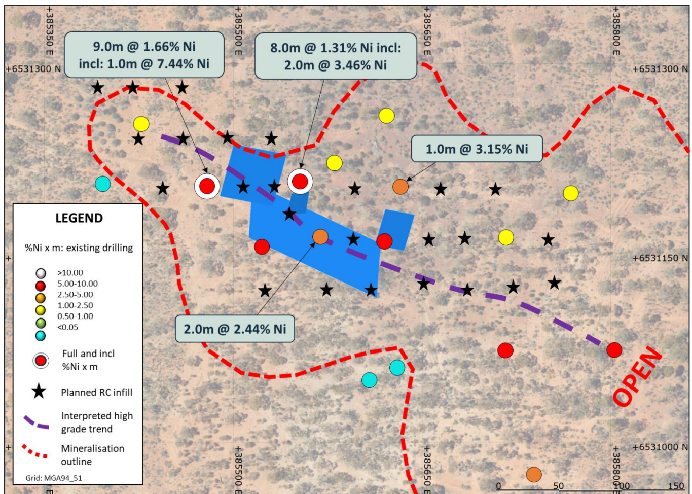
Figure 1 : Plan of East Cooee area illustrating pierce points of upcoming RC infill drill holes, previous drilling 2 to date and re-modelled DHTEM plates (blue rectangles)
