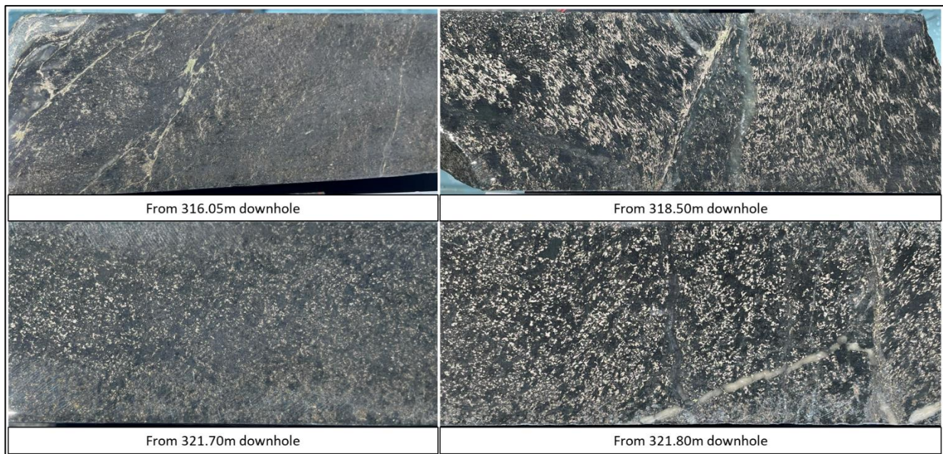
Figure 2: Photo-mosaic - visual observations: nickel sulphides in FOS21DD_003 – images show from downhole depth – for scale core width 50mm
