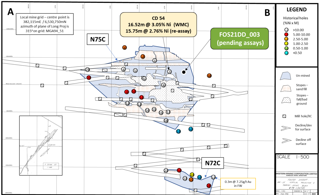
Figure 3 : Representation of WMC Resources Longitudinal Projection for the N75C & N72C nickel surfaces at the Foster Mine, KNP (looking north east) – see ASX announcement dated 26 th November 2021 for WMC drill hole details.
