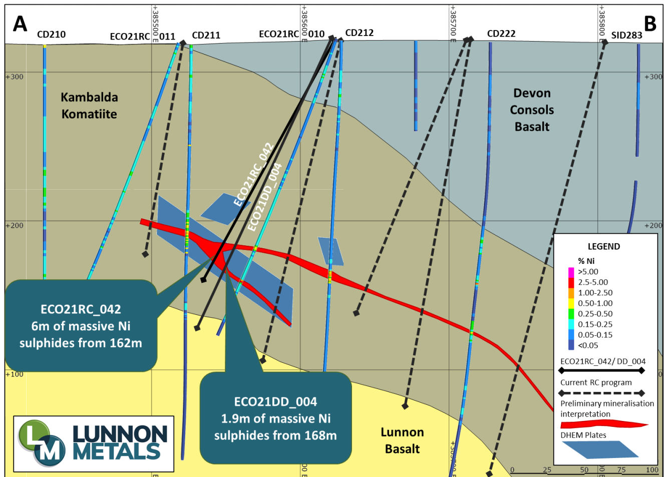
Figure 3 : Diagrammatic cross section A-B (6,531,160mN) through drill line hosting ECO21RC_042 and ECO21DD_004 diamond hole (looking north: Grid:MGA94_51)
