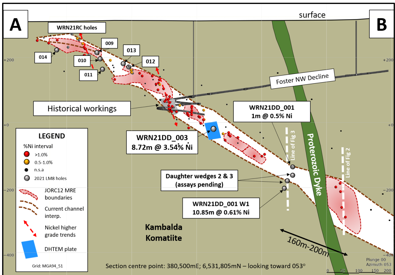
Figure 4: Long Projection of the Warren channel showing pierce points for WMC intercepts and the WRN21DD_001 daughter programme
