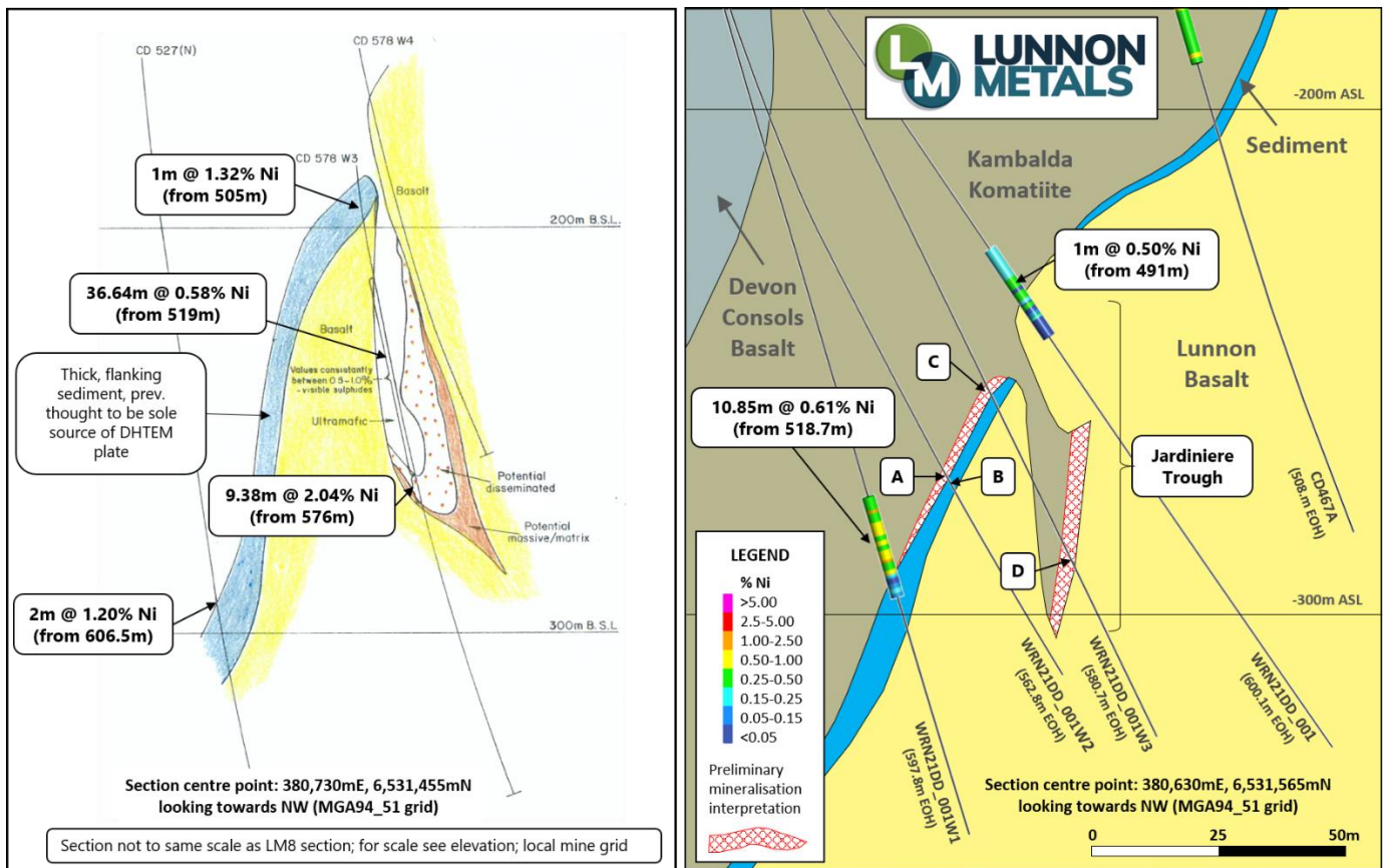
Figure 2 & 3: WMC's cross section through the Jardiniere Trough (left) and Lunnon Metals' current WRN21DD_001 daughter programme (right), see Tables 1 & 2 for descriptions of A, B, C and D visual intercepts.
