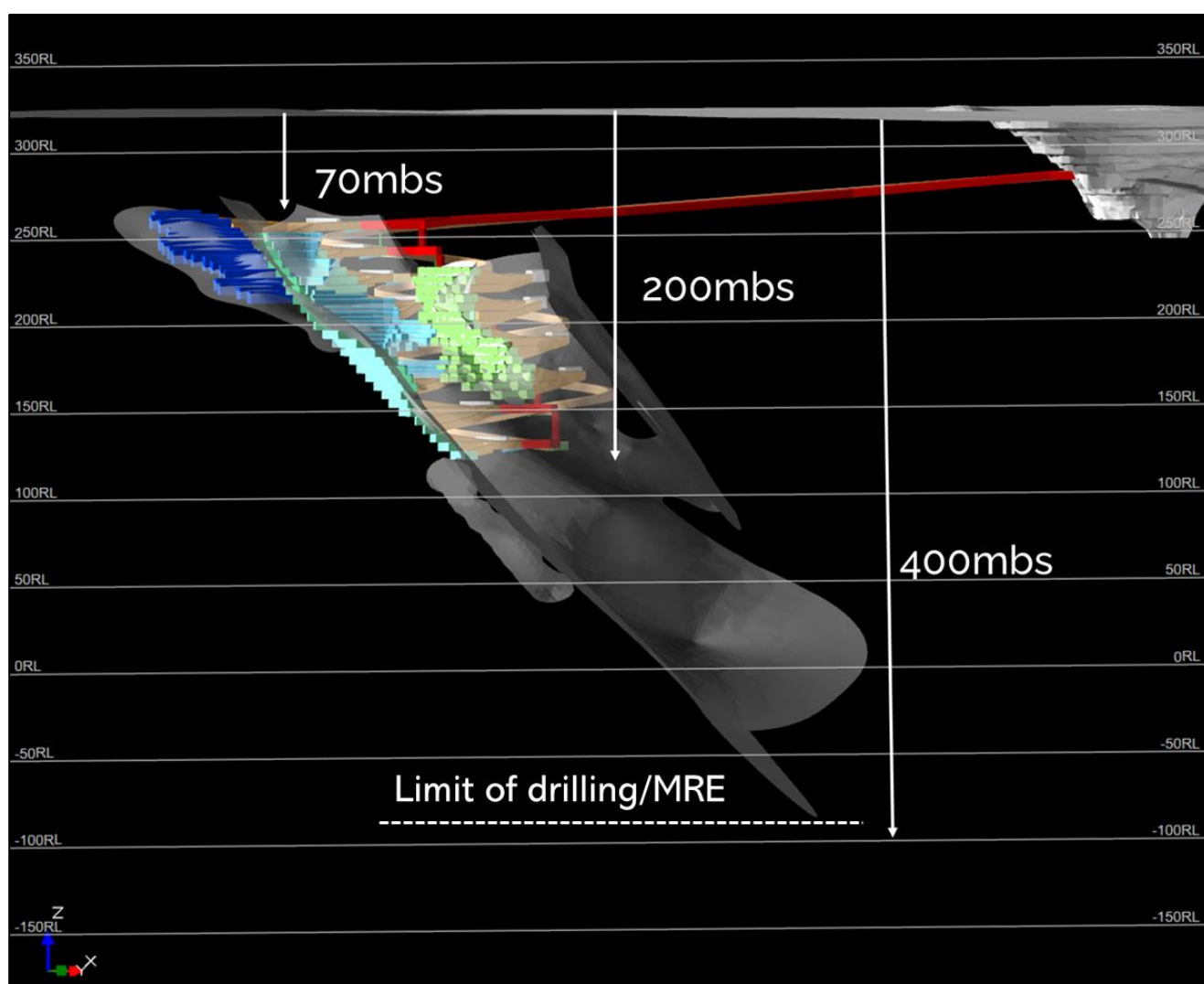
Figure 1: Isometric view of conceptual mine design for potential future Baker underground mine accessed from adjacent historical West Idough gold open pit (view looking north illustrating approximate depth below surface in metres - "mbs").
