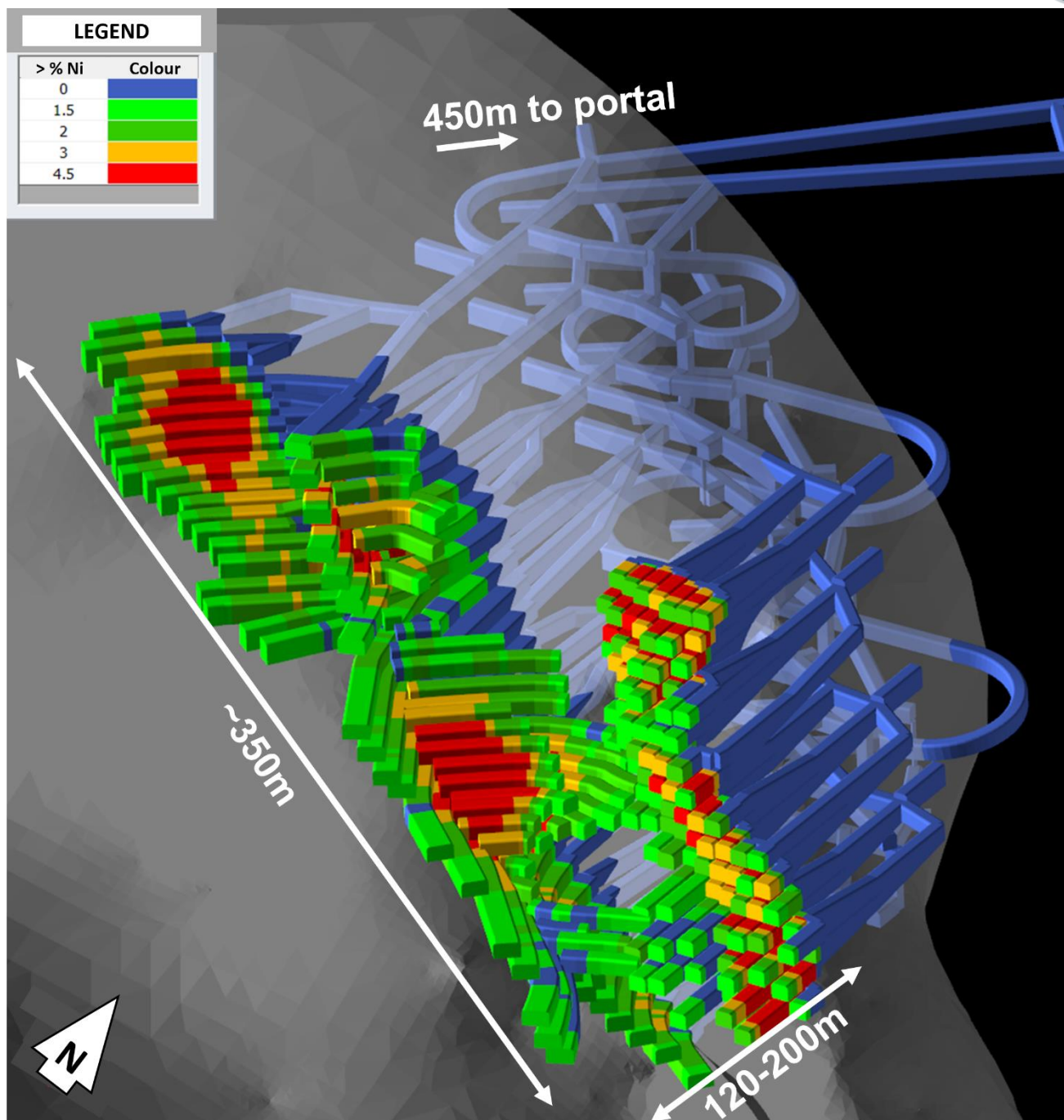
Figure 2: Isometric view of conceptual mine design for potential future Baker underground mine (view looking down to the north west coloured by diluted modelled nickel grade %).
