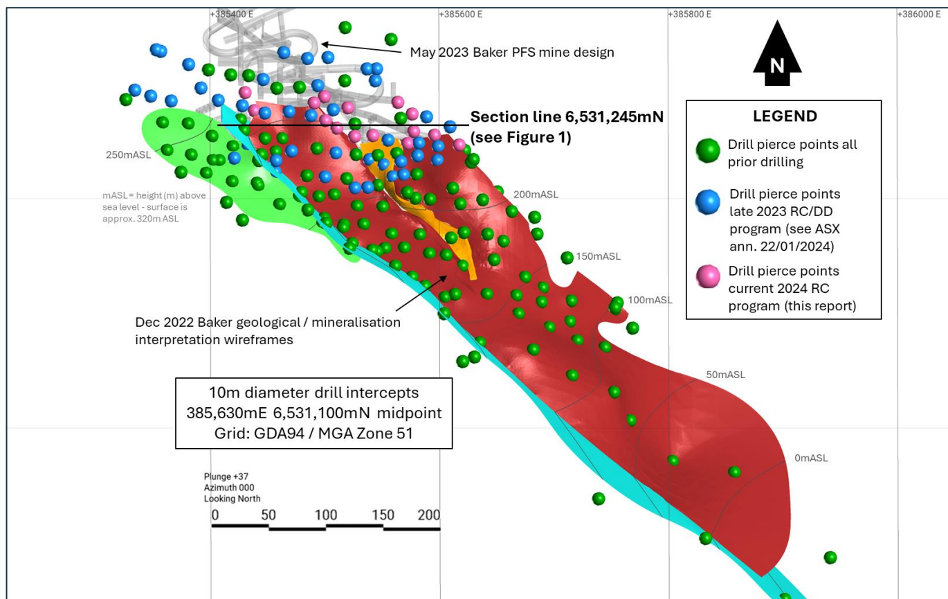
Figure 2: Isometric view (orthogonally down to the north) of the project to date Baker drilling pierce points represented by 10m diameter spheres (both DD and RC), highlighting the regular and close spaced drill pattern, together with this latest 2024 RC program.
