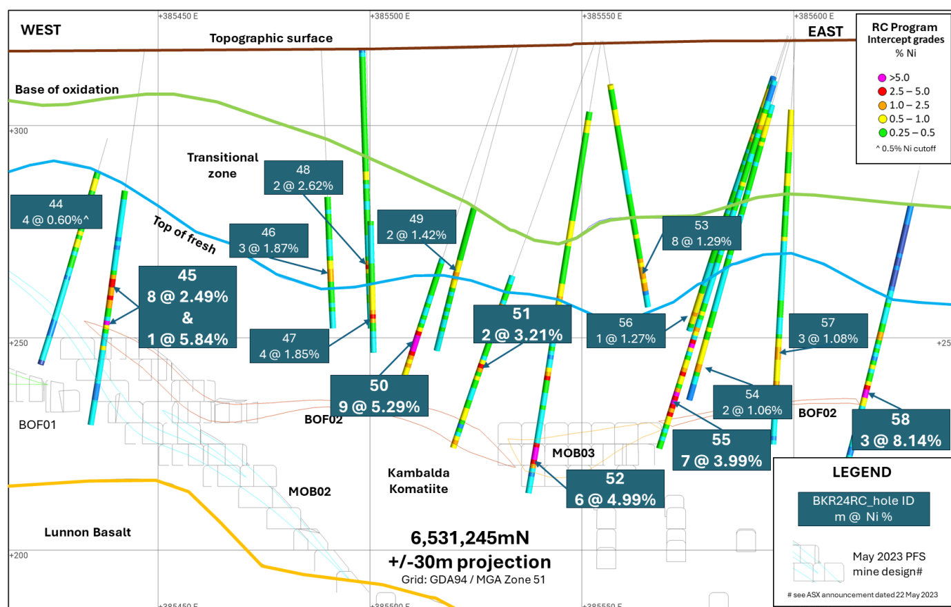
Figure 1: Cross section 6,531,245mN (looking north) through the Baker May 2023 MRE domains (BOF01, MOB02 etc), the current mine design and the latest 2024 RC drill program results.
