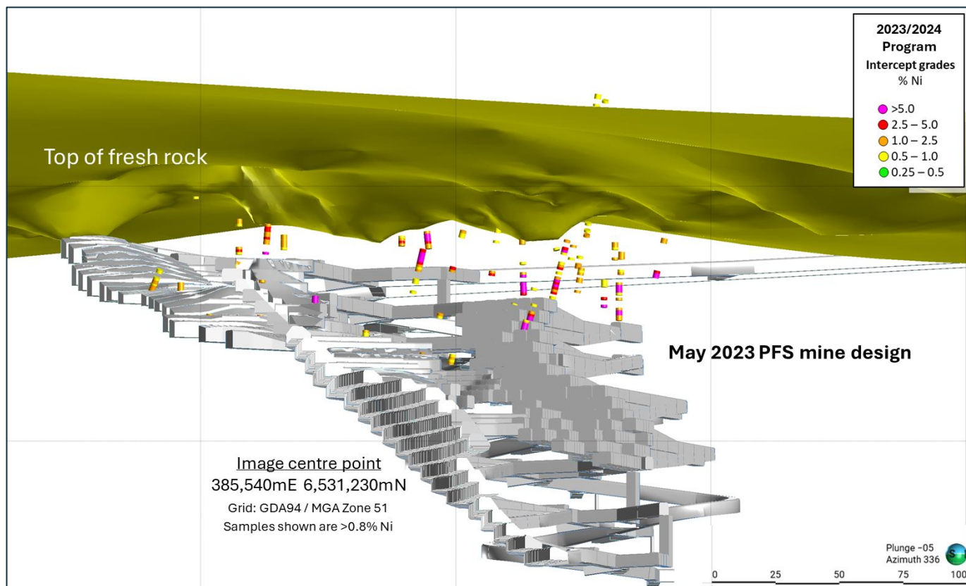
Figure 3: Isometric view (looking north-west) of the previously reported 2023 RC/DD and the latest 2024 RC program intercepts shown relative to and outside the existing May 2023 PFS mine design (the basis for the current Ore Reserve at Baker) and below the top of fresh rock (yellow wireframe).
