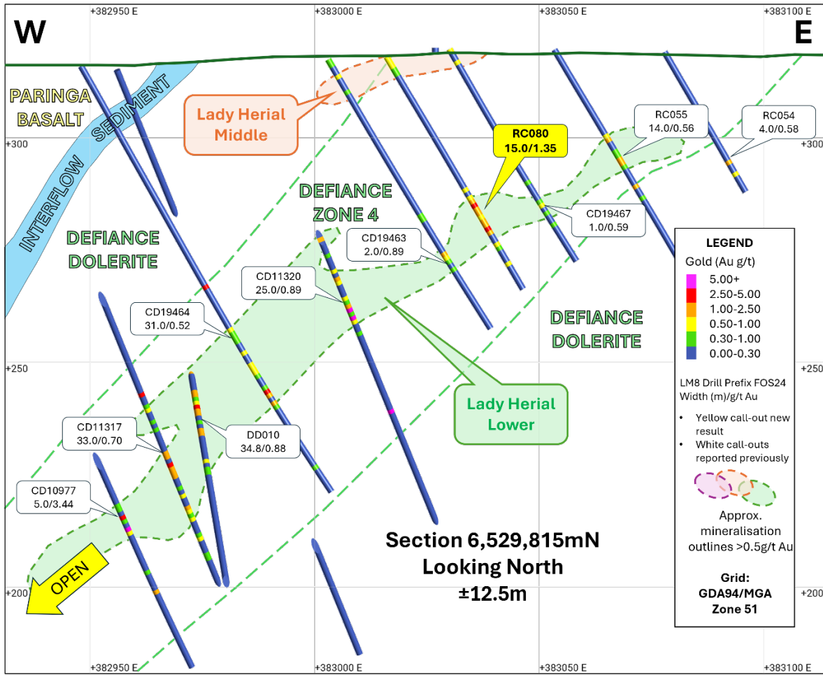
Figure 3: Cross section 6,529,815mN through the Lower Structure and the thicker than expected intercept in FOS24RC_080.
