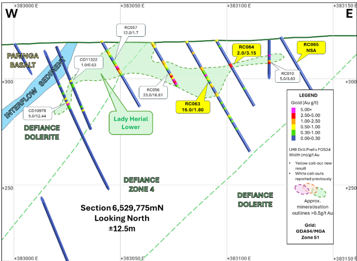
Figure 4: Cross section 6,529,775mN highlighting the Lower Structure at Lady Herial and additional mineralisation in its footwall.
