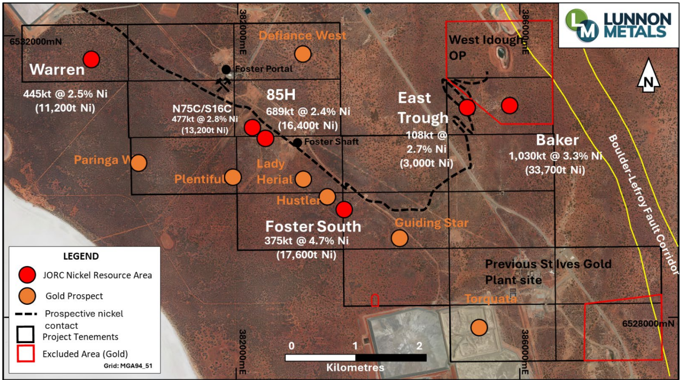
Figure 7: Foster-Baker Project Area showing nickel Mineral Resource 5 positions and select gold prospects.
