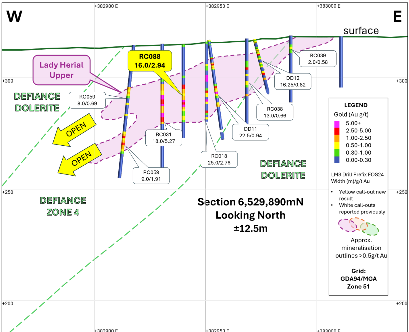
Figure 2: Cross section 6,529,890mN through the Upper Structure illustrating location of FOS24RC_088.
