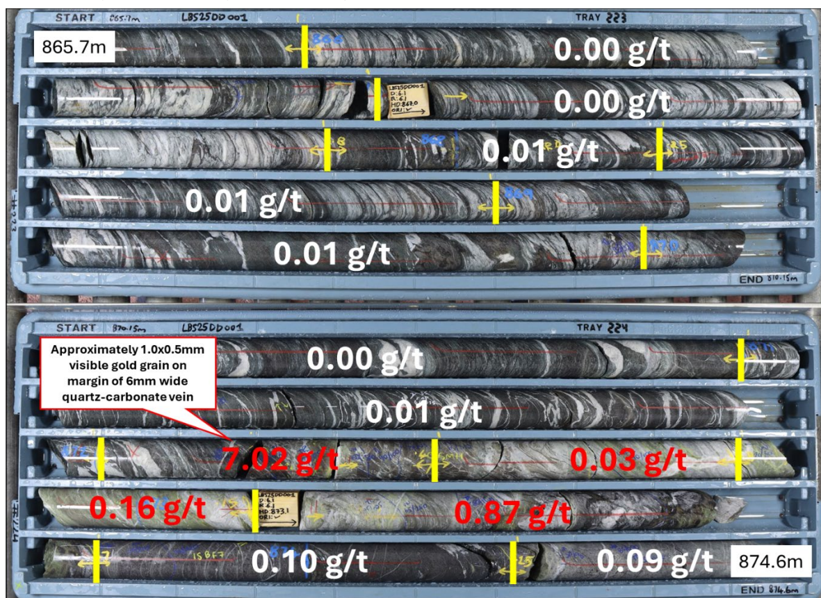
Figure 4. LBS25DD_001 drill core from 865.7m to 874.6m annotated with individual sample gold assay results (g/t Au) through the lower Foster Thrust hosted gold structure. The yellow lines demarcate individual samples. Each core tray is approximately 1 metre in length.
