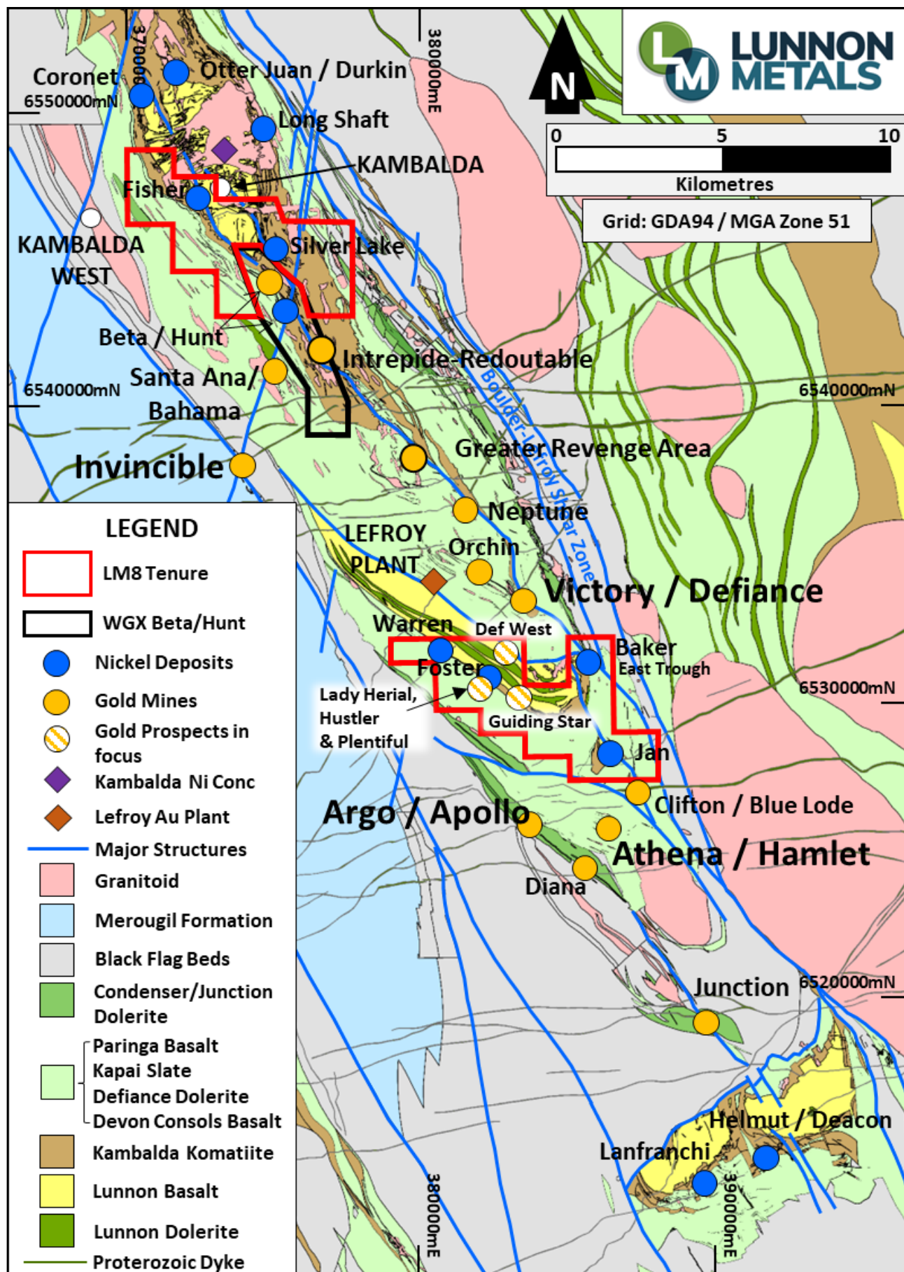
Figure 8: The KGNP (red outlines) with Kambalda / St Ives regional geology and location of key nickel and gold mines/infrastructure.
