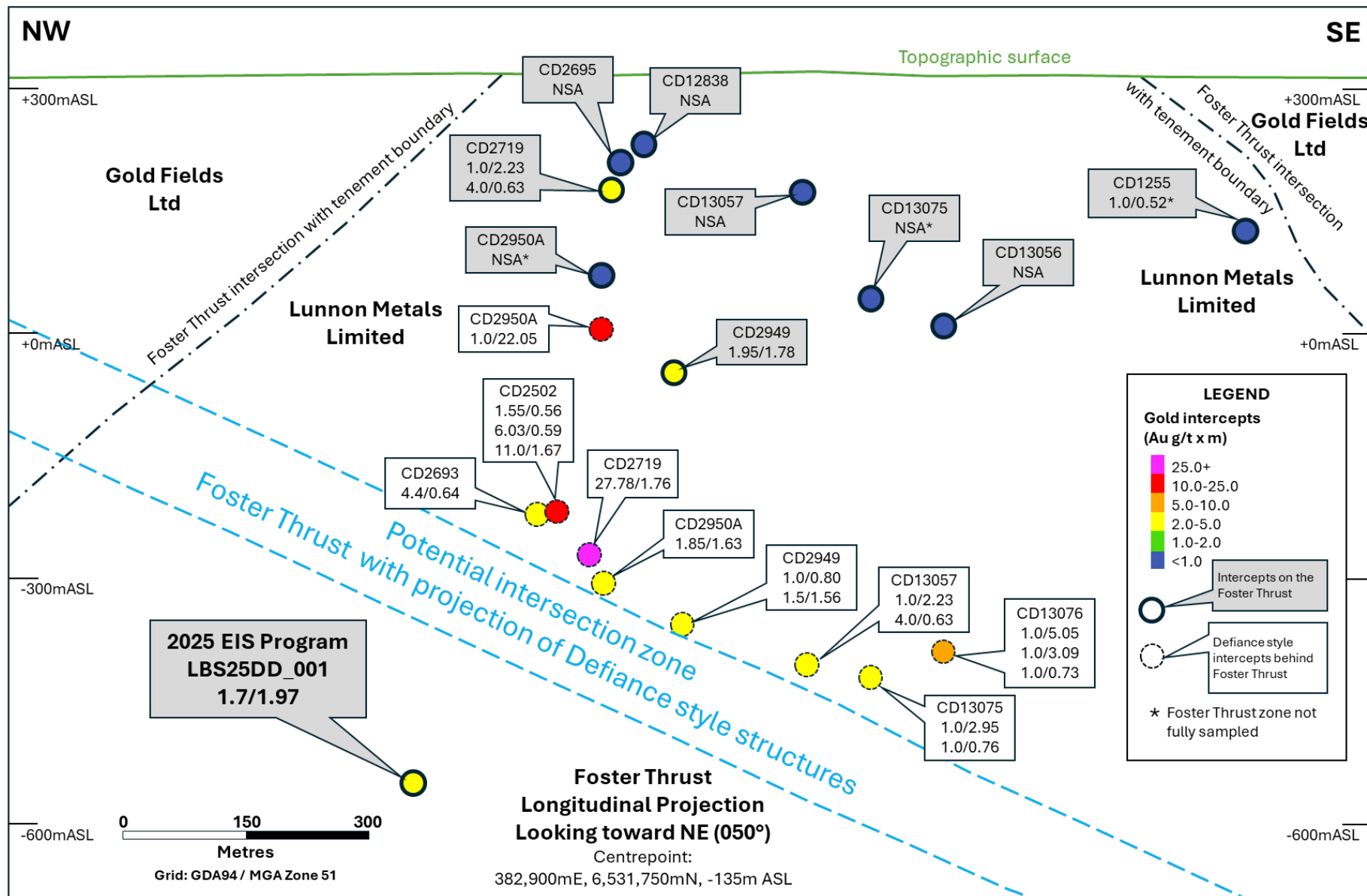
Figure 6. Longitudinal projection of the Foster Thrust (looking NE) showing drilling pierce points on the thrust (bold circles) with Defiance style structure intercepts located further to the NE behind the thrust projected onto the image (dashed circles).
