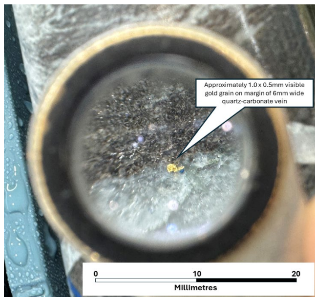
Figure 1: Gold bearing quartz-carbonate vein in drill core at approximately 872.2m downhole showing the magnified 1.0x0.5mm gold grain within 0.4m which assayed 7.02g/t Au.
