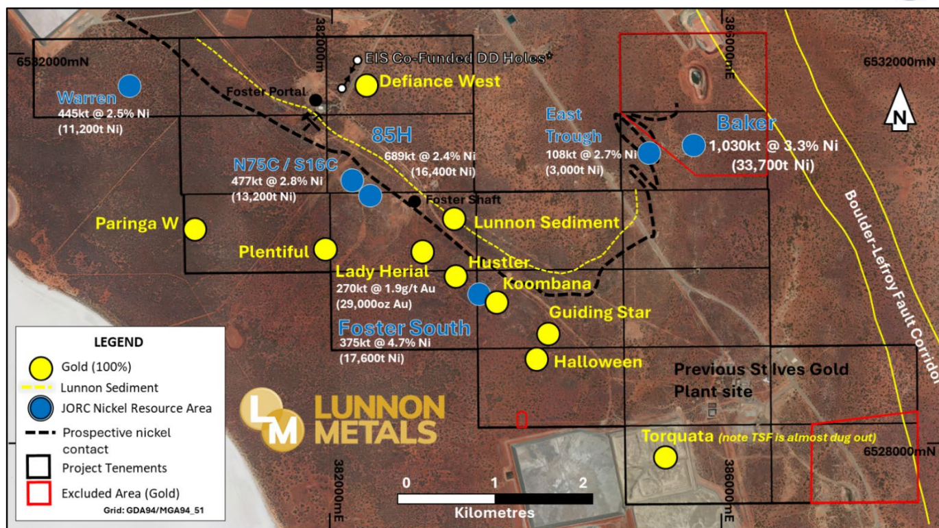
Figure 7: Foster-Baker Project Area showing select high-ranking gold prospects, collar locations of EIS DD Holes (*subject to change based on progress/outcomes) plus gold & nickel Mineral Resource 5 positions.
