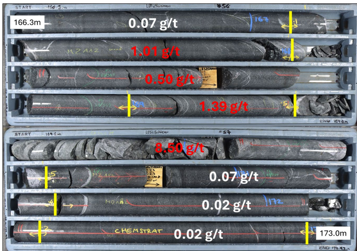
Figure 3. LBS25DD_001 drill core from 166.3m to 173.0m annotated with individual sample gold assay results (g/t Au) through the upper dolerite hosted gold structure. The yellow lines demarcate individual samples. Each core tray is approximately 1 metre in length.
