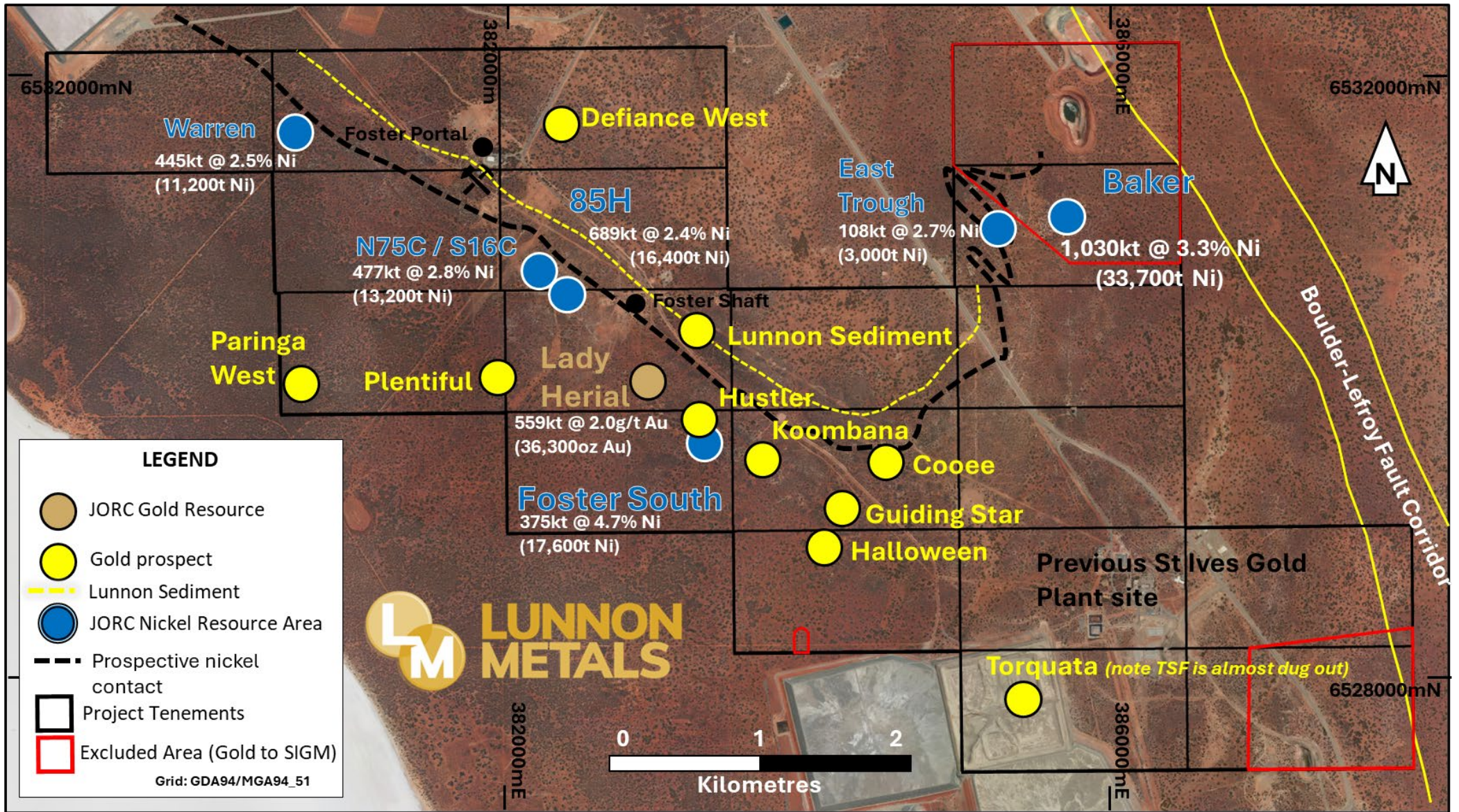
Figure 7: Foster-Baker Project Area showing select high-ranking gold prospects, gold & nickel Mineral Resource 5 positions.
