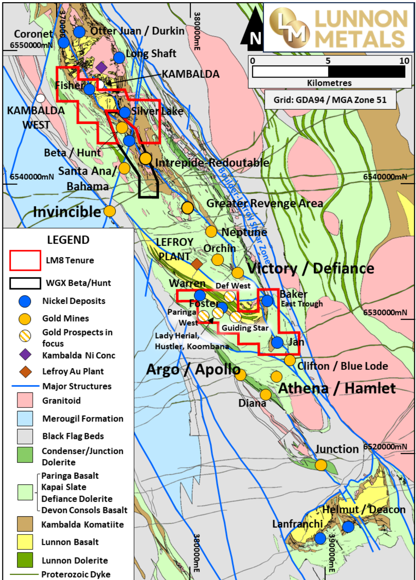
Figure 8: Location of the KGNP (red outlines) at the local Kambalda/St Ives scale; showing surface geology and structure of this significant Australian gold camp.
