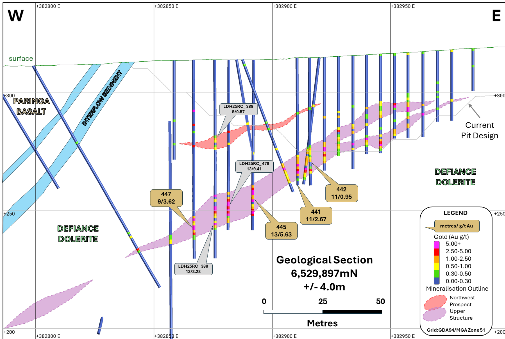
Figure 5: Section 6,529,897mN (looking north +/- 4m) illustrating the Upper Structure results reported today (gold call-outs) and select prior reported results (grey call-outs).
