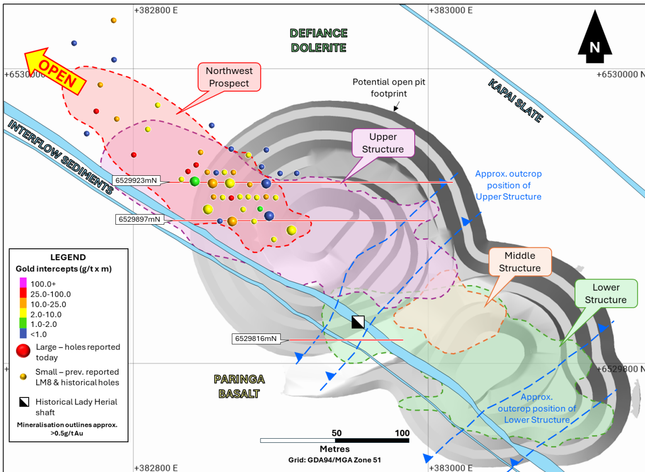
Figure 3: Plan view of the Lady Herial open pit development area illustrating the NWP results reported today (larger spheres) and prior reported results (smaller spheres) under the northwest wall of the planned pit.
