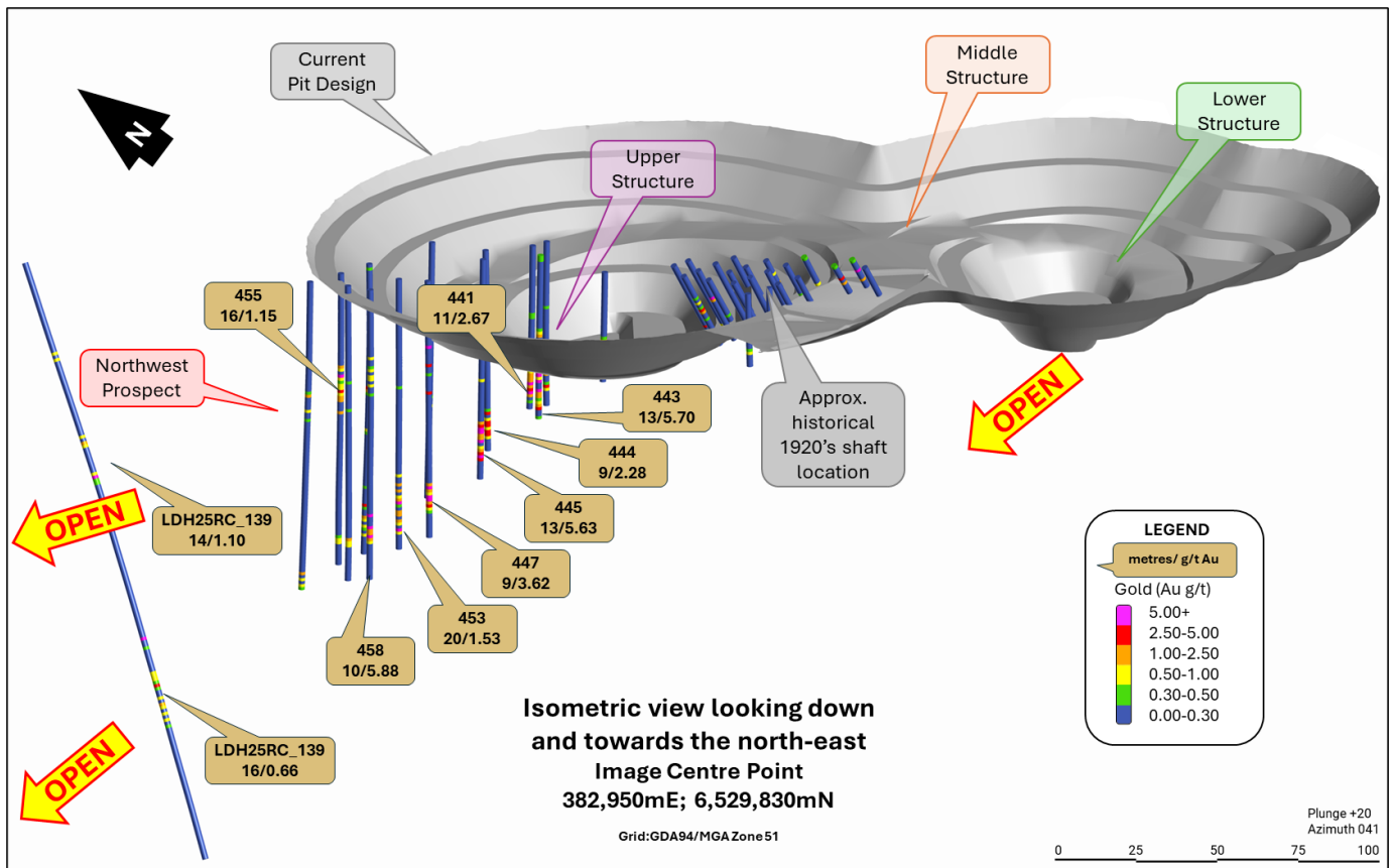
Figure 1: Isometric view of the Lady Herial open pit development area illustrating the results reported today and the opportunity that remains open down plunge on the NWP and the Upper Structure.
