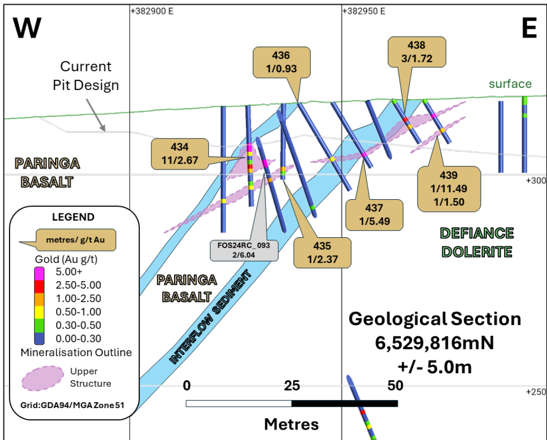
Figure 6: Section 6,529,816mN (looking north +/- 5m) illustrating the Sediment results reported today (gold call-outs) and select prior reported result (grey call-out).
