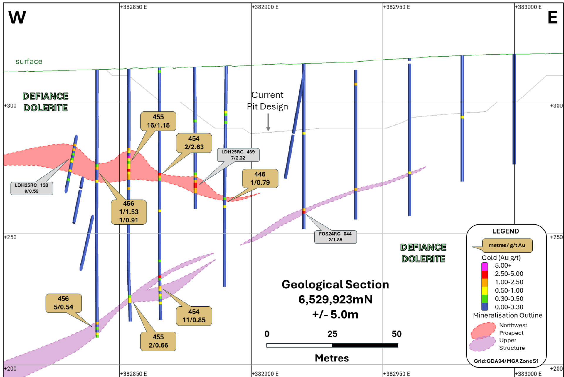
Figure 4: Section 6,529,923mN (looking north +/- 5m) illustrating the NWP results reported today (gold call-outs) and select prior reported results (grey call-outs).
