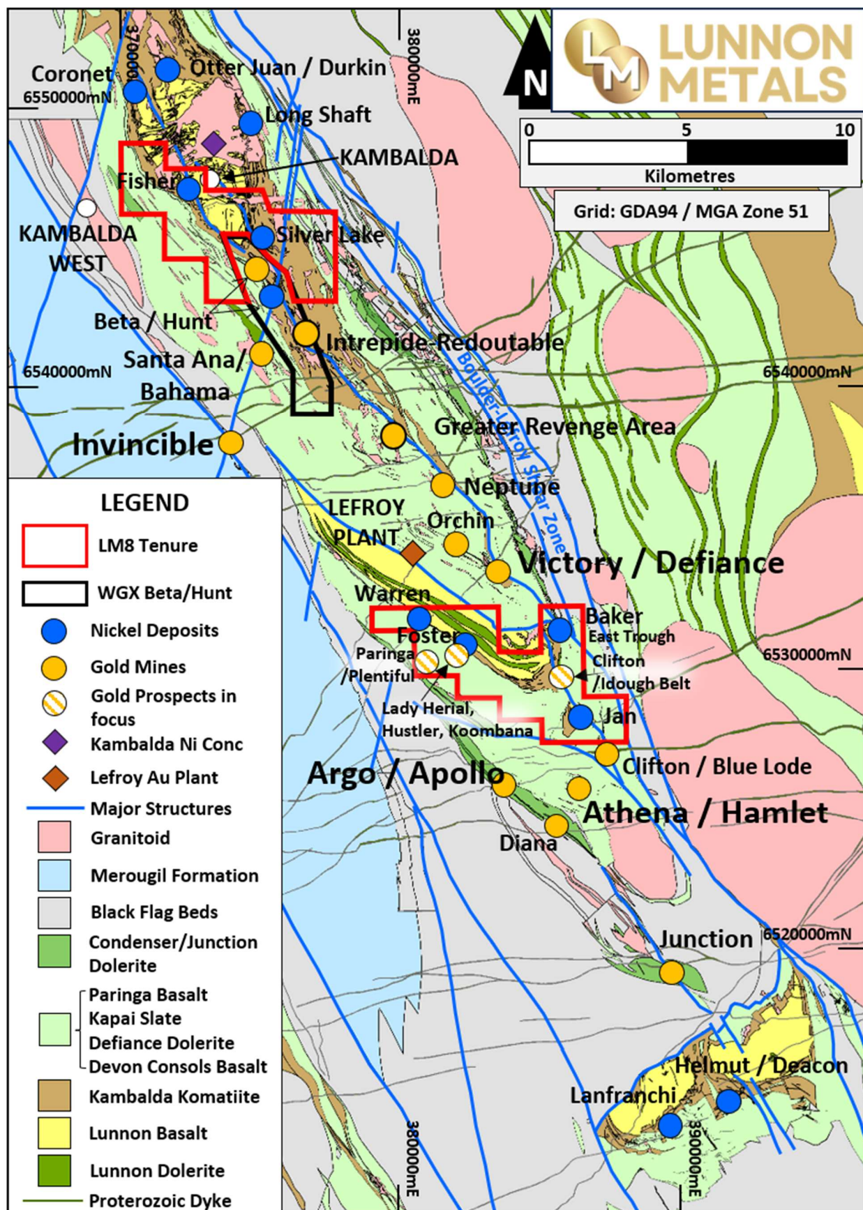
Figure 1: Location of the KGNP (red outlines) at the local Kambalda/St Ives scale; showing surface geology and structure of this significant Australian gold camp and location of the Kambalda Nickel Concentrator.
