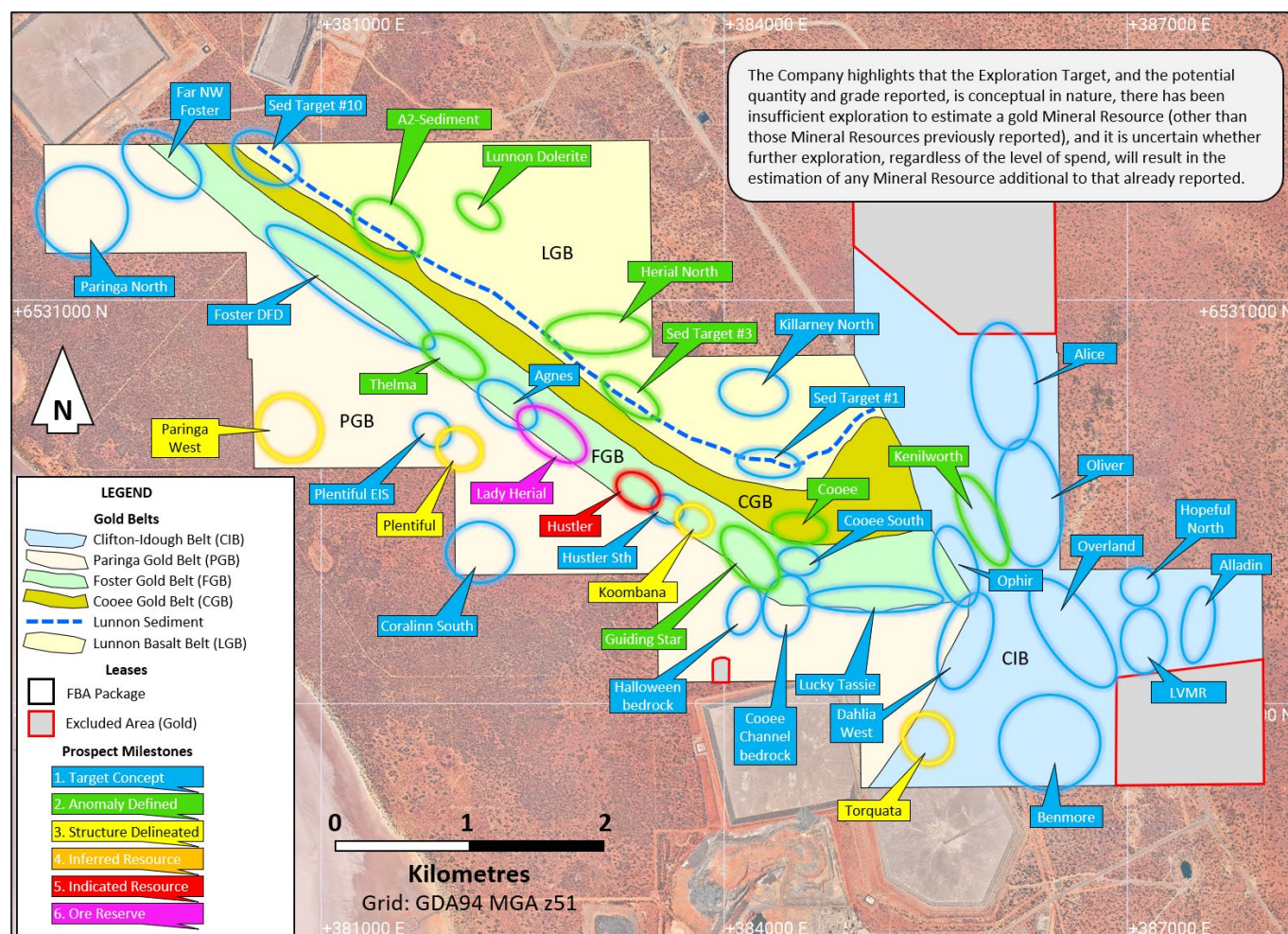
Figure 7: Plan view of the FBA showing the interpreted gold belts hosting the current portfolio of high-quality gold targets, ranging in maturity from Conceptual to Resource Definition.
