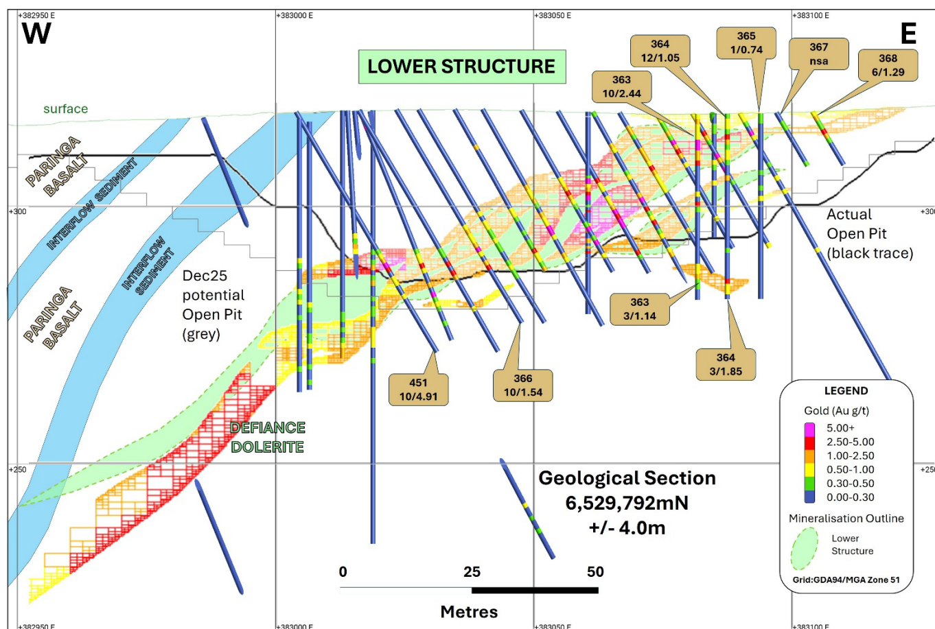
Figure 5: Cross section 6,529,792mN: current Mineral Resource (Feb'26) model draped over section as lodged on 11 Dec 2025 and both actual and prior conceptual pit outlines (see ASX announcement dated 11 Dec 2025 for details of any drill holes represented).
