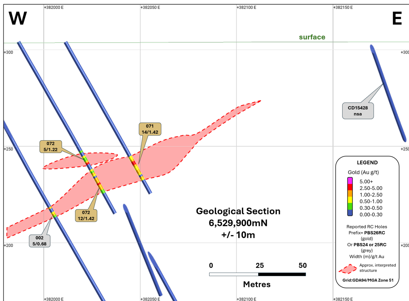
Figure 9: Cross section 6,529,900mN through the Quarter's and previous Plentiful RC results.
