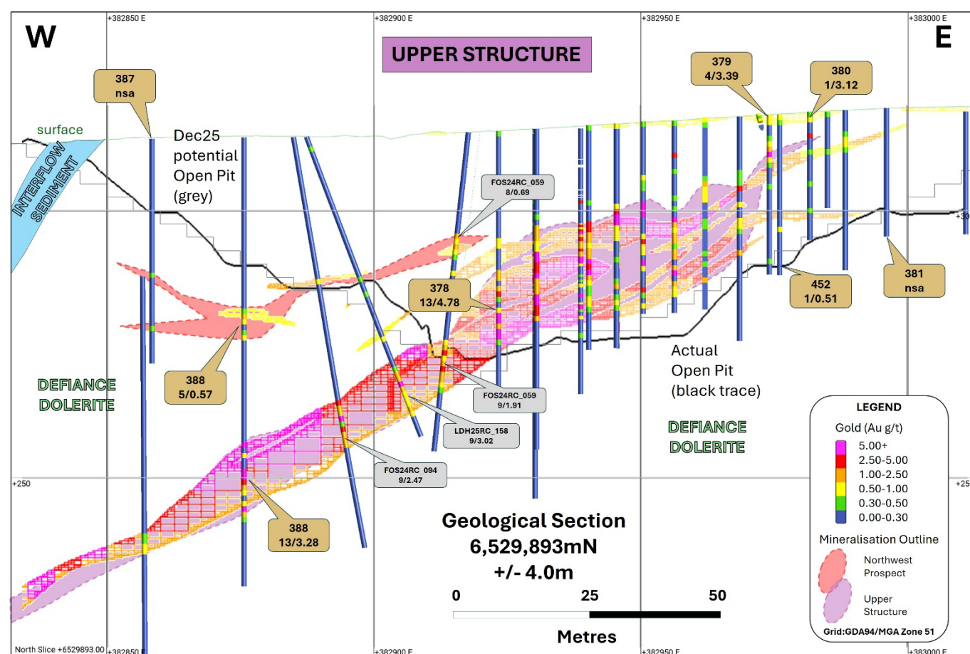
Figure 4: Cross section 6,529,893mN: current Mineral Resource (Feb'26) model draped over section as lodged on 11 Dec 2025 and both actual and prior conceptual pit outlines (see ASX announcement dated 11 Dec 2025 for details of any drill holes represented).
