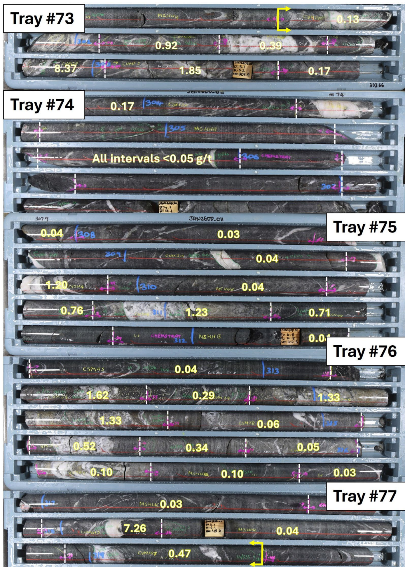
Figure 12: DD core trays from JAN26DD_011 showing sheared, foliated biotite altered mafic rock with zones of albite-pyrite rich breccias and veins. Sampled intervals are shown with the relevant returned assays in g/t Au.
