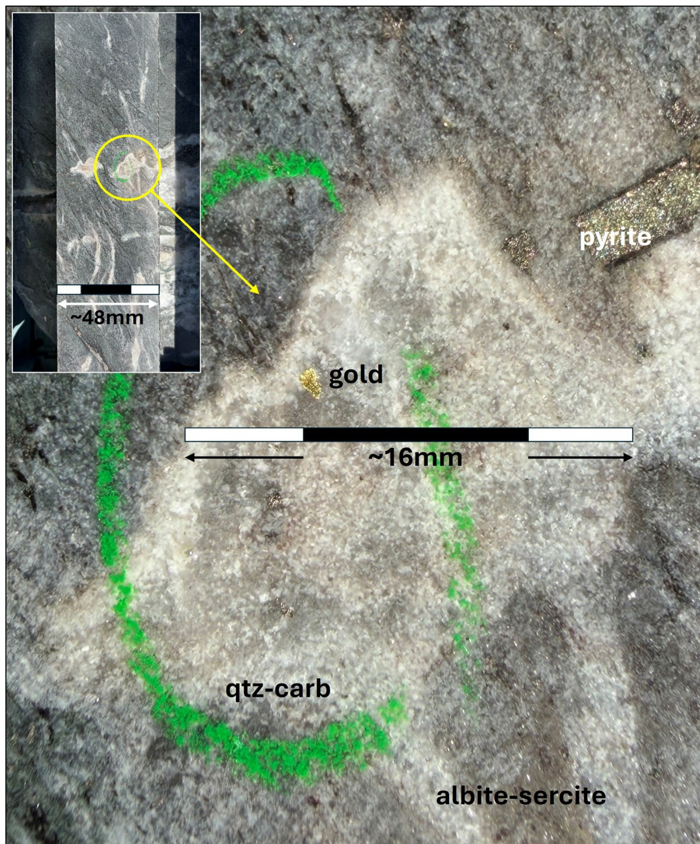
Figure 13: Zoomed image of DD core at 302.25m from JAN26DD_011, illustrating observed visible gold in an interval that assayed only 0.92 g/t Au.
