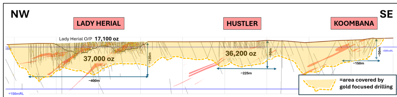
Figure 8: Diagrammatic long section looking north-east showing relative location of Hustler, Koombana and Lady Herial, with current MRE 3 gold ounces and the amount of gold that mining depleted from the last reported Lady Herial MRE (shown directly above the open pit outline).
