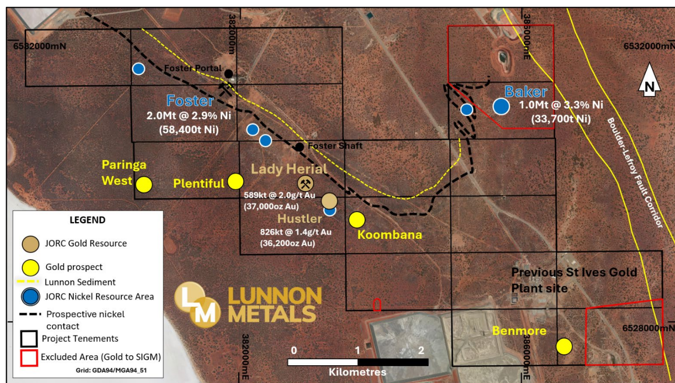
Figure 3: FBA Project showing Lady Herial mine, gold & nickel Mineral Resource 7 positions and select high-ranking gold prospects.
