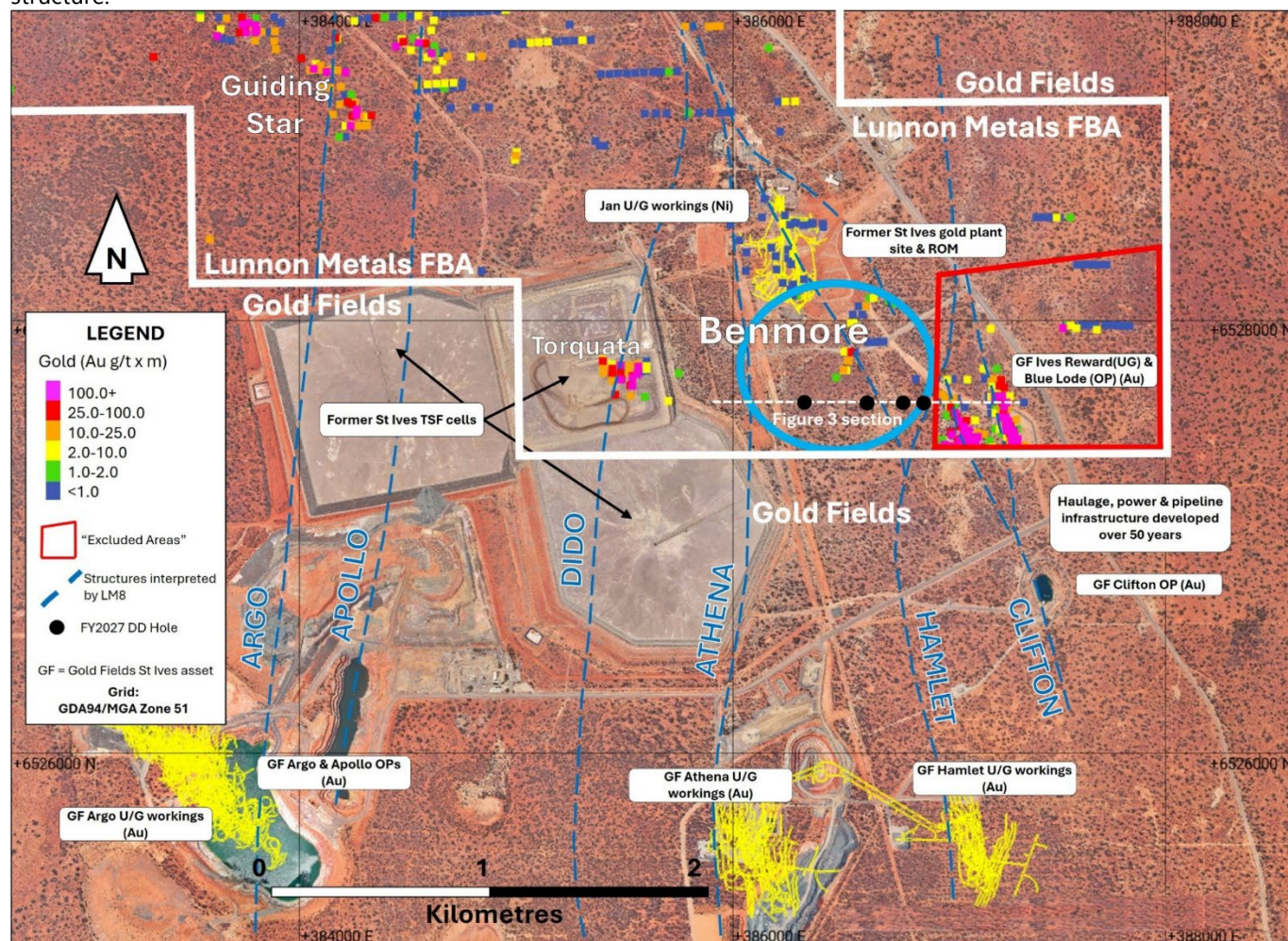
Figure 11: Plan view of the Benmore target area showing the location of the DD transect, the Jan underground nickel mine and the nearby underground gold mines on Gold Fields' leases to the south.
