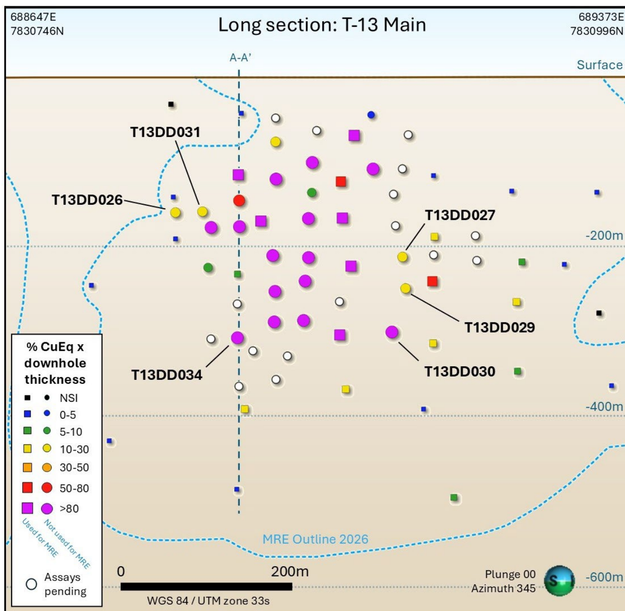
Figure 1: Simplified long section of T-13 Deposit.
