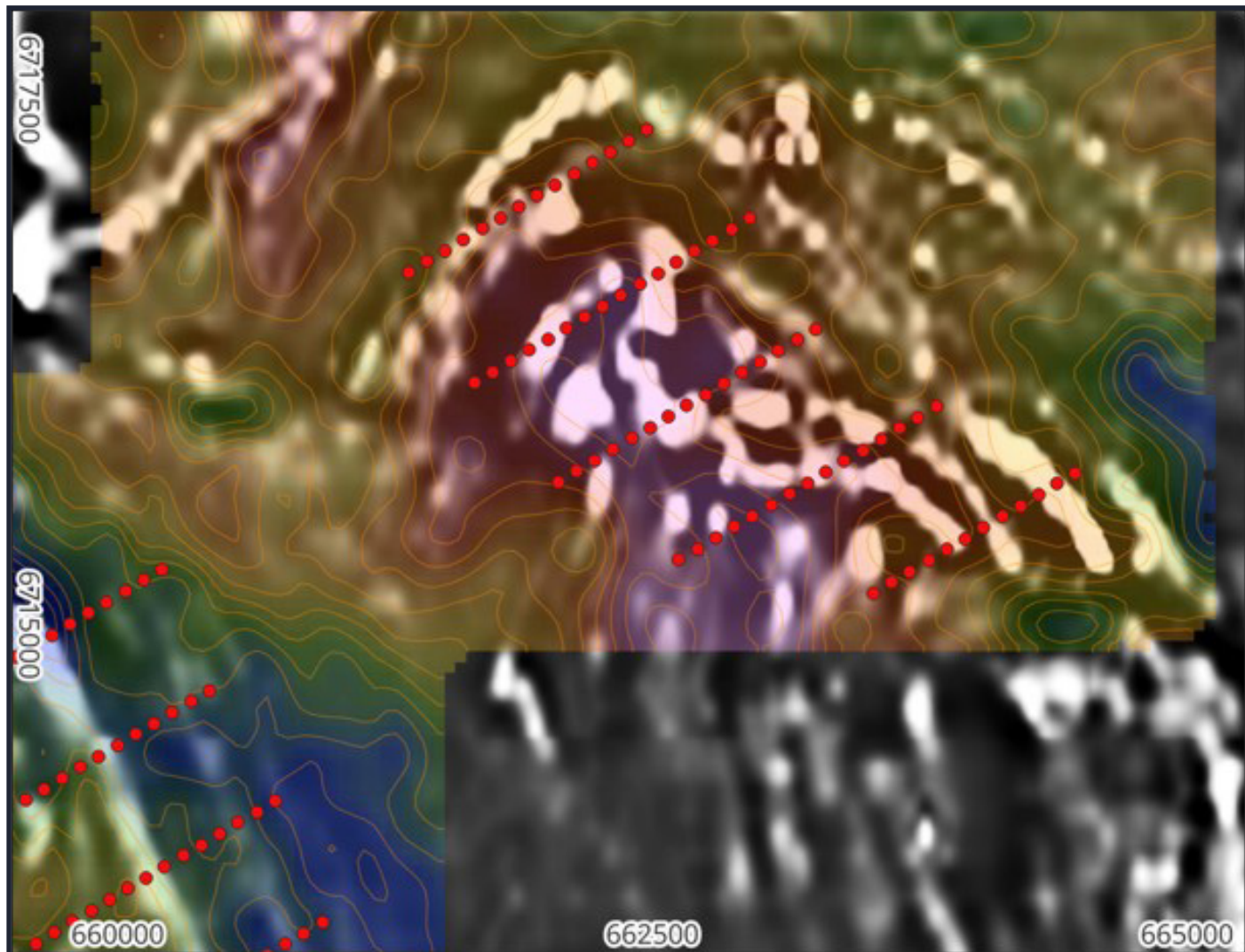
Figure 3: Masson NE planned MLEM stations at 100 x 600m, overlaid onto semi-transparent Bouguer Anomaly Second Residual with contours, and the RTP 1VD.
