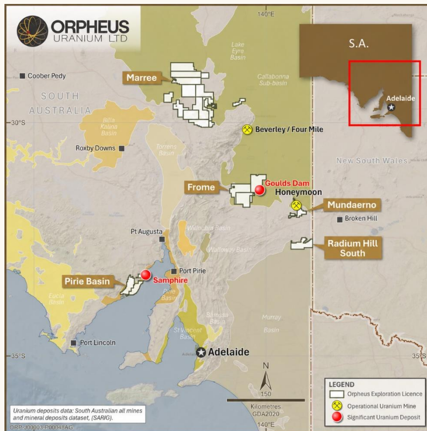
Figure 2: Orpheus Uranium's South Australian project locations relative to South Australia's known resources. includes the incoming Marree tenure from Adavale (ASX: ADD).
