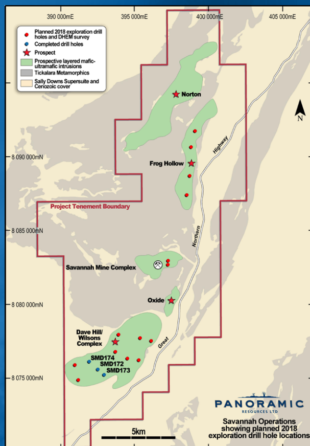
Figure 3 – Savannah Project Plan showing location of prospective mafic-ultramafic intrusions and planned 2018 drill holes.
