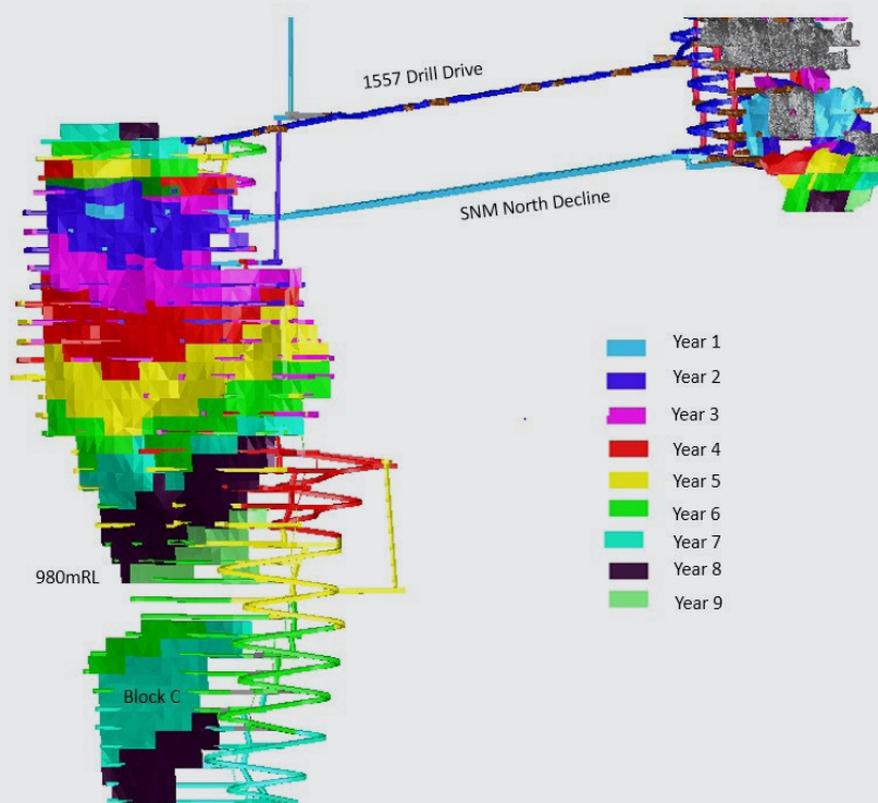
Figure 2. Savannah Project Simplified Mine Plan
