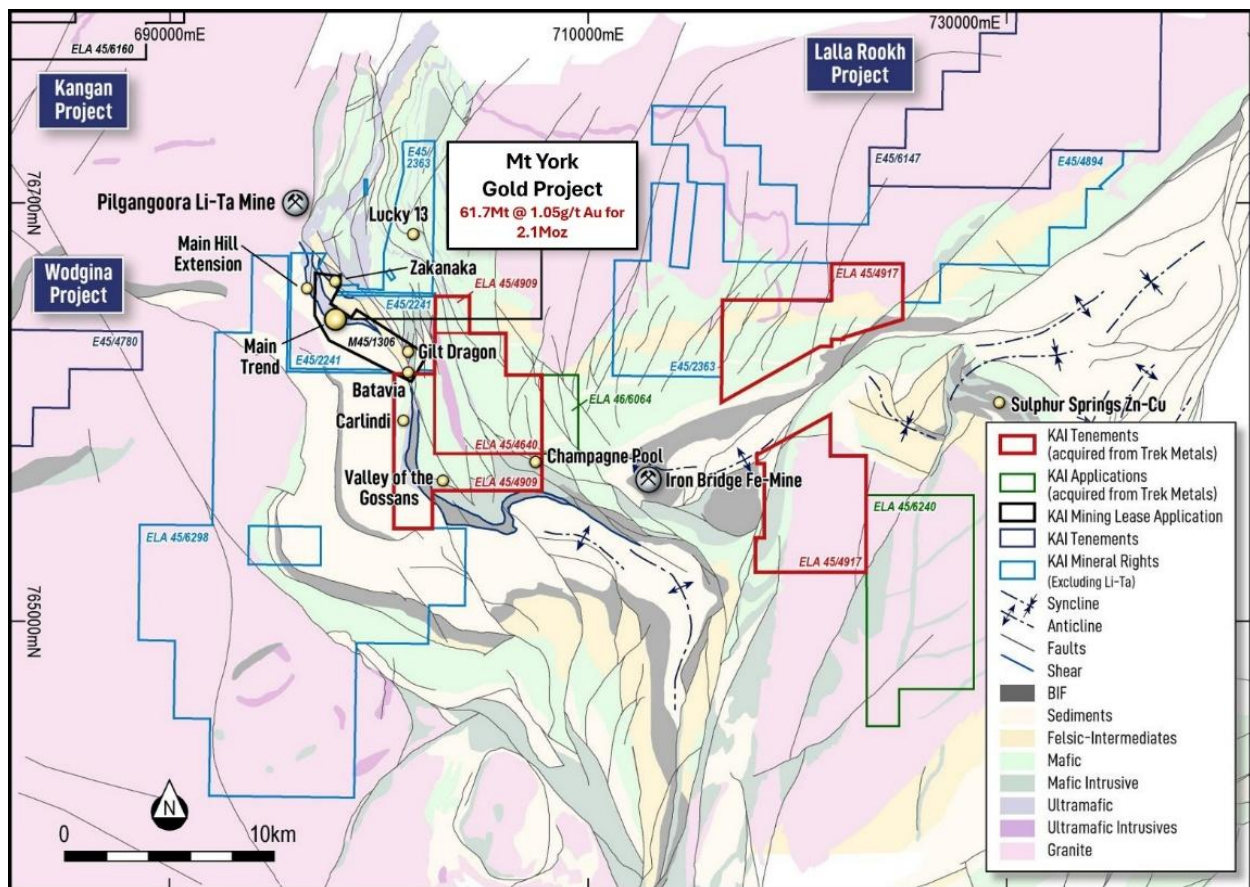
Figure 1. Exploration Licences and applications subject of the MRA (blue licences) surrounding PGL's Mt York Gold Project.
