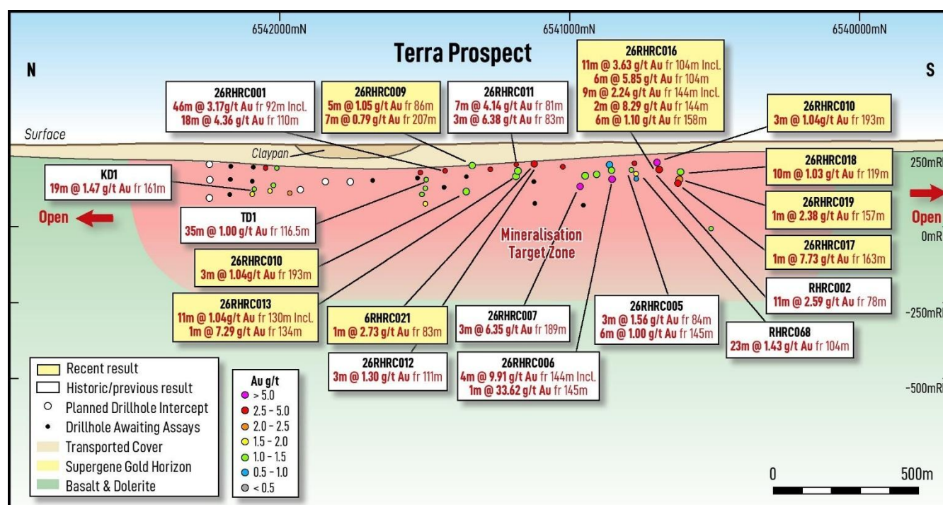
Figure 3. Long-section view of Terra Prospect looking east showing all drill results past (white boxes) and present (yellow boxes) over the >1,500m strike length. Drillhole intercepts are coloured by Au grade and are reporting downhole lengths. 2026 planned drill holes shown as white circles. 2026 drilling results are outlined and show the high degree of lateral continuity that is being defined from North (left) to South (right) of the prospect. See Figure 4 for a plan view. The image includes results reported on 13 October 2026 in ASX announcement entitled 'Further high-grade gold results expand mineralisation at Terra Prospect, Roe Hills'
