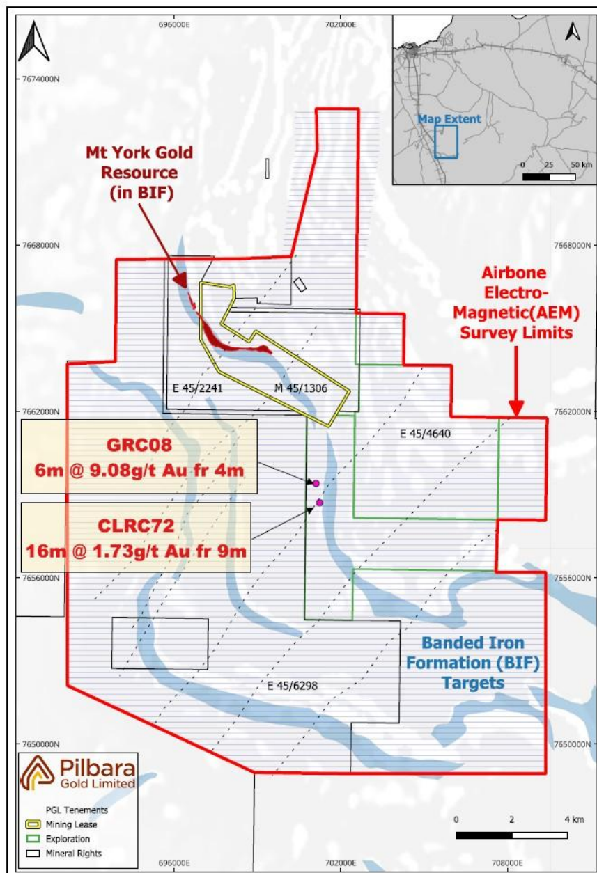
Figure 2. AEM survey area in relation to the position of the Mt York Project resource and interpreted banded iron formations. Historic results shown from the Carlindi trend.
