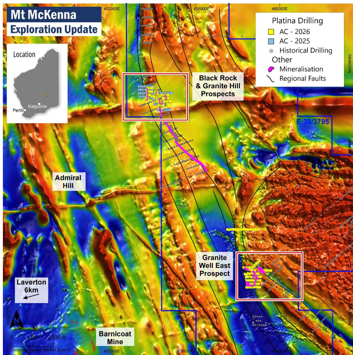
Figure 4. Map showing historical drilling and Platina's aircore drilling on Mt McKenna's E38/3795 tenement. Red boxes indicate areas of aircore drilling focus and observed mineralised corridors are shown in pink. Map underlain by the Geological Survey of Western Australia's (GSWA) reprocessed and Platina's newly acquired merged TMIRTP 1VD magnetic image by Core Geophysics.
