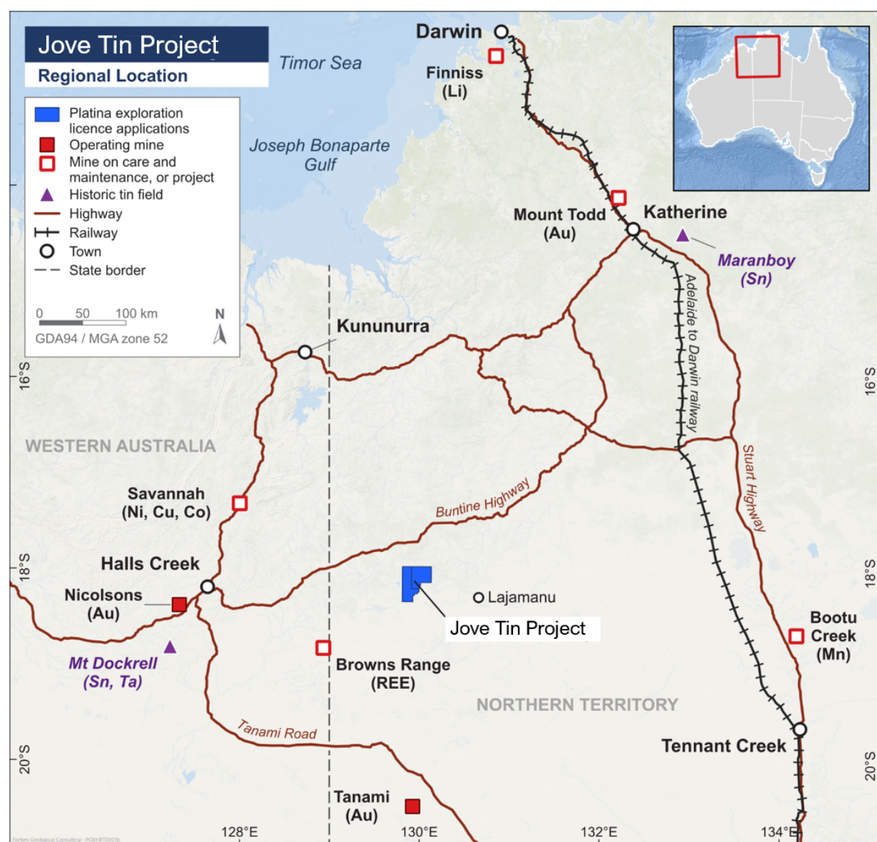
Figure 6. Location of the Jove Project.
