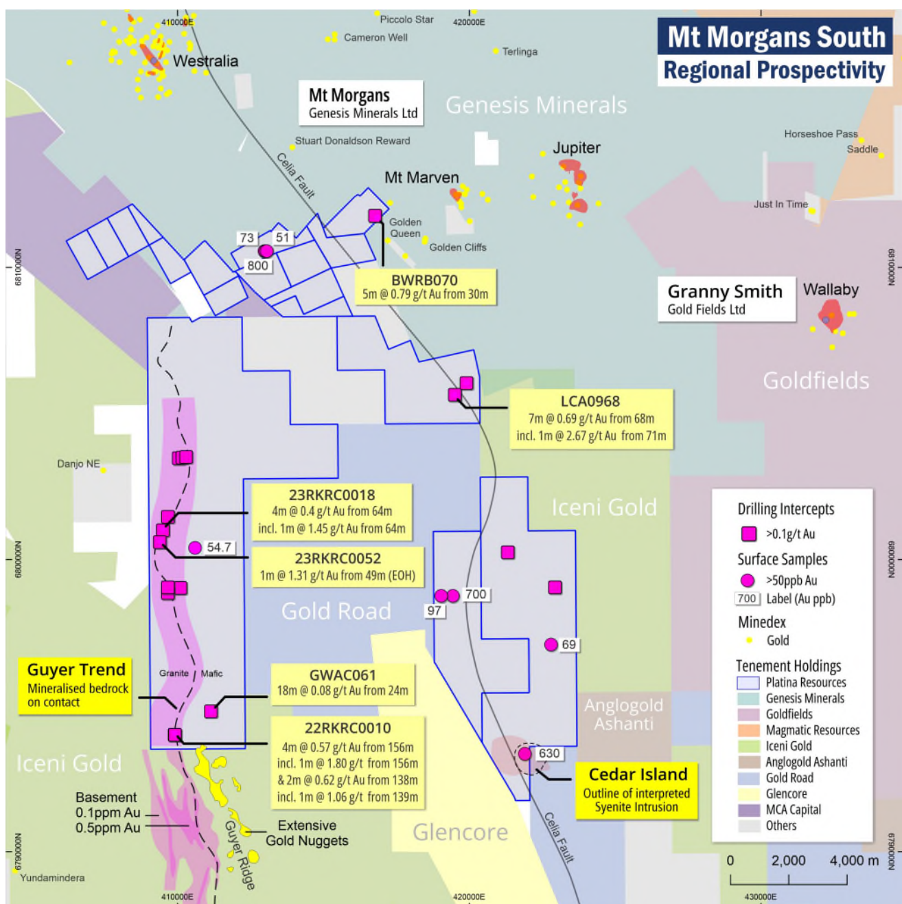
Figure 5. Mt Morgans South Project showing mineralised trends interpreted from historical exploration, Platina's near-term exploration target areas and the tenement holdings of major gold producers in the district.
