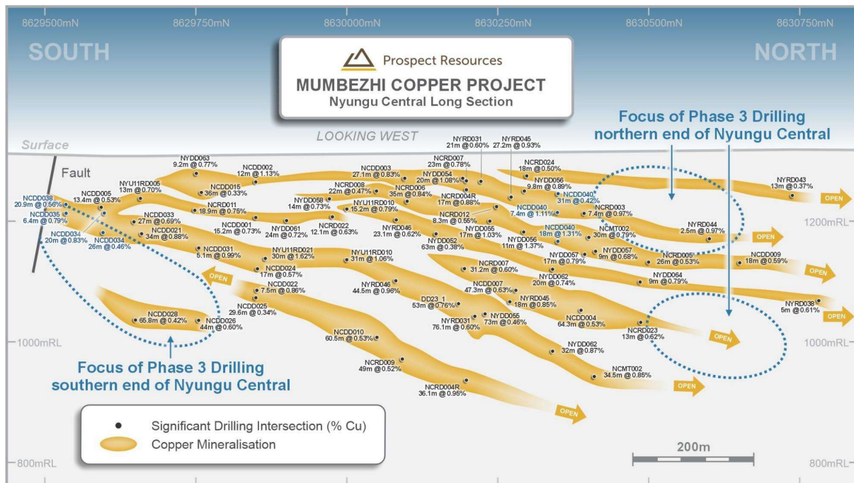
Figure 2: Nyungu Central long section (looking west) showing the locations of the new Phase 3 drill hole intercepts in blue.
