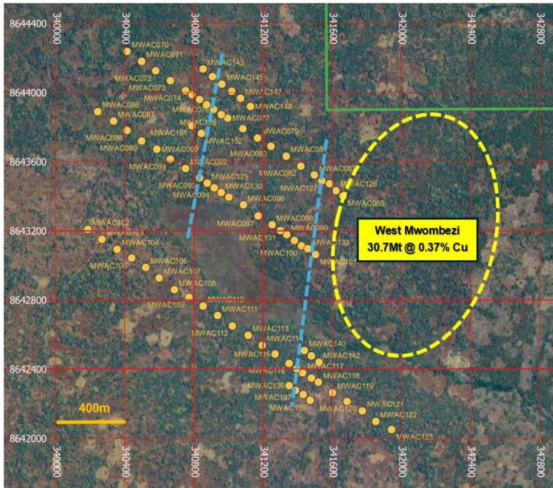
Figure 3: West Mwombezhi Phase 3 AC drilling has generated two new coherent copper anomalies (dashed blue lines) directly west of the defined Inferred Mineral Resource
