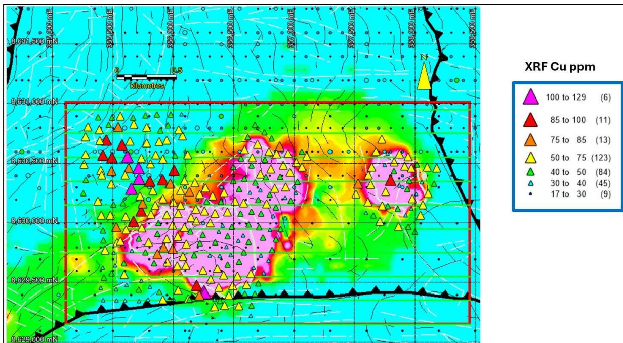
Figure 4: Chipimpa termite hill copper geochemistry over the three large conductive AEM anomalies, showing pXRF assays in ppm Cu
