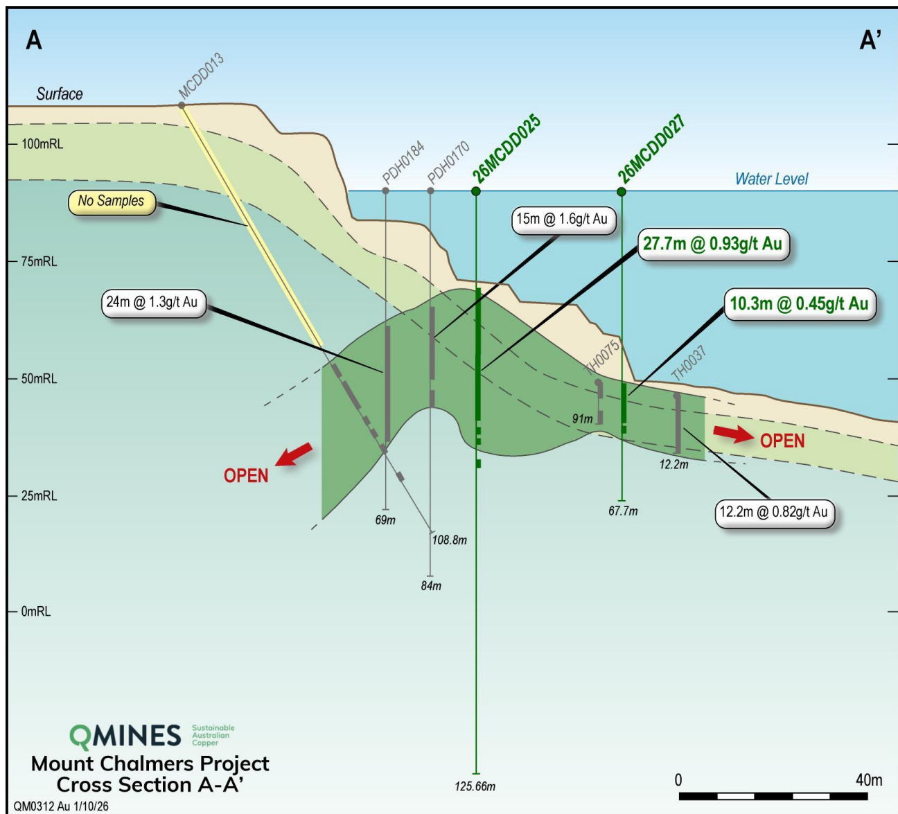
Figure 4 – A-A'; cross-section on a 12.5m window thickness illustrating the gold-dominant mineralised envelope.
