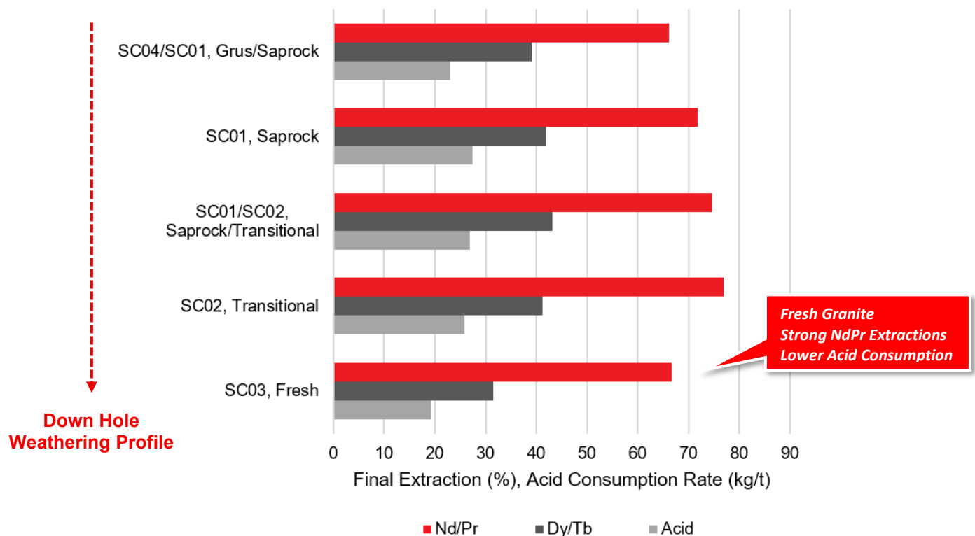
Figure 2 Sybella Kary Zone CLT by Lithology: Comparison of terminal acid consumption and NdPr extraction percentage calculated on a discharged mass basis for the -10mm crushed core from samples collected down the regolith profile from surface Grus to Fresh Granite at depth and some blends (Nd = neodymium, Pr = praseodymium). Refer to recent Red Metal ASX announcement dated 26 October 2026.
